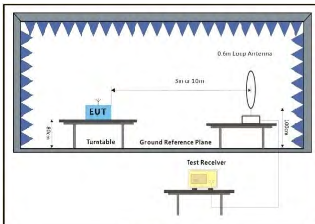
Below 30MHz
