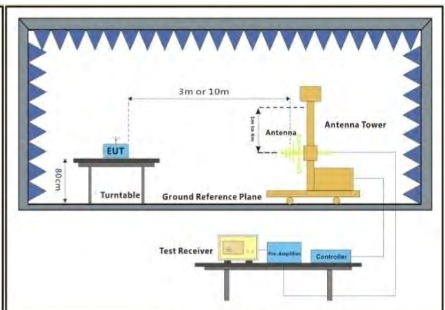
30MHz-1GHz
