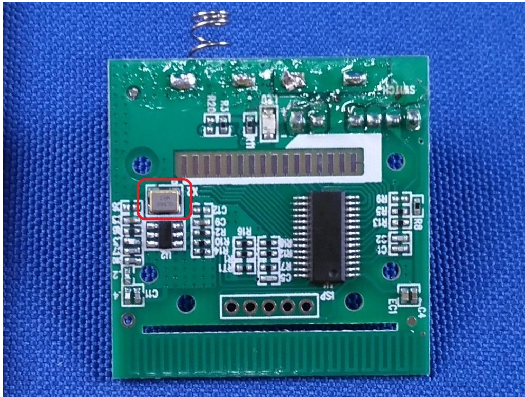
Oscillator
