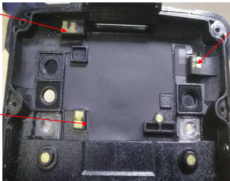
Main Antenna
