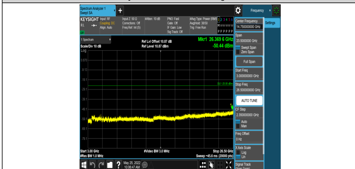
Band41-20MHz-QPSK-39750-1RB#0-Range5:3000~26500MHz
