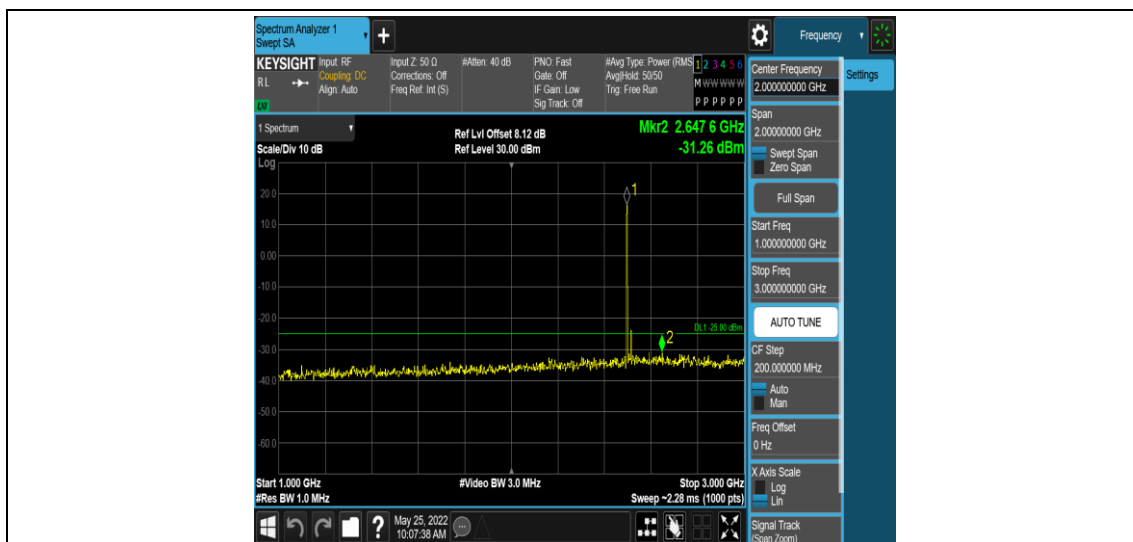
Band41-20MHz-16QAM-39750-1RB#0-Range4:1000~3000MHz
