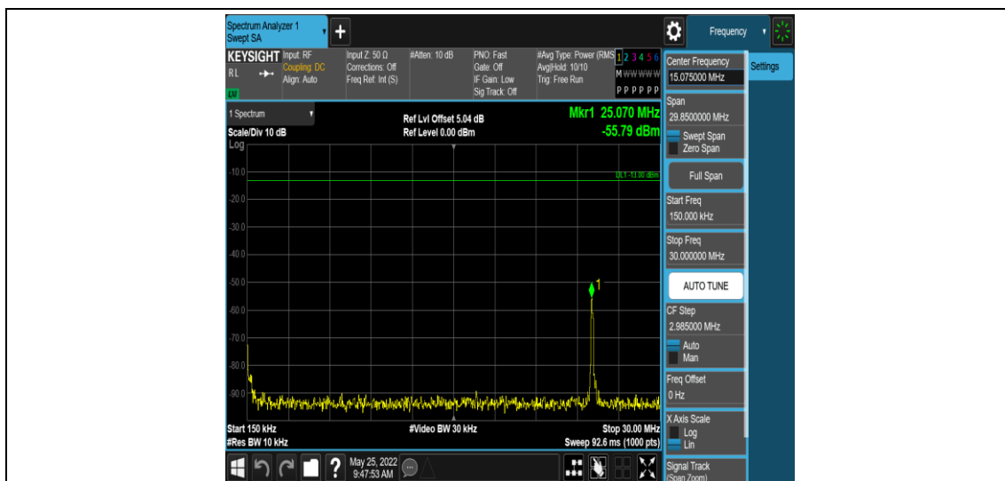
Band41-15MHz-16QAM-40620-1RB#0-Range2:0.15~30MHz
