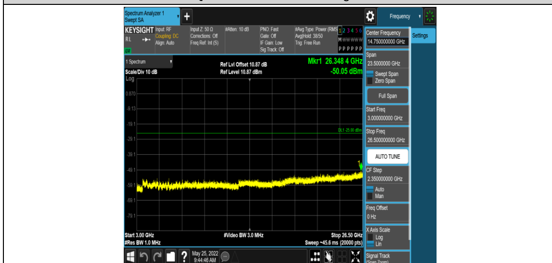
Band41-15MHz-QPSK-39725-1RB#0-Range5:3000~26500MHz
