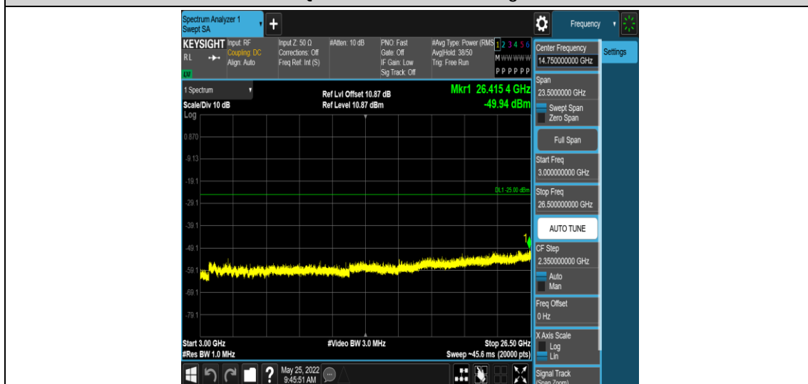
Band41-15MHz-16QAM-39725-1RB#0-Range5:3000~26500MHz
