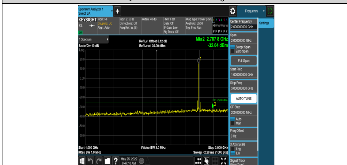
Band41-15MHz-QPSK-40620-1RB#0-Range4:1000~3000MHz
