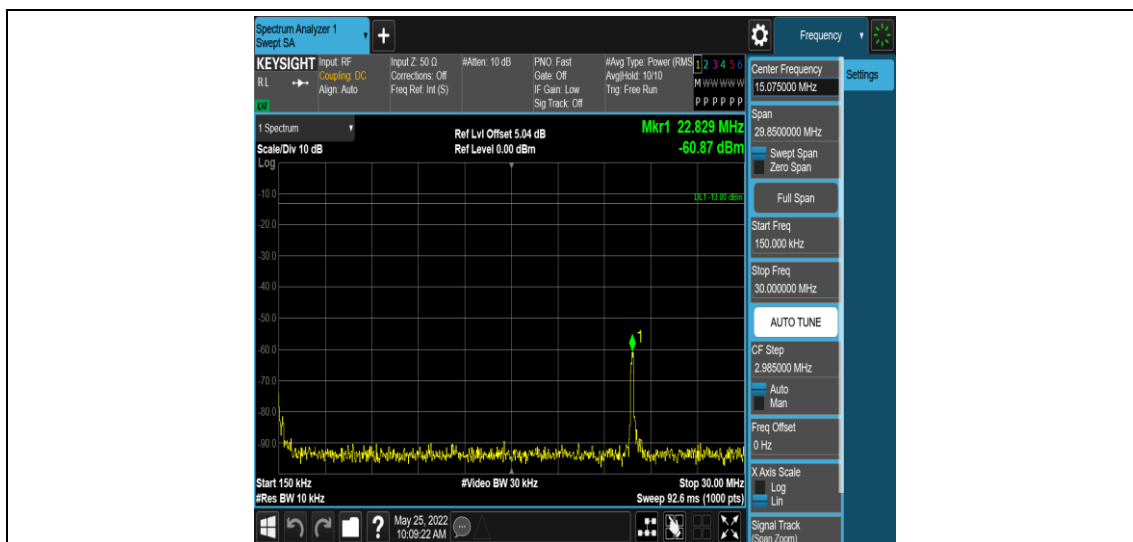
Band41-20MHz-16QAM-40620-1RB#0-Range2:0.15~30MHz
