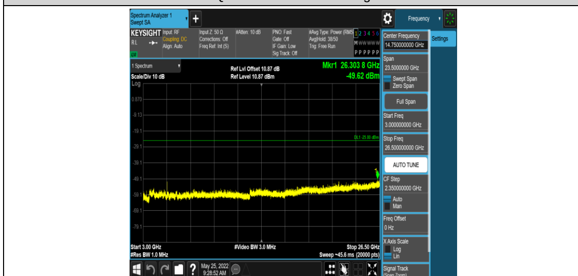
Band41-10MHz-16QAM-41540-1RB#0-Range5:3000~26500MHz
