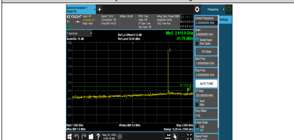
Band41-15MHz-16QAM-40620-1RB#0-Range4:1000~3000MHz
