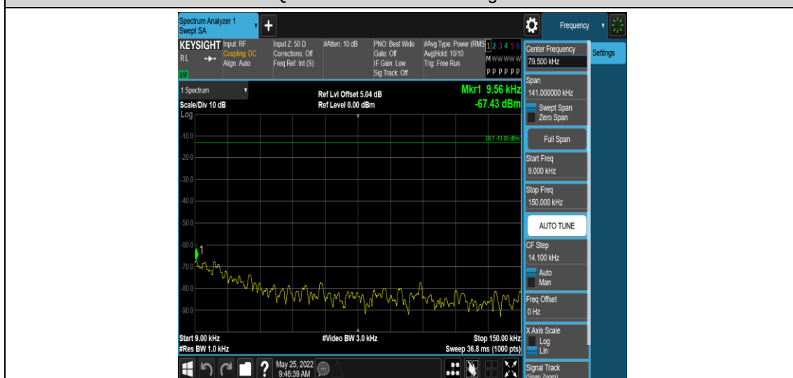
Band41-15MHz-QPSK-40620-1RB#0-Range1:0.009~0.15MHz
