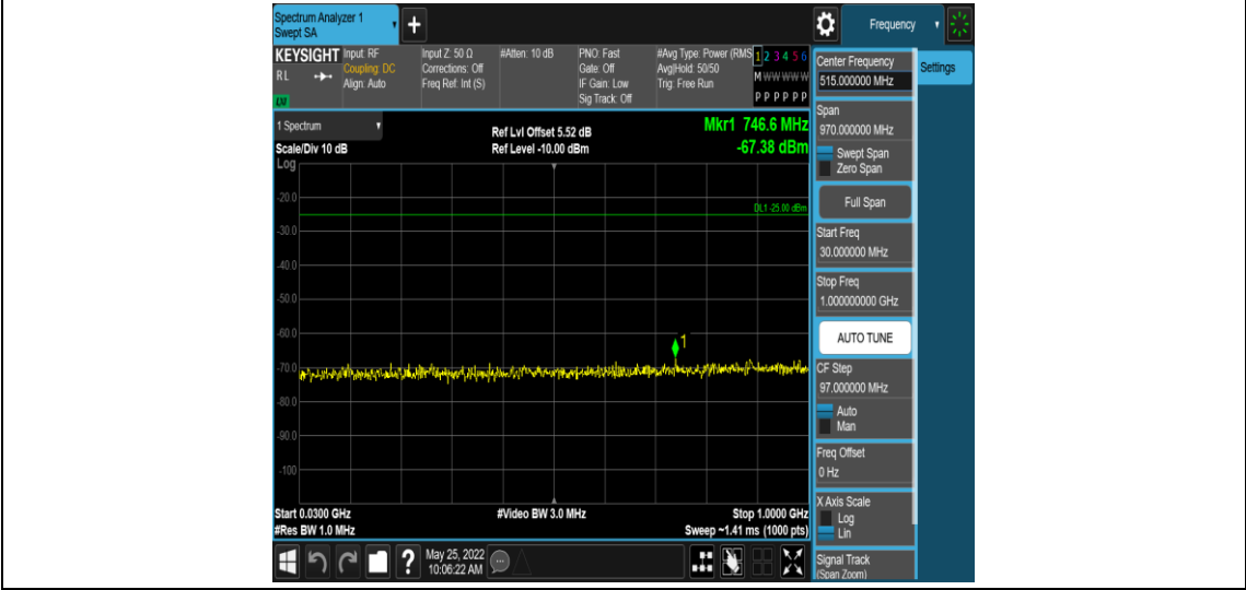
Band41-20MHz-QPSK-39750-1RB#0-Range3:30~1000MHz
