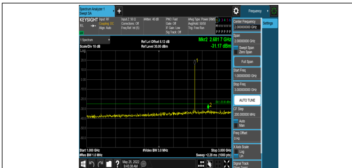
Band41-15MHz-16QAM-39725-1RB#0-Range4:1000~3000MHz
