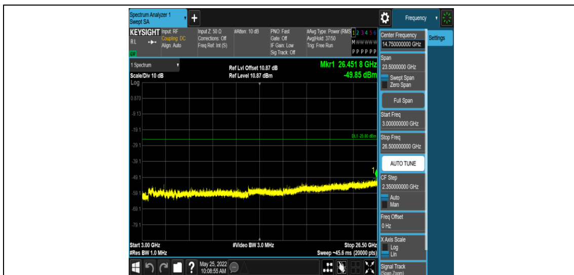
Band41-20MHz-QPSK-40620-1RB#0-Range5:3000~26500MHz
