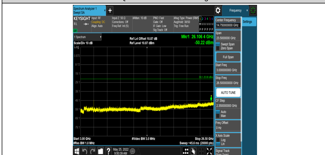
Band41-15MHz-16QAM-41515-1RB#0-Range5:3000~26500MHz
