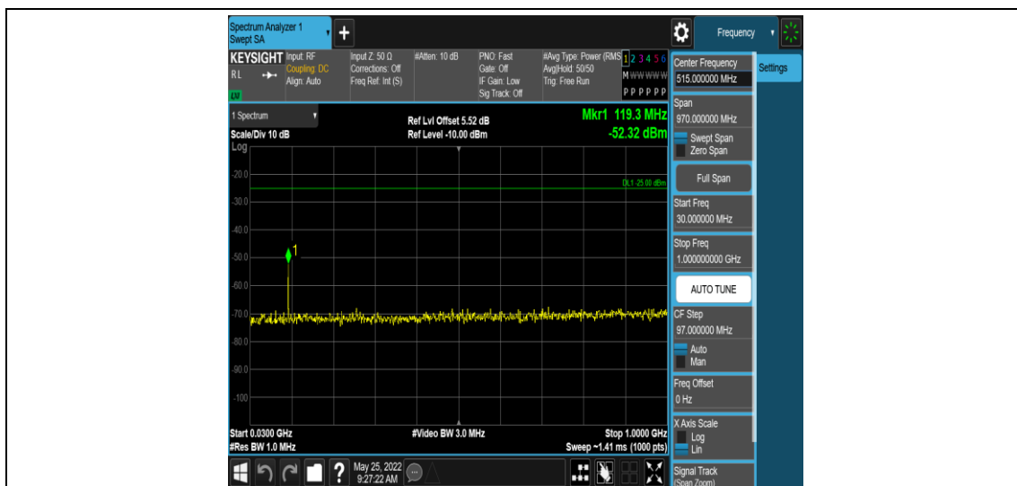
Band41-10MHz-QPSK-41540-1RB#0-Range3:30~1000MHz
