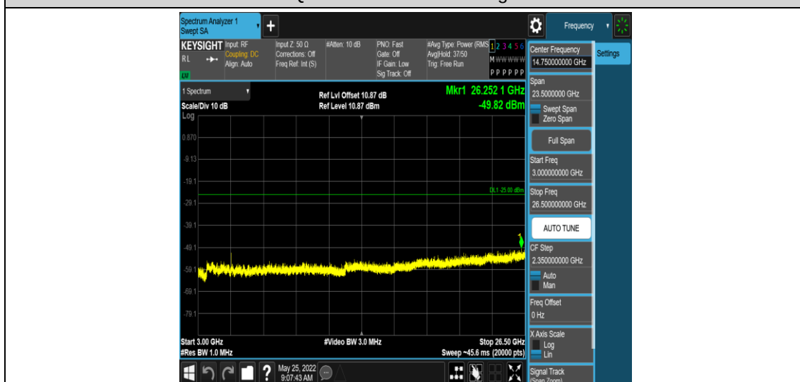
Band41-5MHz-16QAM-41565-1RB#0-Range5:3000~26500MHz
