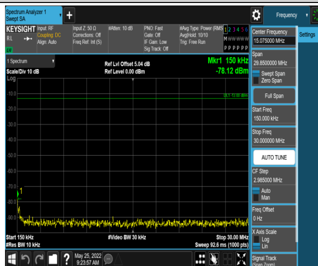
Band41-10MHz-16QAM-39700-1RB#0-Range2:0.15~30MHz
