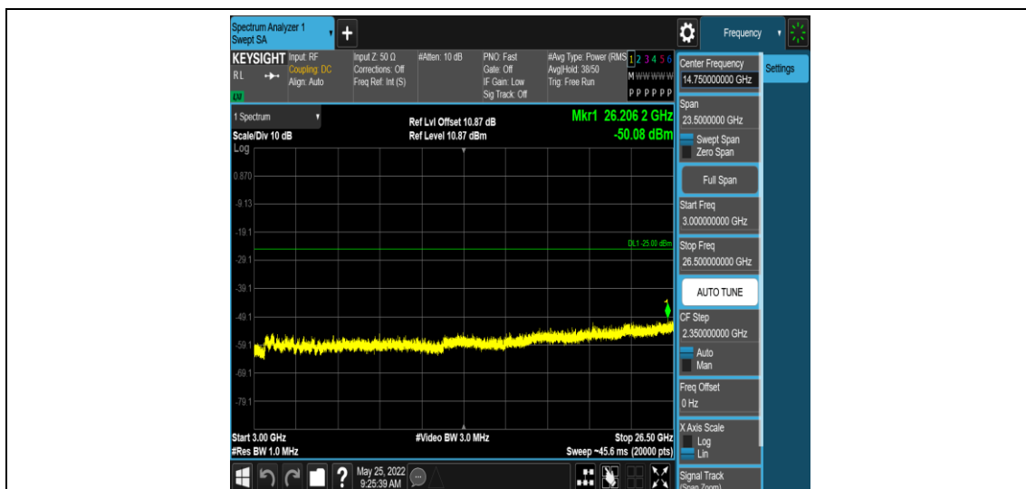
Band41-10MHz-QPSK-40620-1RB#0-Range5:3000~26500MHz
