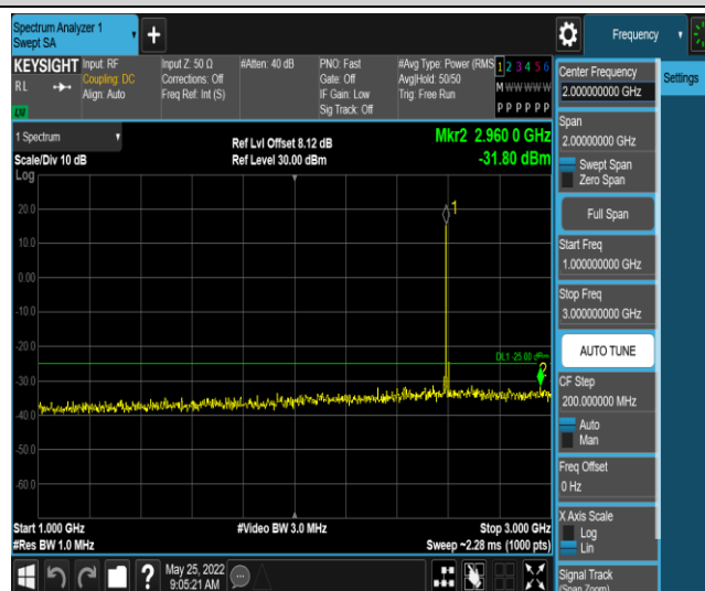
Band41-5MHz-16QAM-40620-1RB#0-Range4:1000~3000MHz
