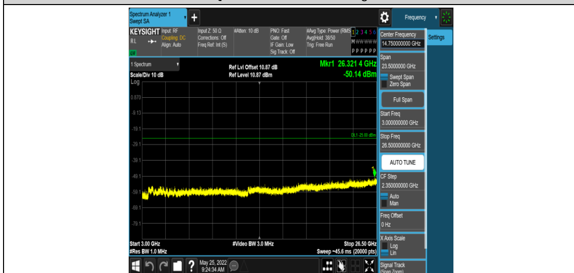
Band41-10MHz-16QAM-39700-1RB#0-Range5:3000~26500MHz
