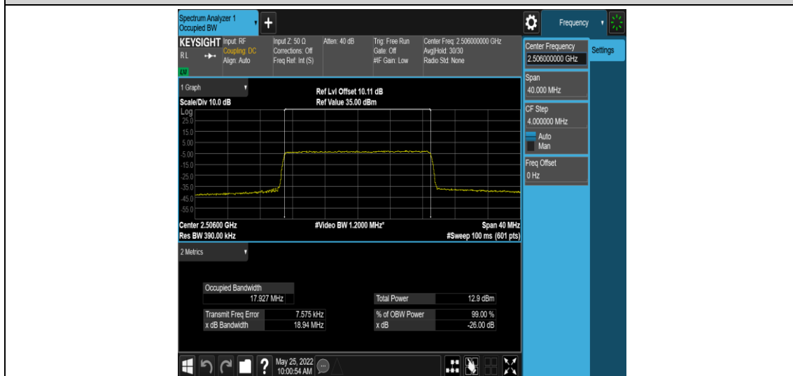
Band41-20MHz-16QAM-39750-100RB#0
