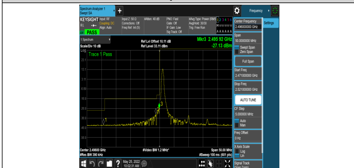
Band41-20MHz-16QAM-39750-1RB#0
