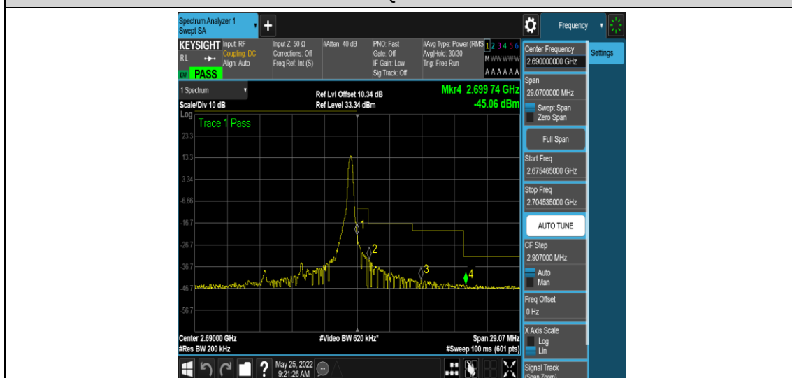
Band41-10MHz-QPSK-41540-1RB#49
