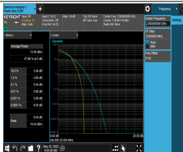
Band41-15MHz-16QAM-40620-1RB#0
