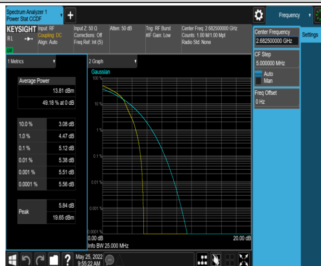
Band41-15MHz-16QAM-41515-1RB#0
