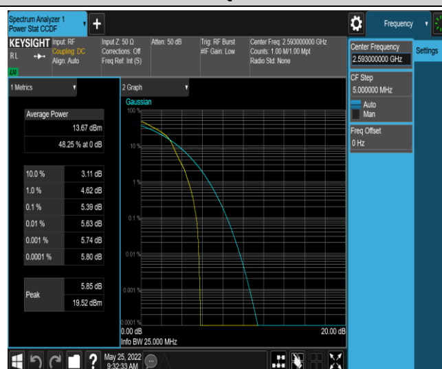
Band41-10MHz-16QAM-40620-1RB#0
