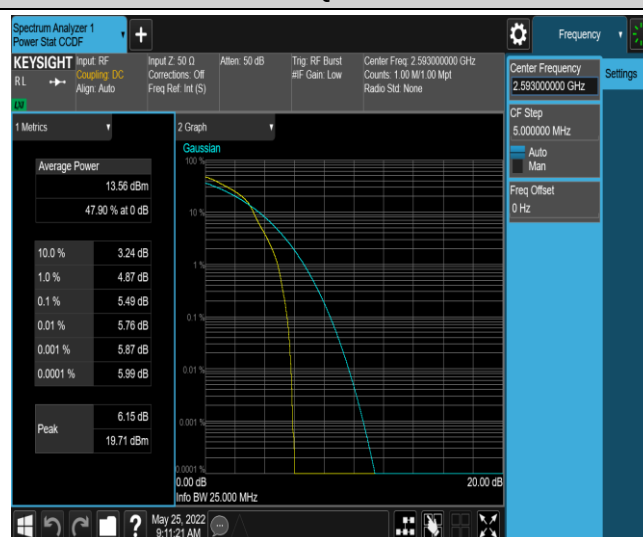
Band41-5MHz-16QAM-40620-1RB#0
