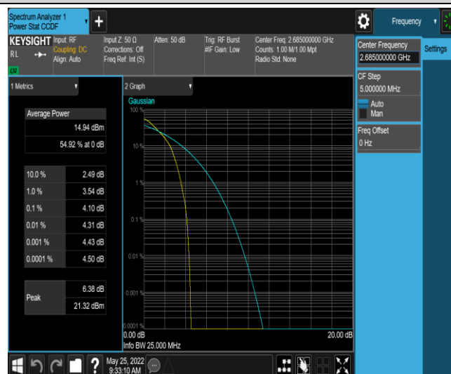
Band41-10MHz-QPSK-41540-1RB#0
