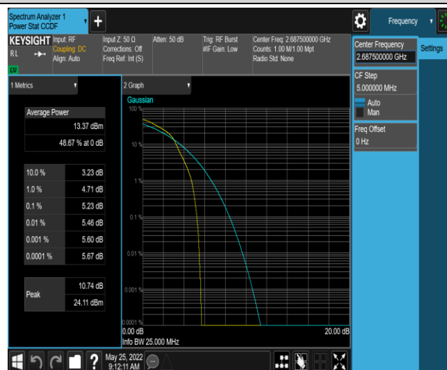
Band41-5MHz-16QAM-41565-1RB#0
