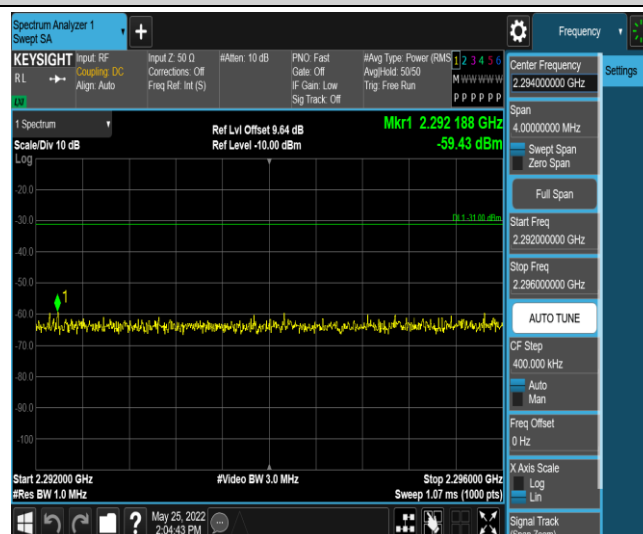
Band40-5MHz-16QAM-39175-1RB#0-Range6:2292~2296MHz
