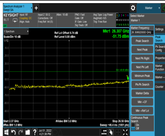
Band40-5MHz-16QAM-39175-1RB#0-Range15:2365~26500MHz
