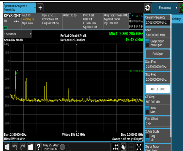
Band40-5MHz-16QAM-39175-1RB#0-Range14:2360~2365MHz
