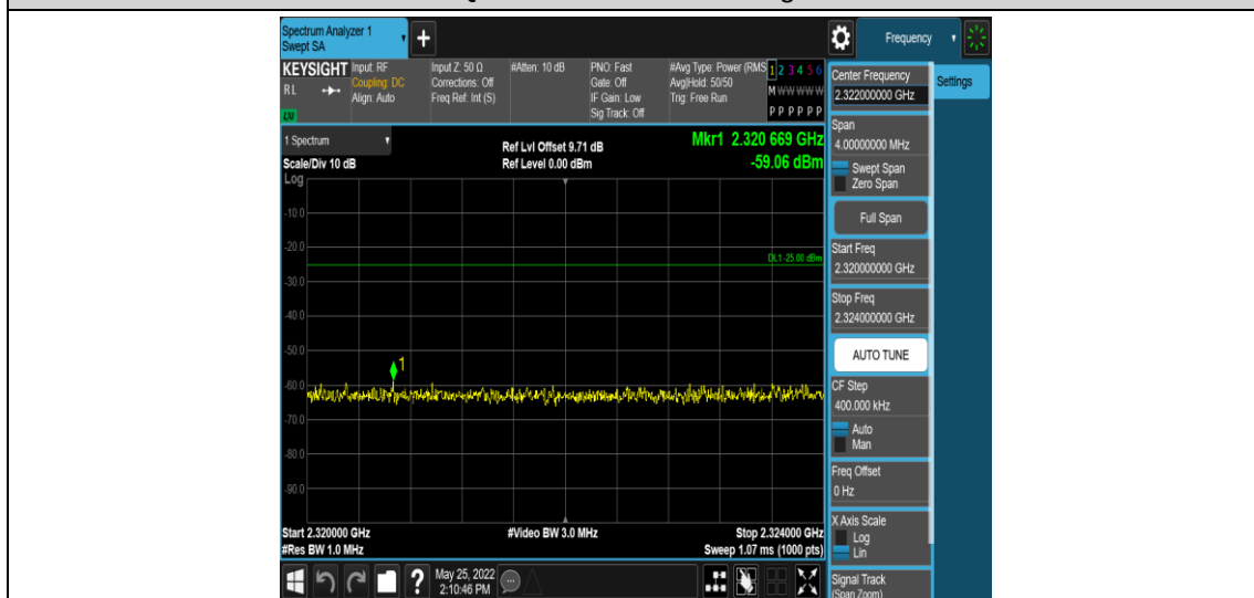
Band40-5MHz-16QAM-39200-1RB#0-Range9:2320~2324MHz
