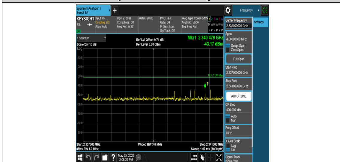
Band40-5MHz-QPSK-39200-1RB#0-Range12:2337~2341MHz
