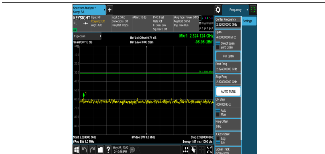
Band40-5MHz-16QAM-39200-1RB#0-Range10:2324~2328MHz
