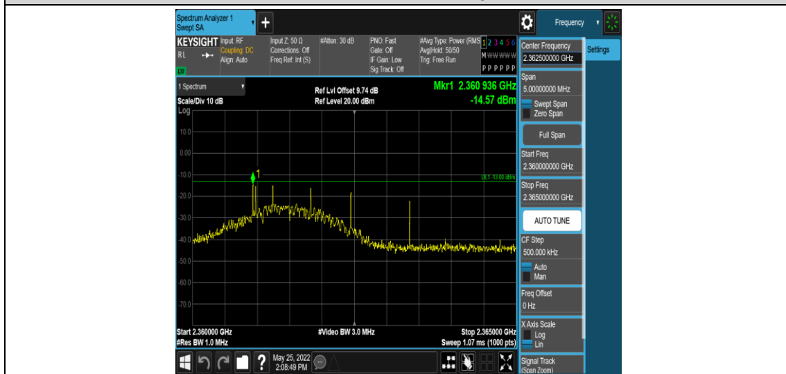
Band40-5MHz-QPSK-39200-1RB#0-Range14:2360~2365MHz
