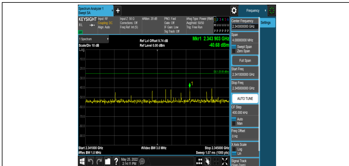
Band40-5MHz-QPSK-39225-1RB#0-Range13:2341~2345MHz
