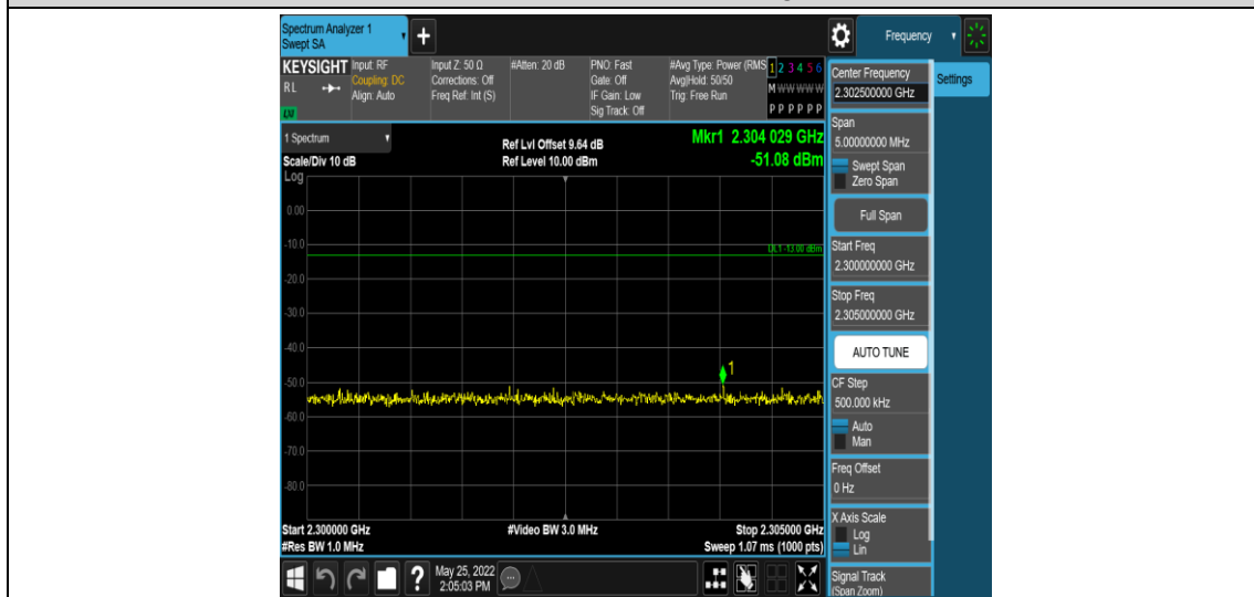
Band40-5MHz-16QAM-39175-1RB#0-Range8:2300~2305MHz
