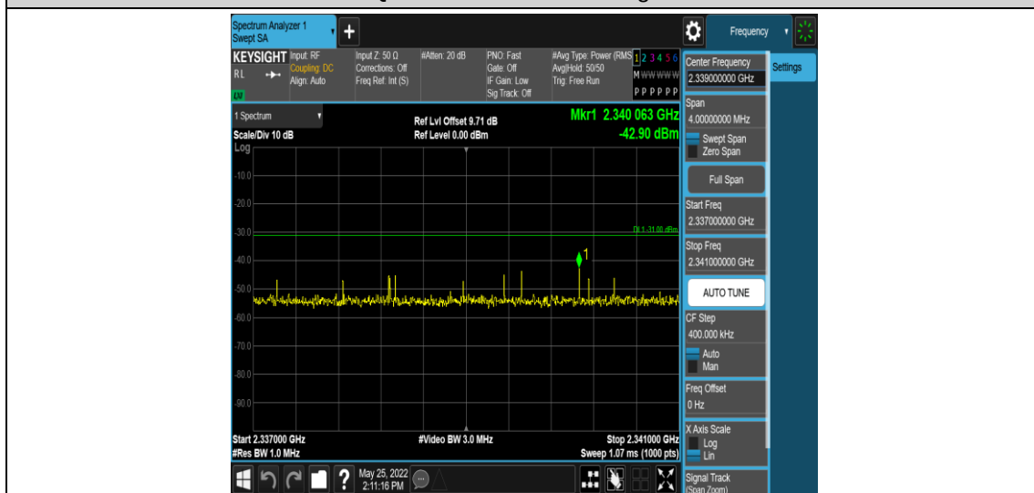
Band40-5MHz-16QAM-39200-1RB#0-Range12:2337~2341MHz
