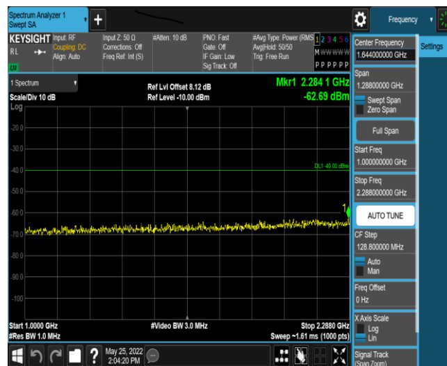
Band40-5MHz-16QAM-39175-1RB#0-Range4:1000~2288MHz
