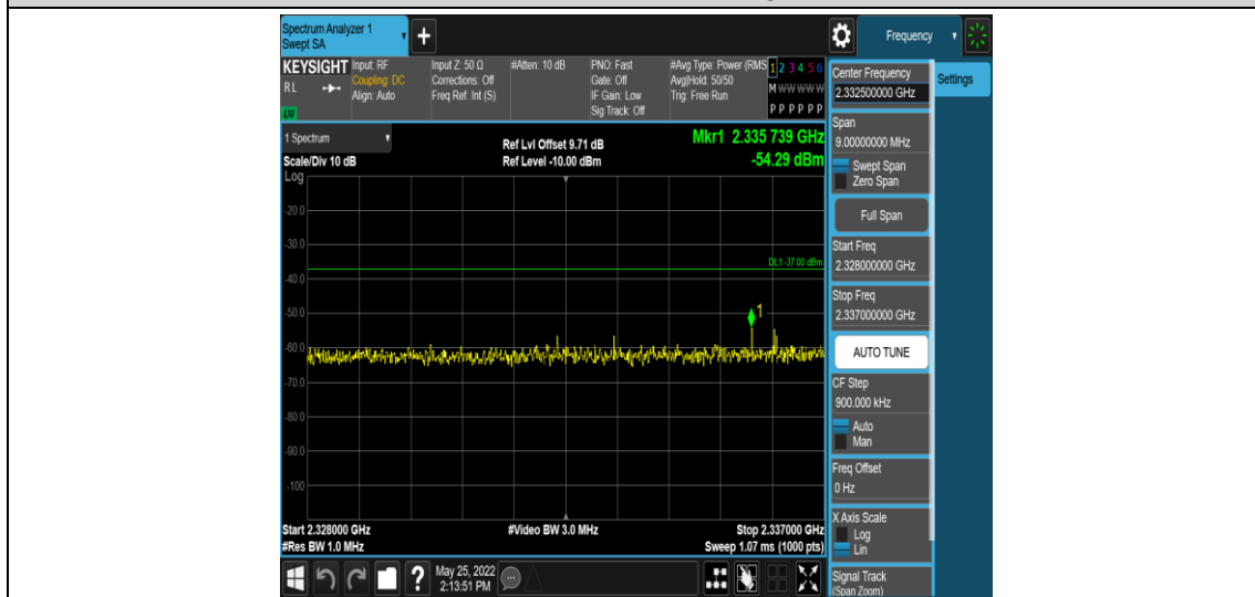
Band40-5MHz-QPSK-39225-1RB#0-Range11:2328~2337MHz
