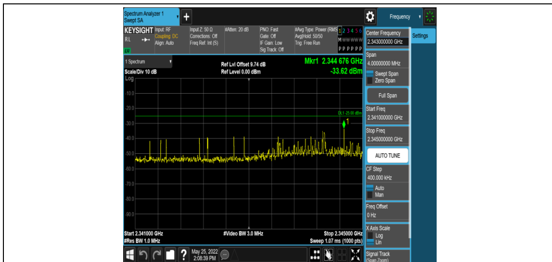
Band40-5MHz-QPSK-39200-1RB#0-Range13:2341~2345MHz
