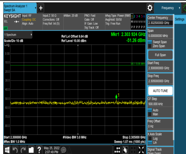
Band40-5MHz-QPSK-39200-1RB#0-Range8:2300~2305MHz
