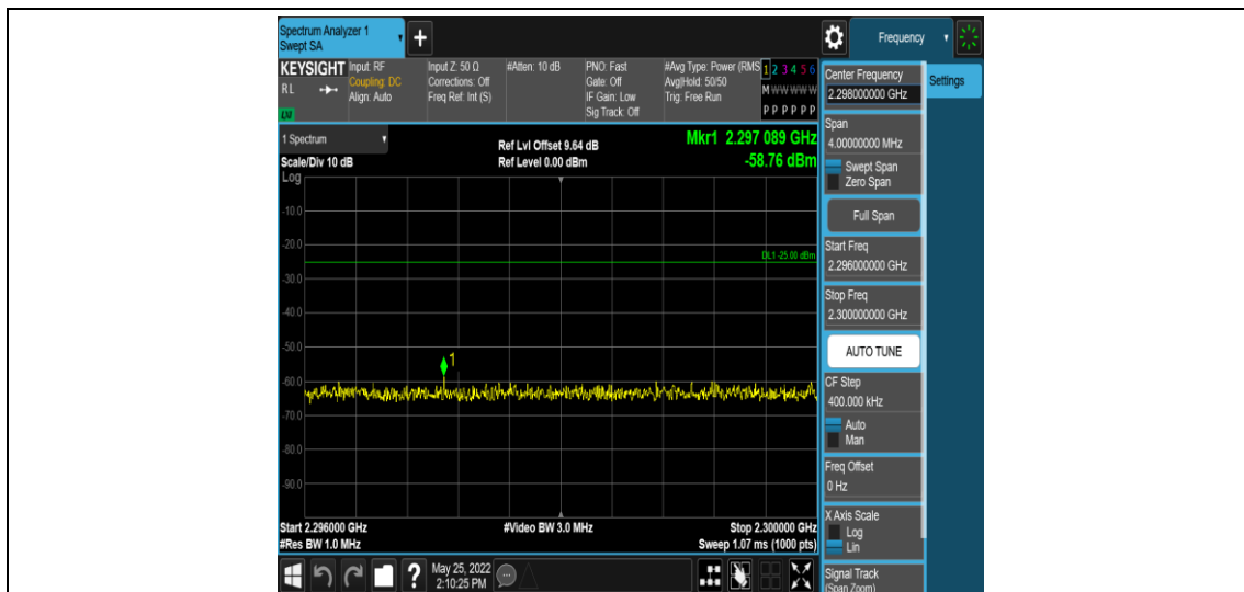
Band40-5MHz-16QAM-39200-1RB#0-Range7:2296~2300MHz
