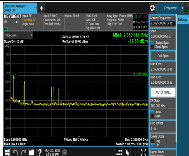
Band40-5MHz-QPSK-39175-1RB#0-Range14:2360~2365MHz
