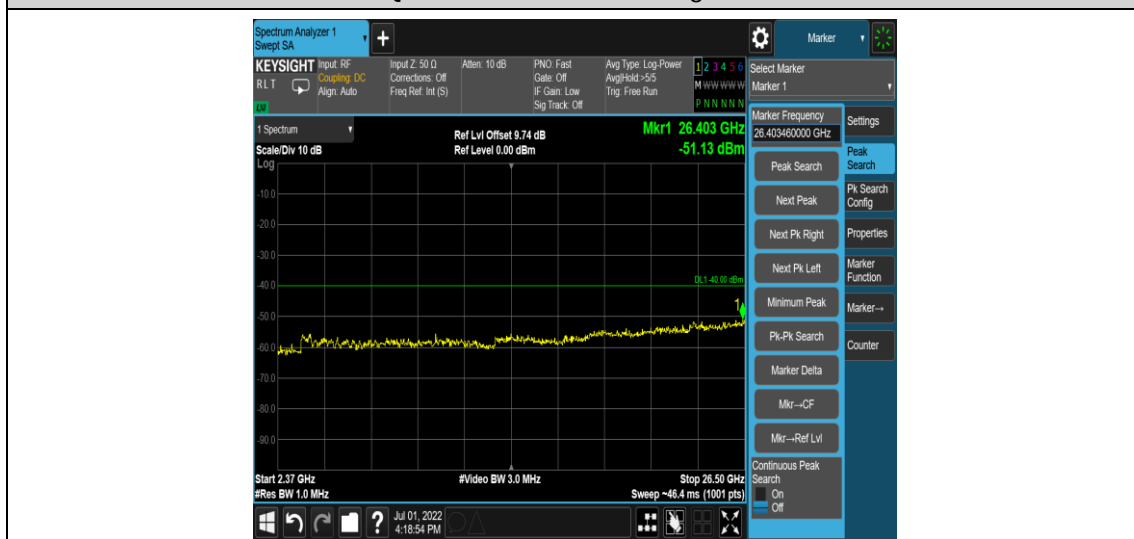
Band40-5MHz-QPSK-39200-1RB#0-Range15:2365~26500MHz
