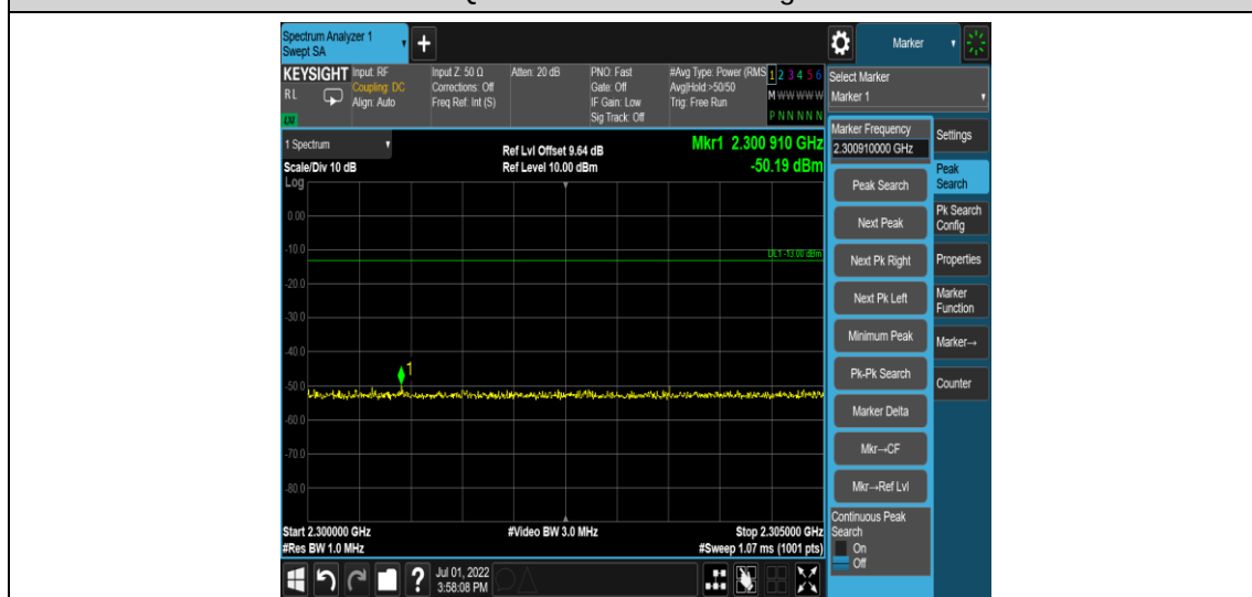
Band40-5MHz-16QAM-38750-1RB#0-Range8:2300~2305MHz
