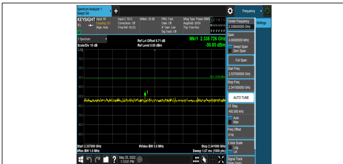
Band40-5MHz-QPSK-38775-1RB#0-Range12:2337~2341MHz
