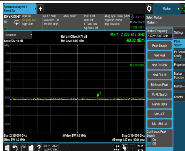
Band40-5MHz-QPSK-38775-1RB#0-Range9:2320~2324MHz
