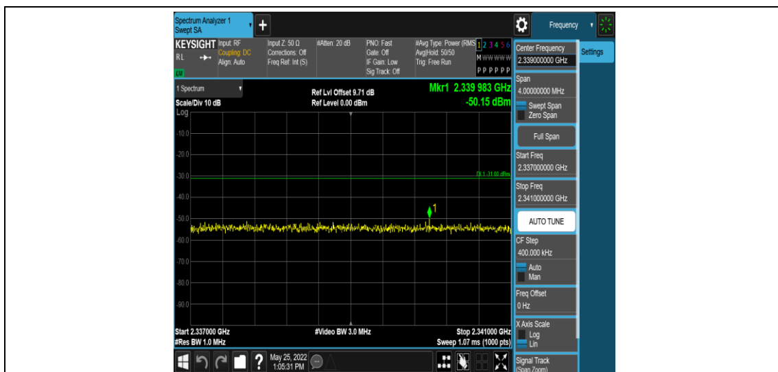
Band40-5MHz-16QAM-38725-1RB#0-Range12:2337~2341MHz
