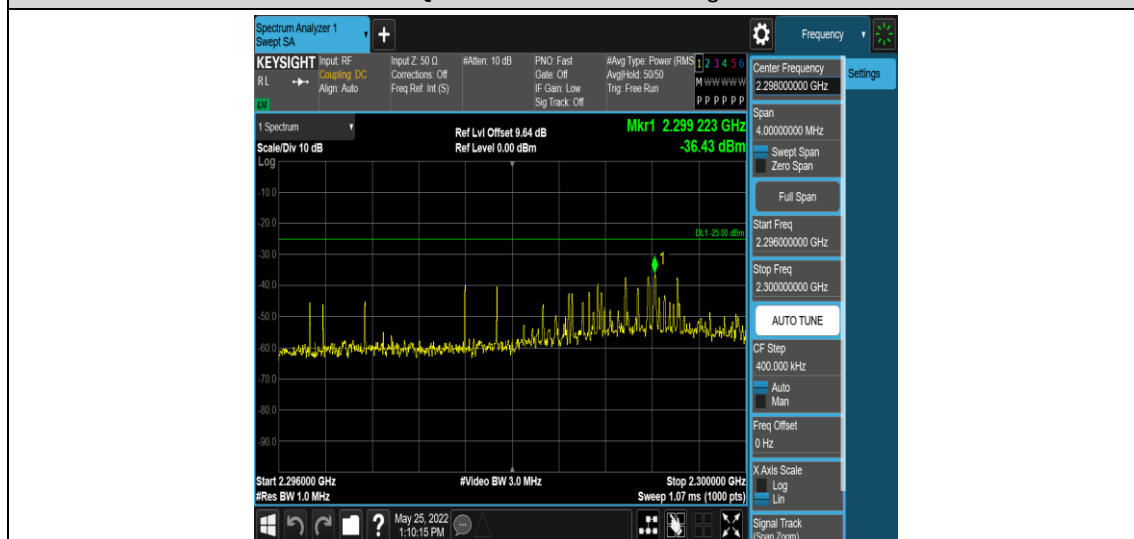
Band40-5MHz-16QAM-38750-1RB#0-Range7:2296~2300MHz
