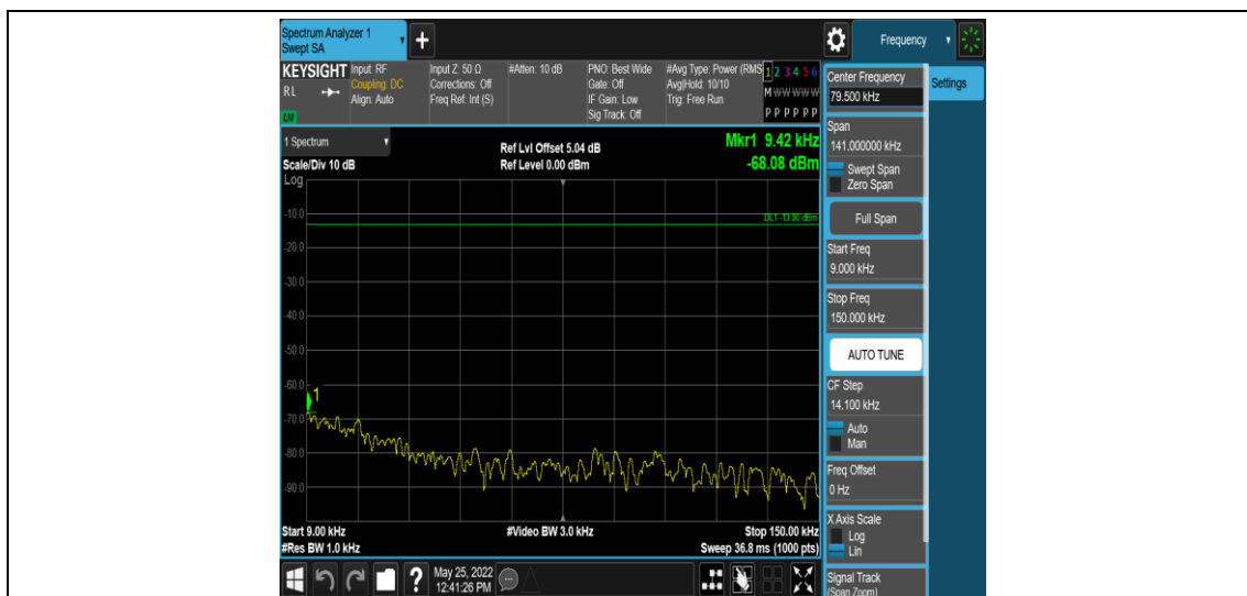
Band38-20MHz-QPSK-38000-1RB#0-Range1:0.009~0.15MHz
