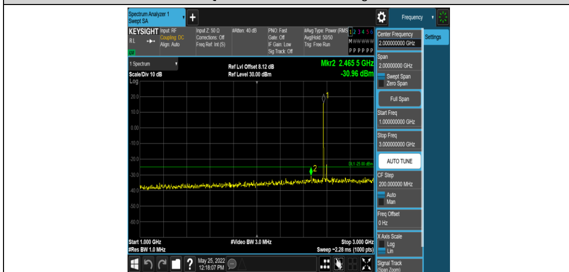
Band38-15MHz-QPSK-37825-1RB#0-Range4:1000~3000MHz
