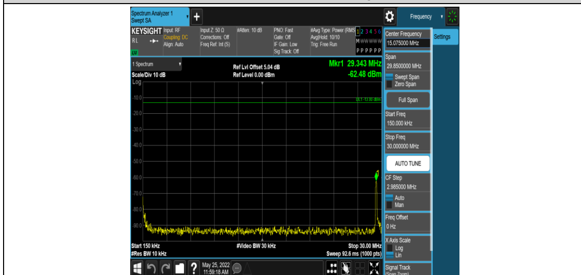
Band38-10MHz-16QAM-38000-1RB#0-Range2:0.15~30MHz
