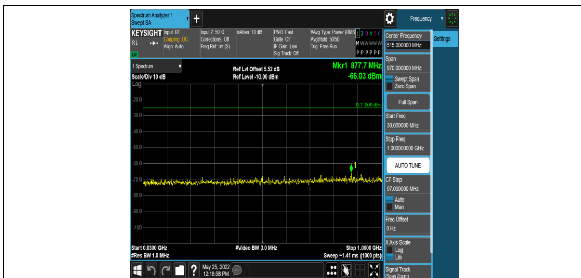
Band38-15MHz-16QAM-37825-1RB#0-Range3:30~1000MHz
