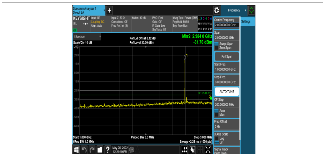
Band38-15MHz-16QAM-38000-1RB#0-Range4:1000~3000MHz
