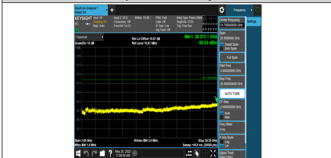
Band38-10MHz-16QAM-38000-1RB#0-Range5:3000~26500MHz
