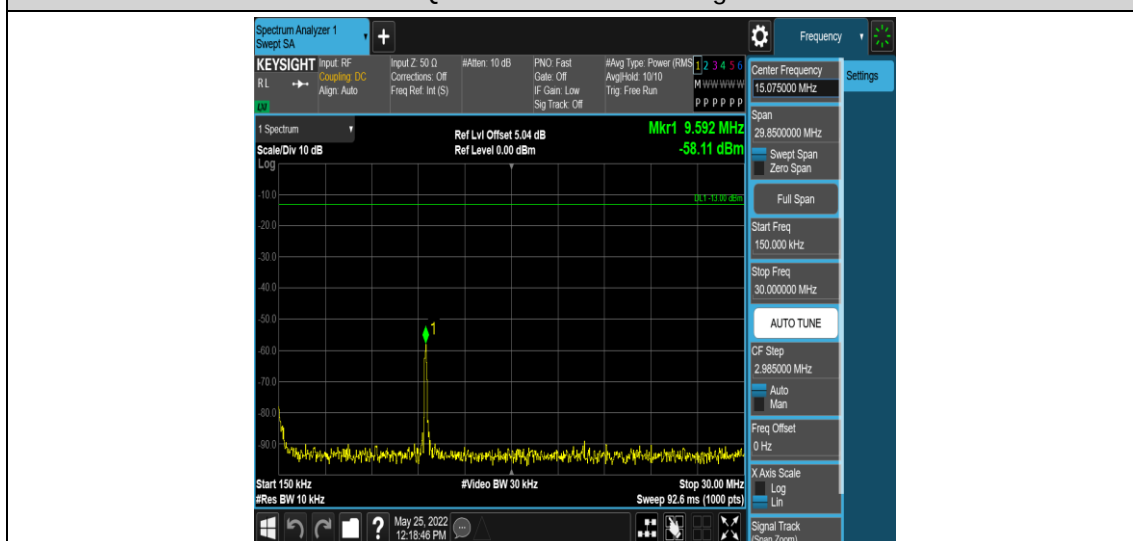
Band38-15MHz-16QAM-37825-1RB#0-Range2:0.15~30MHz
