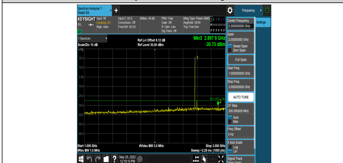
Band38-15MHz-16QAM-37825-1RB#0-Range4:1000~3000MHz
