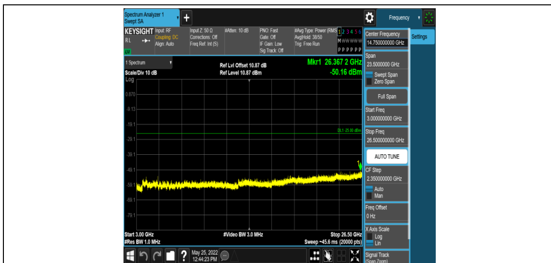
Band38-20MHz-QPSK-38150-1RB#0-Range5:3000~26500MHz
