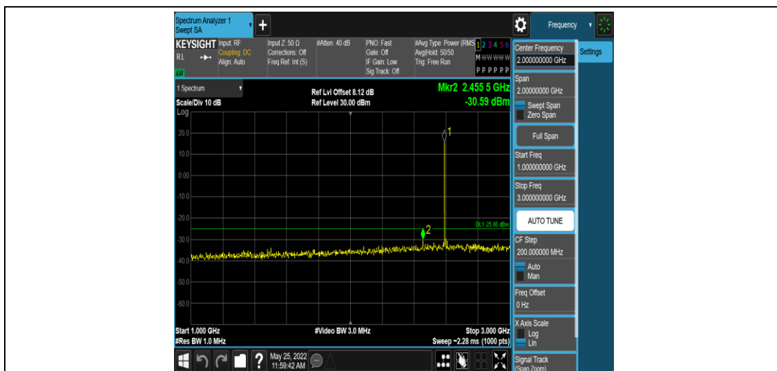
Band38-10MHz-16QAM-38000-1RB#0-Range4:1000~3000MHz
