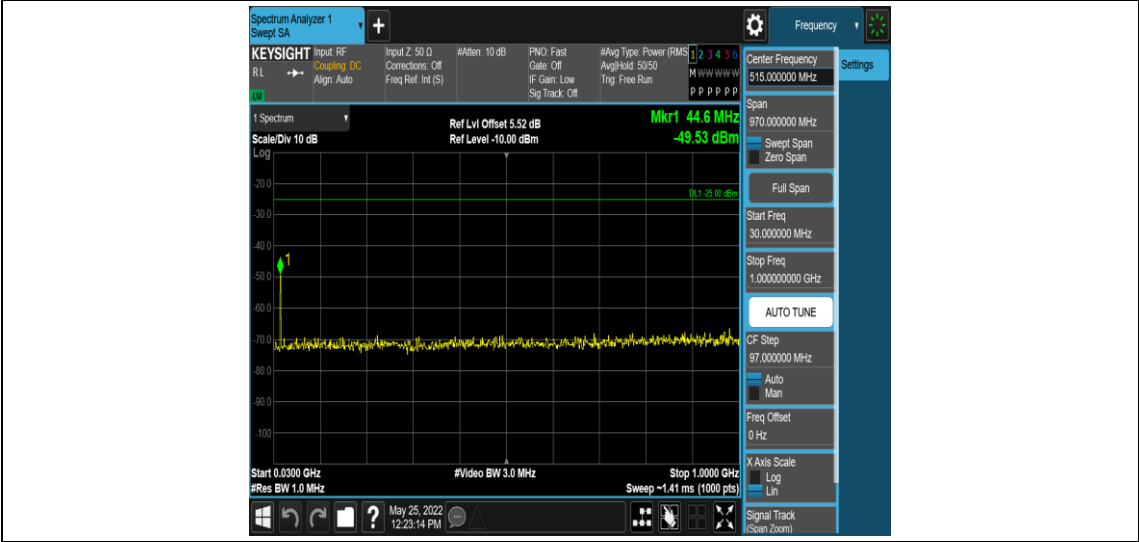
Band38-15MHz-16QAM-38175-1RB#0-Range3:30~1000MHz
