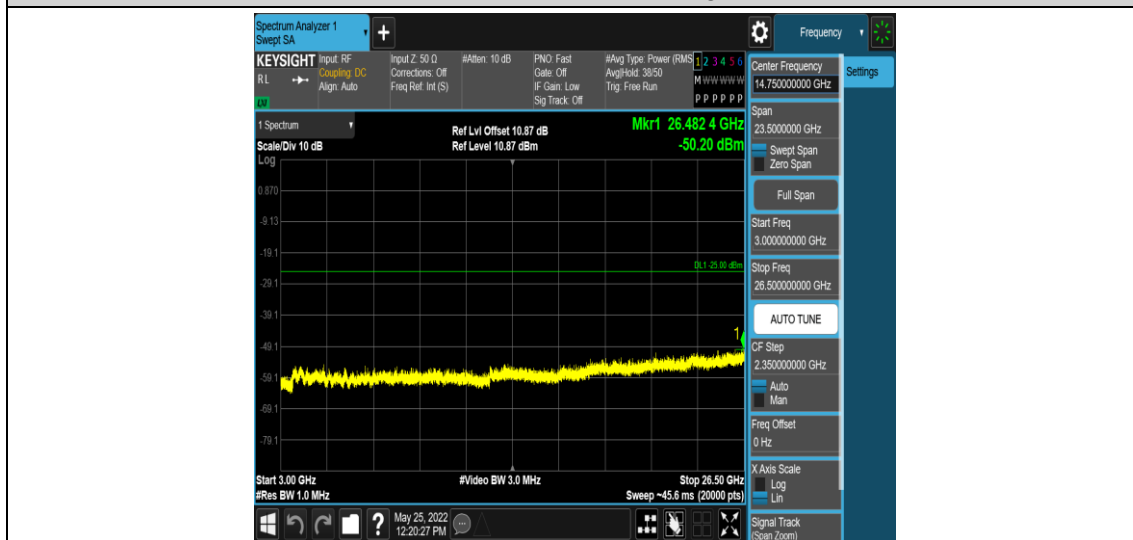
Band38-15MHz-QPSK-38000-1RB#0-Range5:3000~26500MHz
