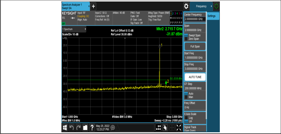
Band38-15MHz-16QAM-38175-1RB#0-Range4:1000~3000MHz
