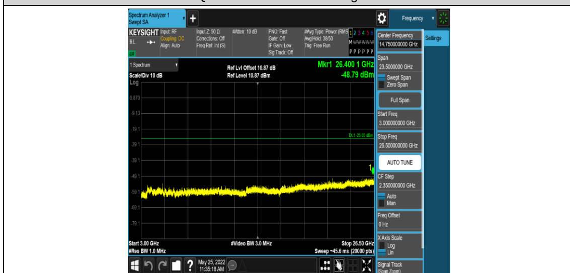
Band38-5MHz-QPSK-37775-1RB#0-Range5:3000~26500MHz
