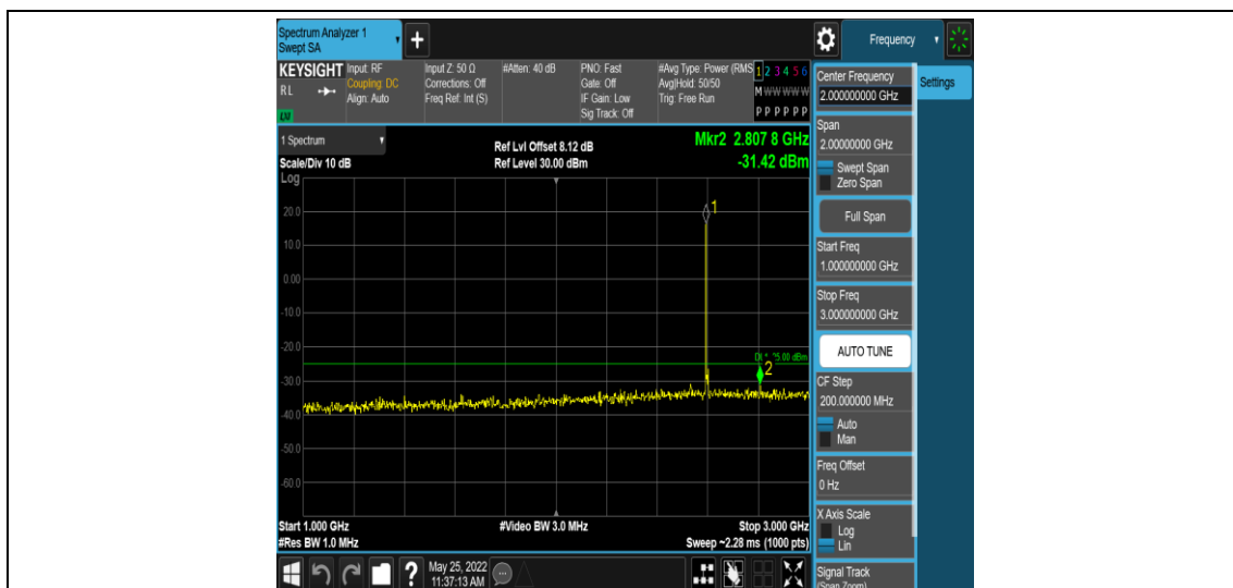
Band38-5MHz-QPSK-38000-1RB#0-Range4:1000~3000MHz
