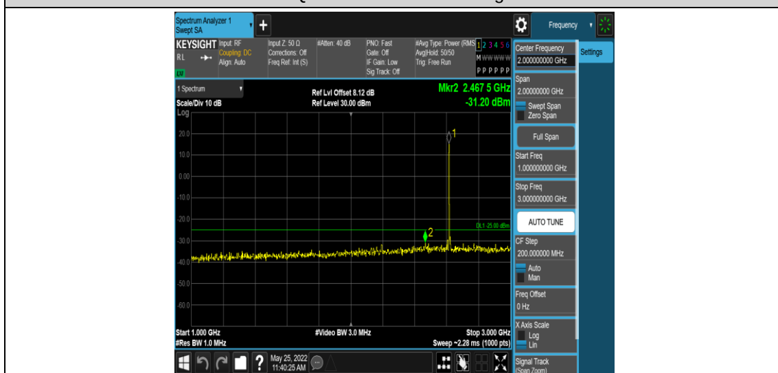
Band38-5MHz-16QAM-38225-1RB#0-Range4:1000~3000MHz
