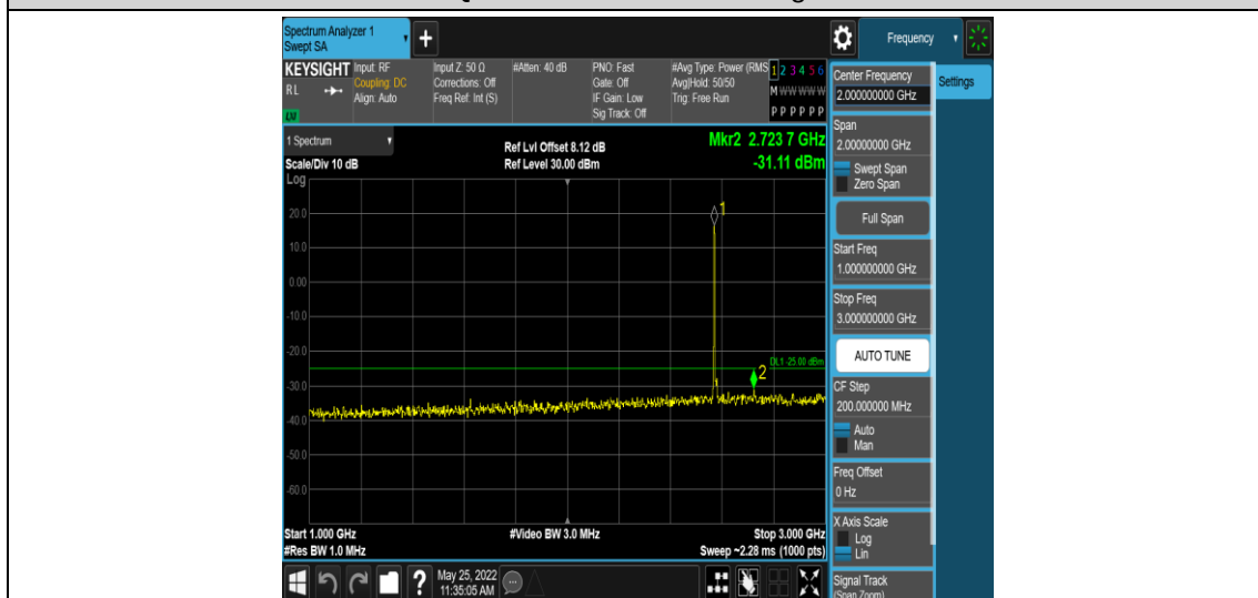
Band38-5MHz-QPSK-37775-1RB#0-Range4:1000~3000MHz
