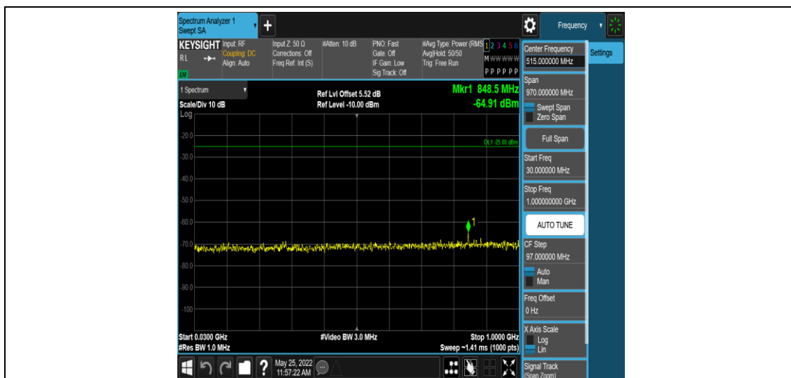
Band38-10MHz-16QAM-37800-1RB#0-Range3:30~1000MHz
