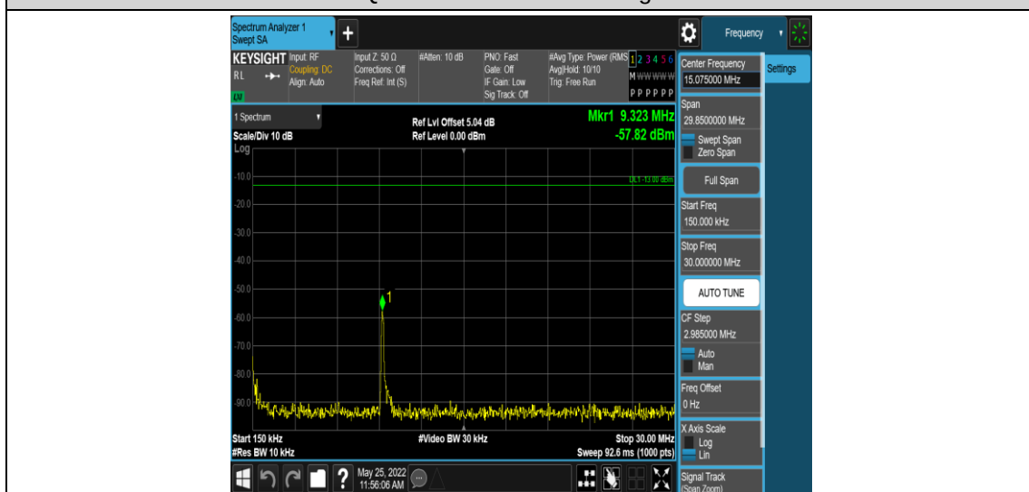
Band38-10MHz-QPSK-37800-1RB#0-Range2:0.15~30MHz
