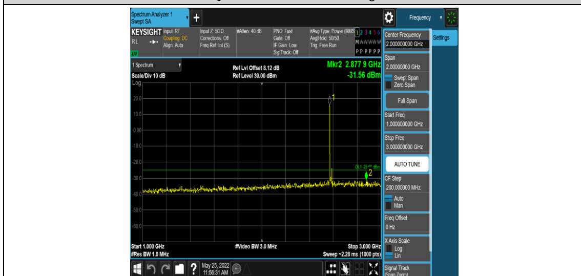
Band38-10MHz-QPSK-37800-1RB#0-Range4:1000~3000MHz
