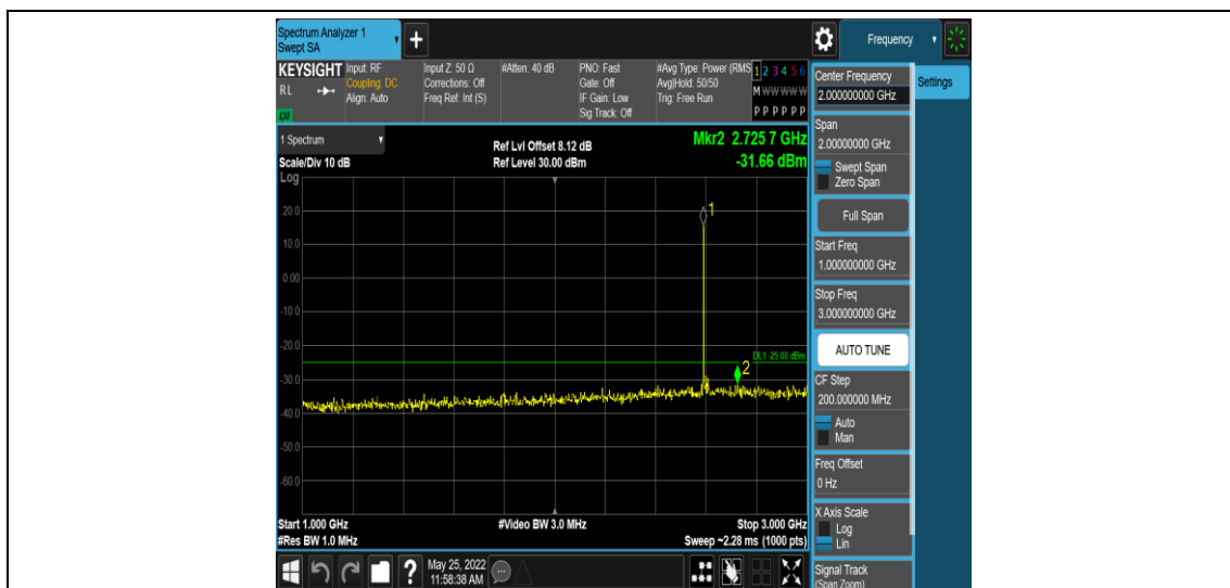
Band38-10MHz-QPSK-38000-1RB#0-Range4:1000~3000MHz
