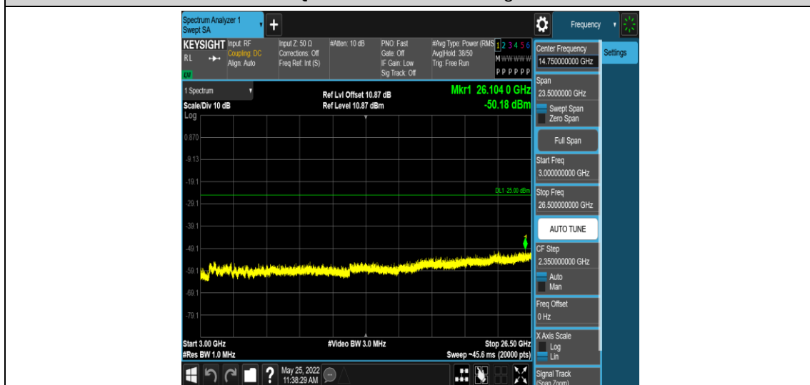
Band38-5MHz-16QAM-38000-1RB#0-Range5:3000~26500MHz
