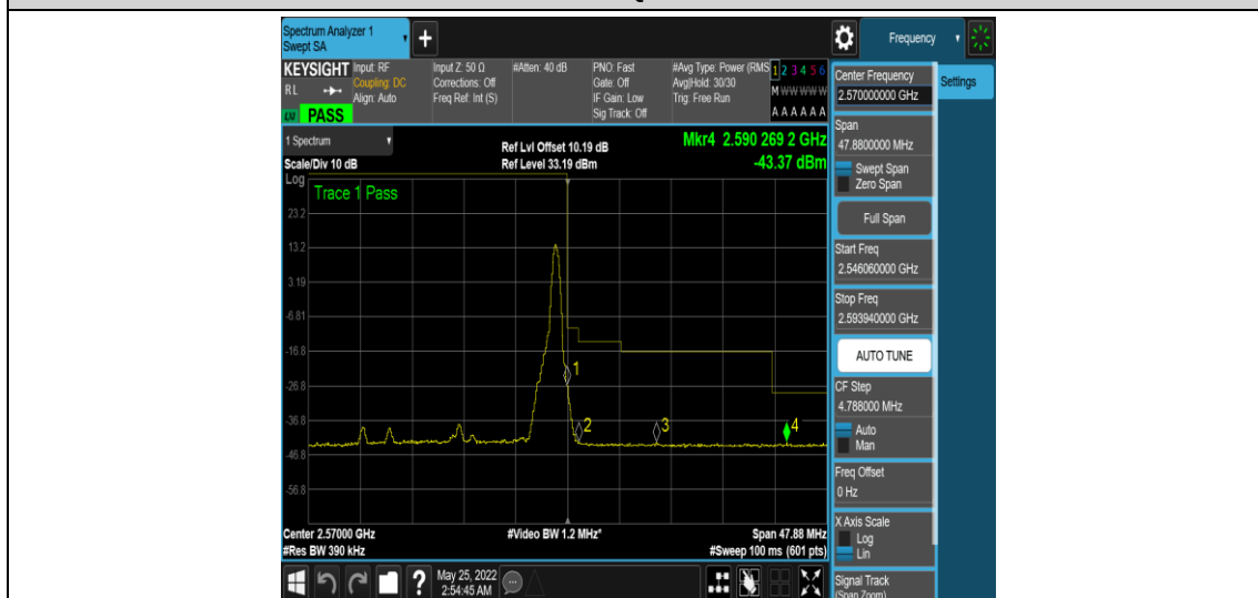
Band7-20MHz-16QAM-21350-1RB#99
