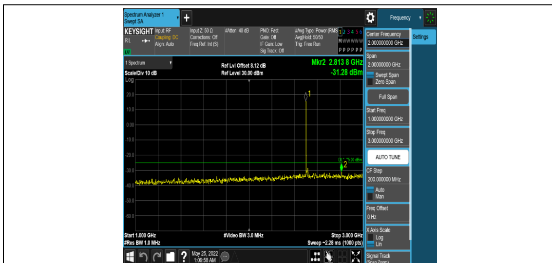
Band7-10MHz-16QAM-20800-1RB#0-Range4:1000~3000MHz
