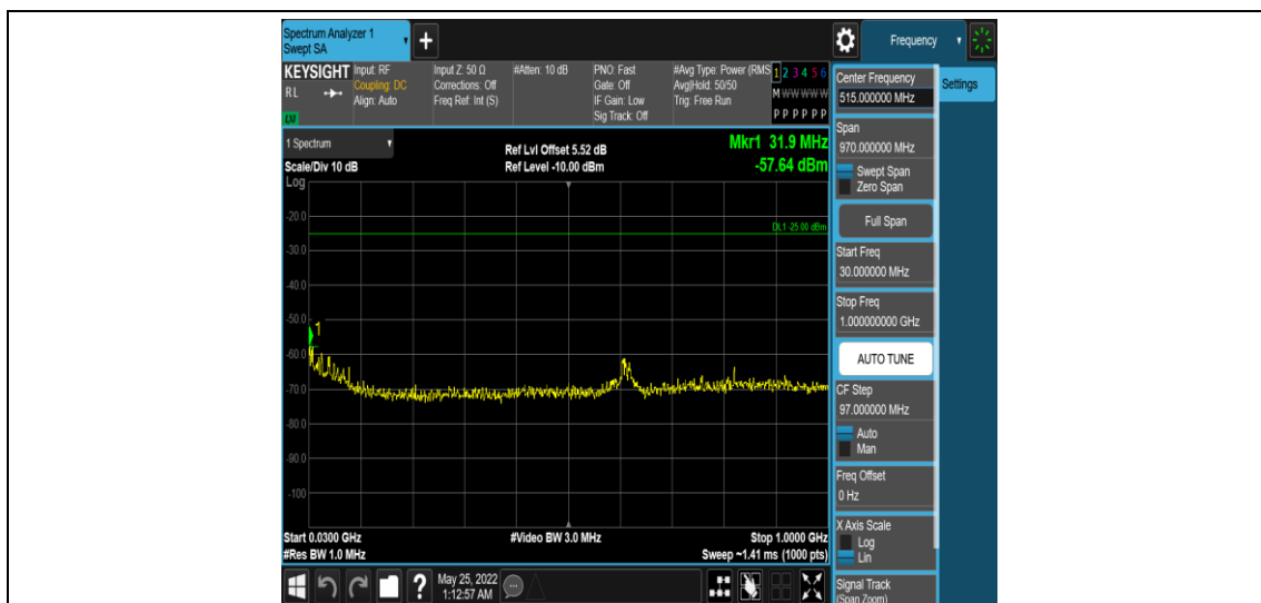
Band7-10MHz-QPSK-21400-1RB#0-Range3:30~1000MHz
