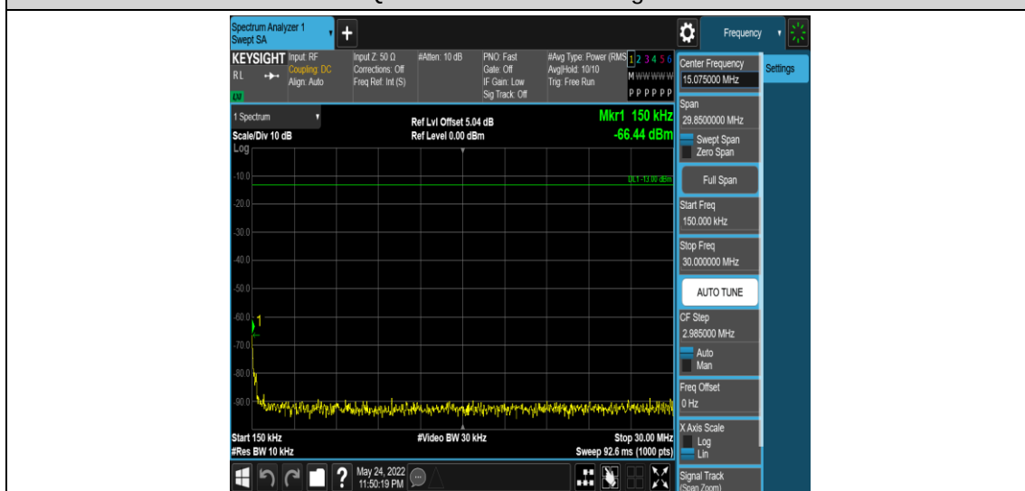
Band5-3MHz-16QAM-20525-1RB#0-Range2:0.15~30MHz
