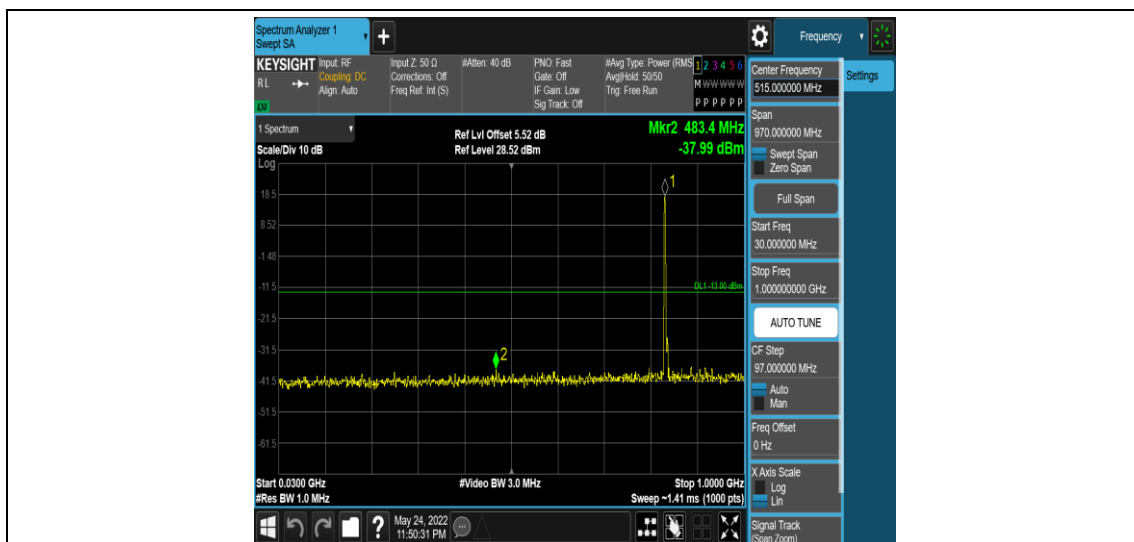
Band5-3MHz-16QAM-20525-1RB#0-Range3:30~1000MHz
