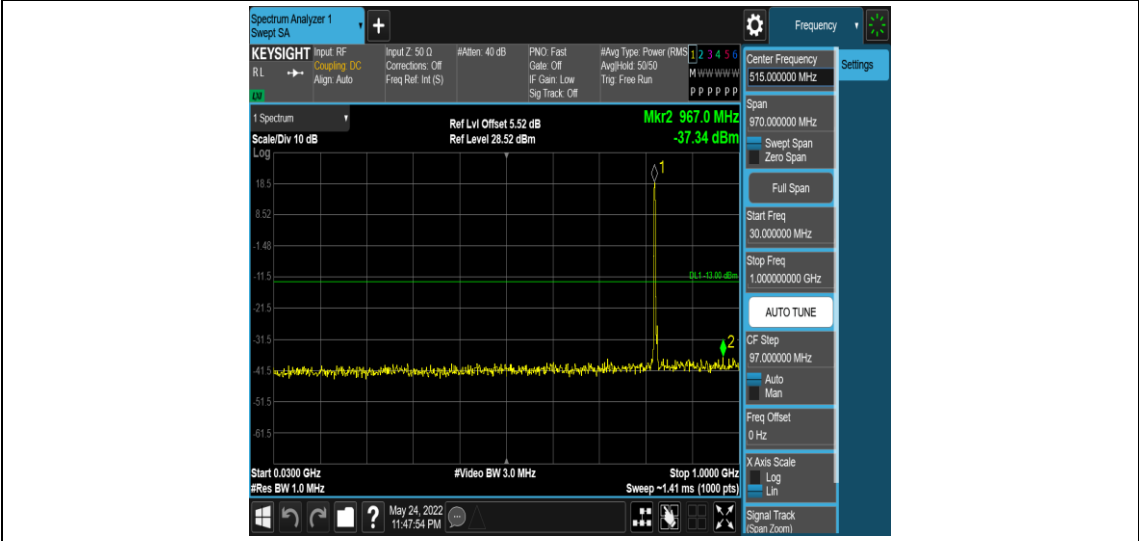
Band5-3MHz-QPSK-20415-1RB#0-Range3:30~1000MHz
