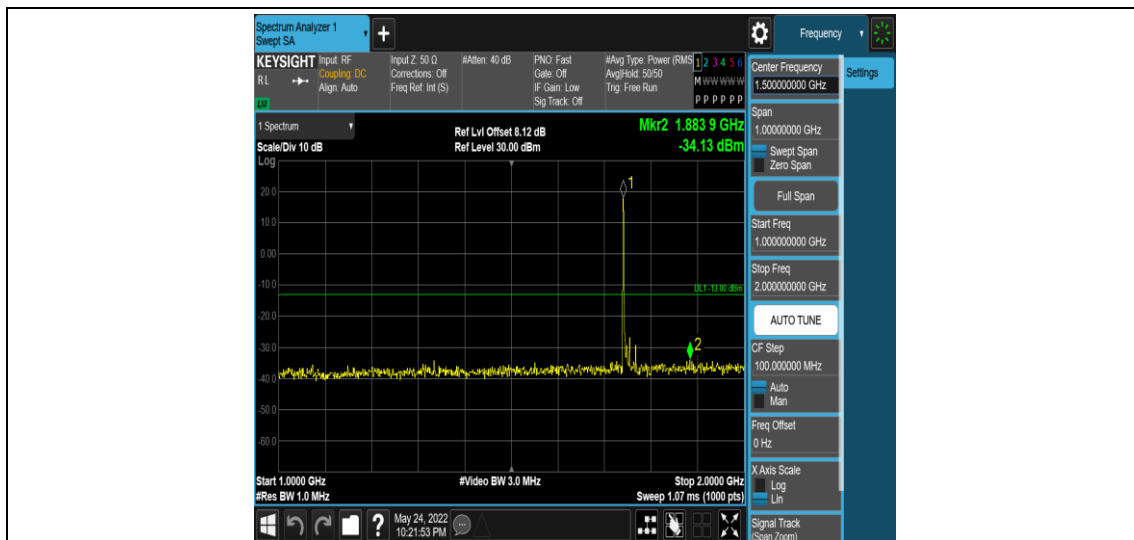
Band4-15MHz-QPSK-20325-1RB#0-Range4:1000~2000MHz
