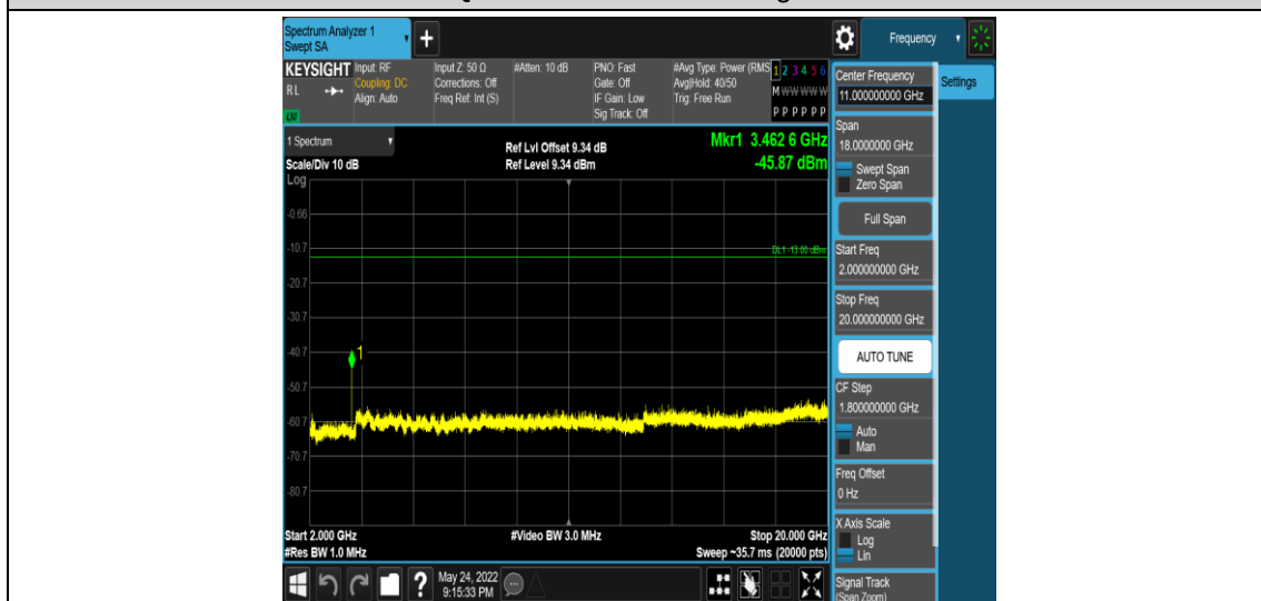
Band4-3MHz-16QAM-20175-1RB#0-Range5:2000~20000MHz
