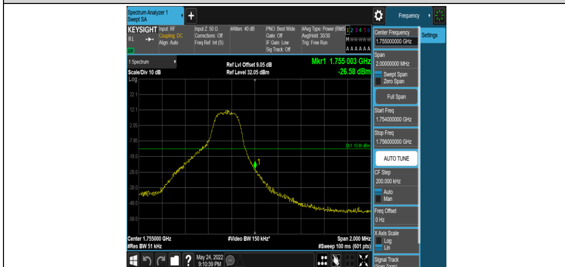
Band4-3MHz-16QAM-20385-1RB#14
