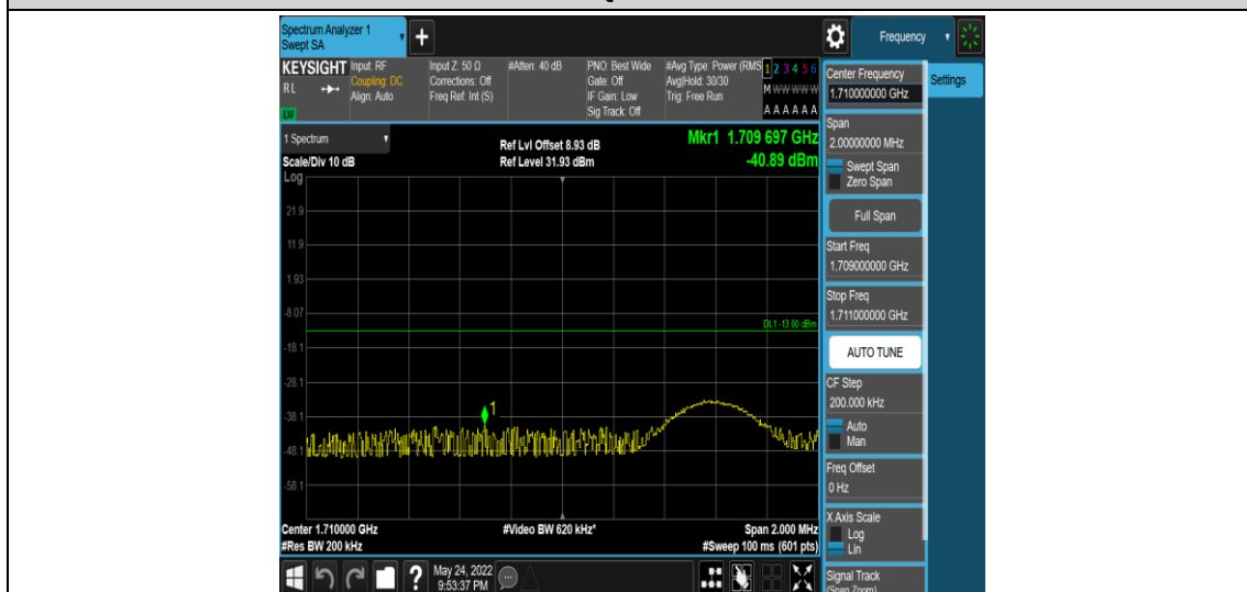
Band4-10MHz-QPSK-20000-1RB#49
