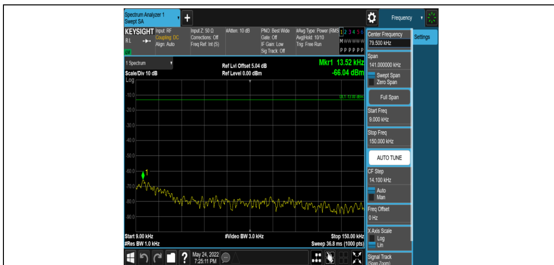
Band2-5MHz-16QAM-19175-1RB#0-Range1:0.009~0.15MHz
