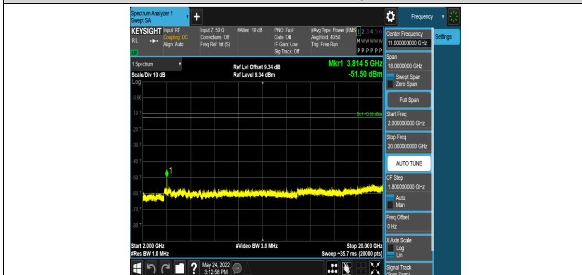
Band2-3MHz-16QAM-19185-1RB#0-Range5:2000~20000MHz
