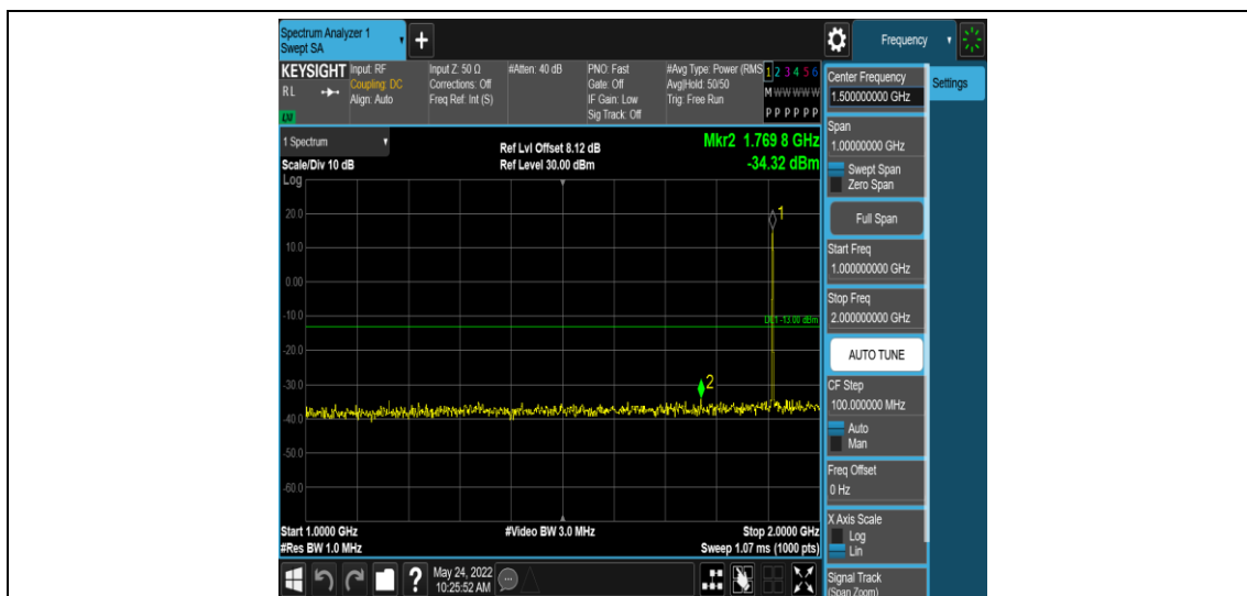
Band2-1.4MHz-16QAM-19193-1RB#0-Range4:1000~2000MHz
