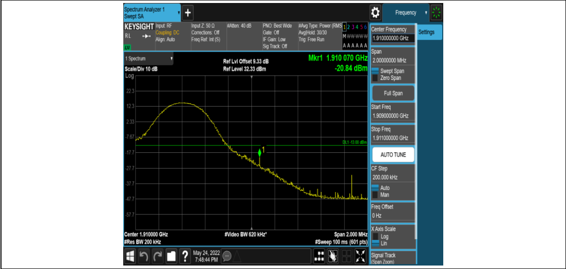
Band2-10MHz-QPSK-19150-1RB#49
