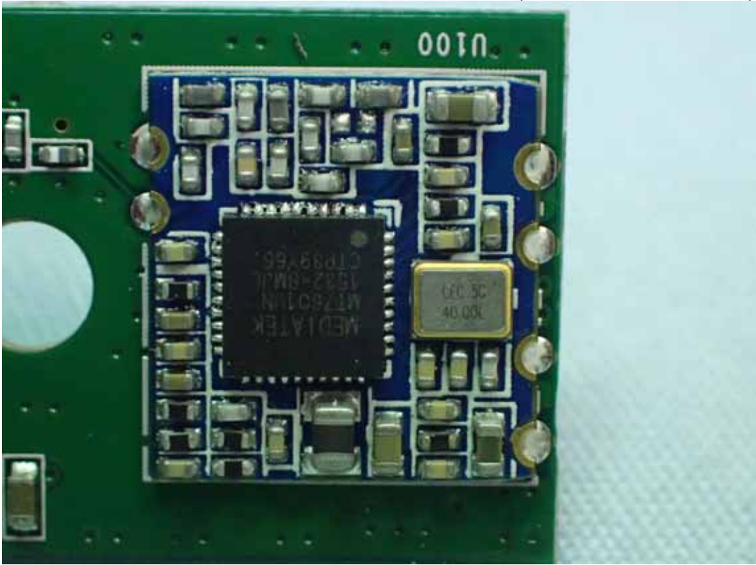
Figure 7 Internal View (RF Module, Front View)
