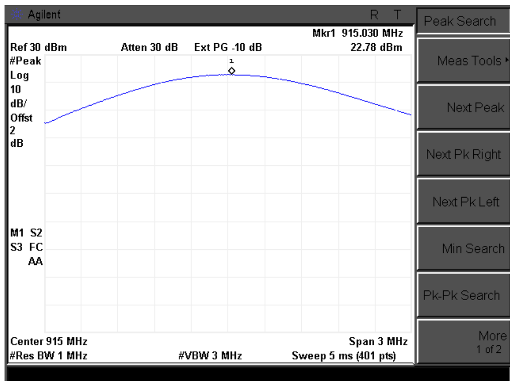
Peak output Power plot on channel 64
