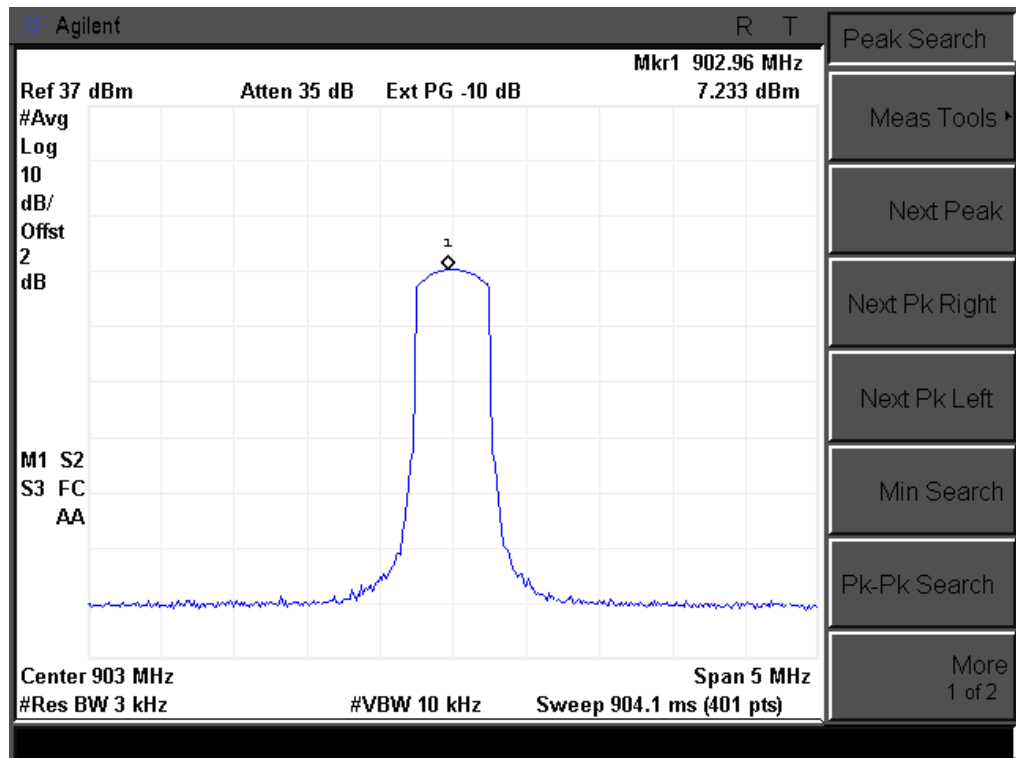
Power spectral density plot on channel 63
