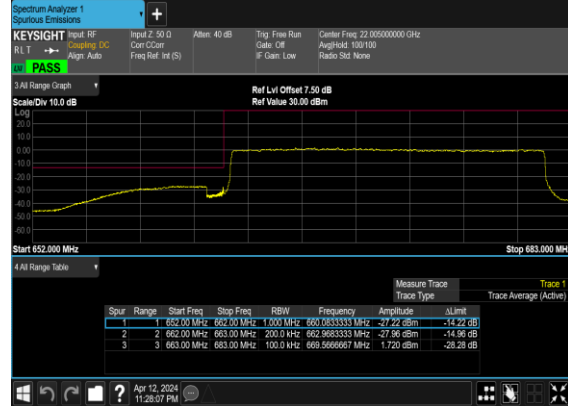
B2_N71(20M)_DFT-s- OFDM_QPSK_Outer_Full_Low_CH
