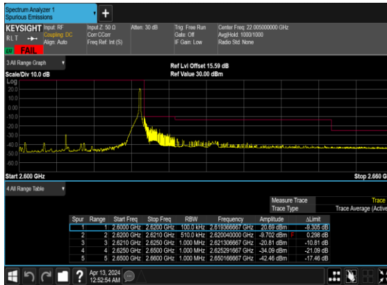
N38(25M)_DFT-s- OFDM_BPSK_Edge_1RB_Right_High_CH
