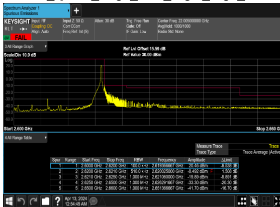
N38(25M)_DFT-s- OFDM_QPSK_Edge_1RB_Right_High_CH
