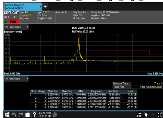
N7(50M)_DFT-s- OFDM_BPSK_Edge_1RB_Right_High_CH
