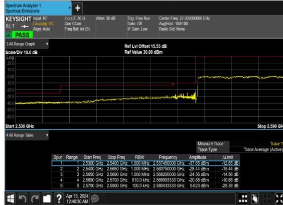
N38(25M)_DFT-s- OFDM_QPSK_Outer_Full_Low_CH
