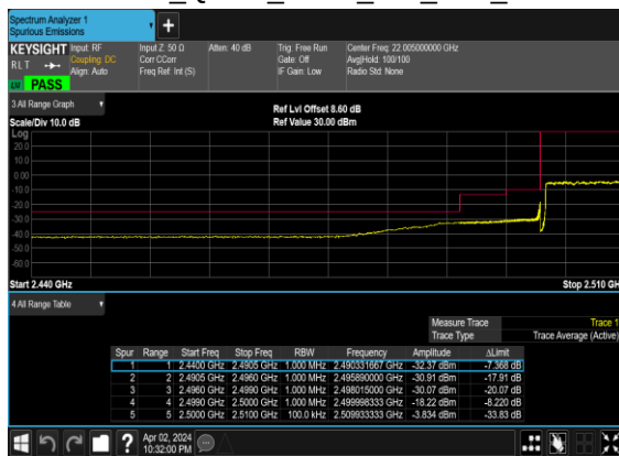
N7(50M)_DFT-s- OFDM_QPSK_Outer_Full_Low_CH
