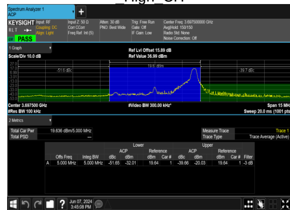
B2_N48(5M)_DFT-s-OFDM_QPSK_Edge_1RB_Right_High_CH
