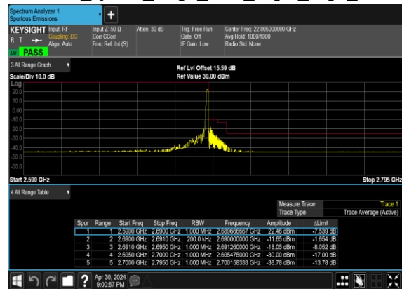
B2_N41(10M)_DFT-s- OFDM_QPSK_Edge_1RB_Right_High_CH
