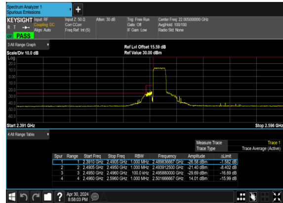
B2_N41(10M)_DFT-s- OFDM_QPSK_Outer_Full_Low_CH
