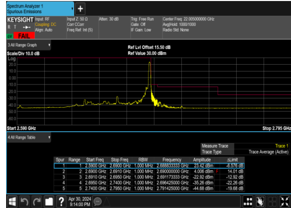
B2_N41(50M)_DFT-s-OFDM_BPSK_Edge_1RB_Right_High_CH
