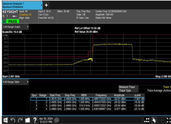
B2_N41(50M)_DFT-s-OFDM_QPSK_Outer_Full_Low_CH
