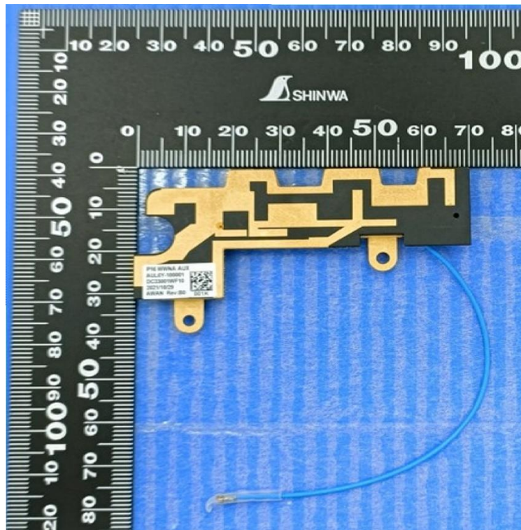
WWAN Aux Antenna
