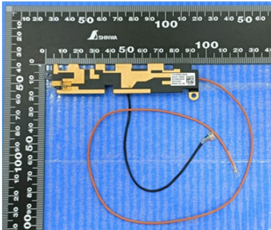
WWAN Main Antenna
