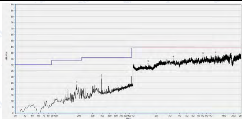
(30MHz to 25GHz, Antenna Horizontal @8-DPSK, channel 78)
