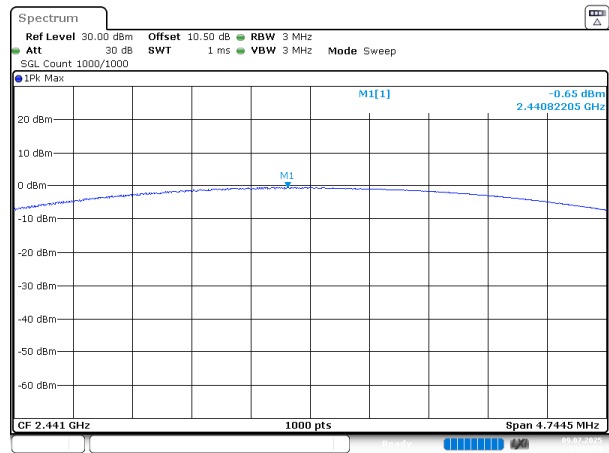
BDR_DH1_Middle
