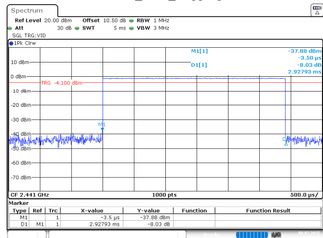
BDR_DH5_Hopping
