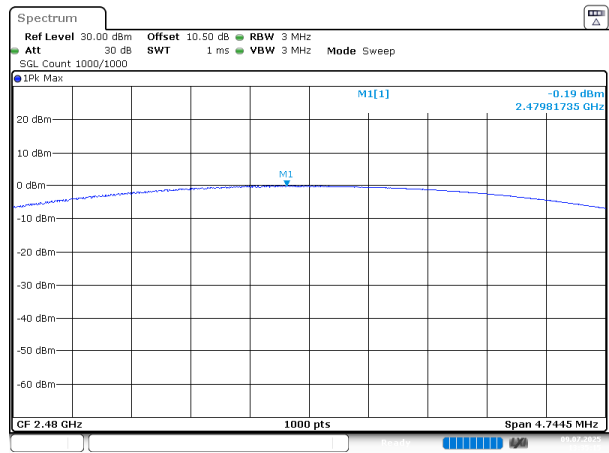
BDR_DH1_High
