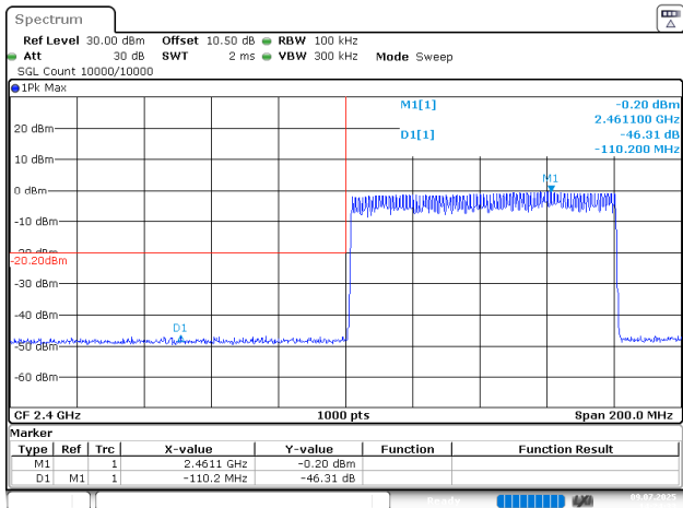
3EDR_DH1_Hopping_Lower
