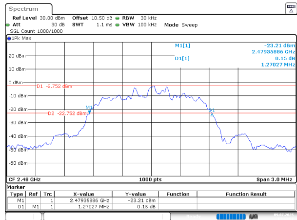
2EDR_DH1_High
