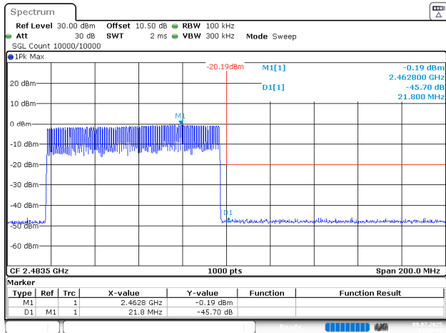
BDR_DH1_Hopping_Upper
