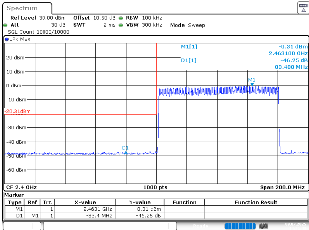
2EDR_DH1_Hopping_Lower
