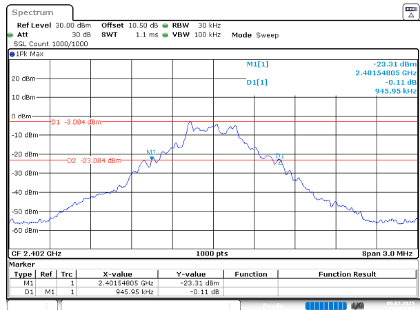
BDR_DH1_Low
