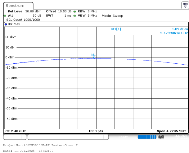
BDR_DH1_High
