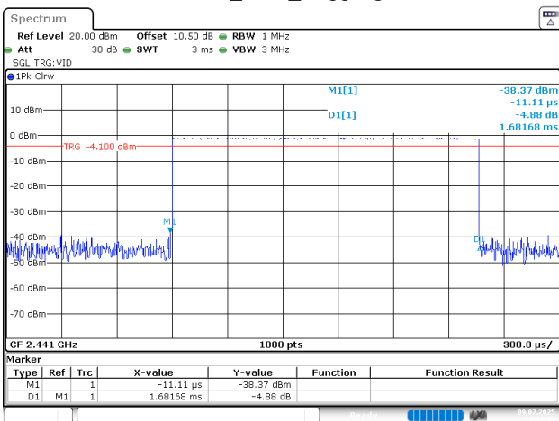
BDR_DH3_Hopping
