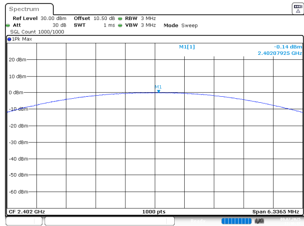
2EDR_DH1_Low
