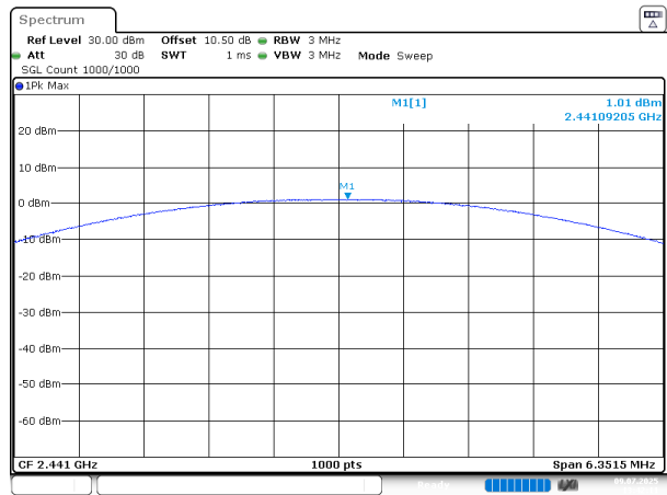
2EDR_DH1_Middle
