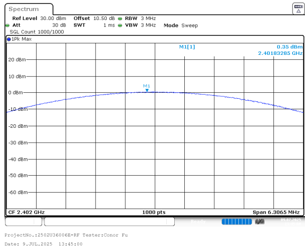
3EDR_DH1_Low
