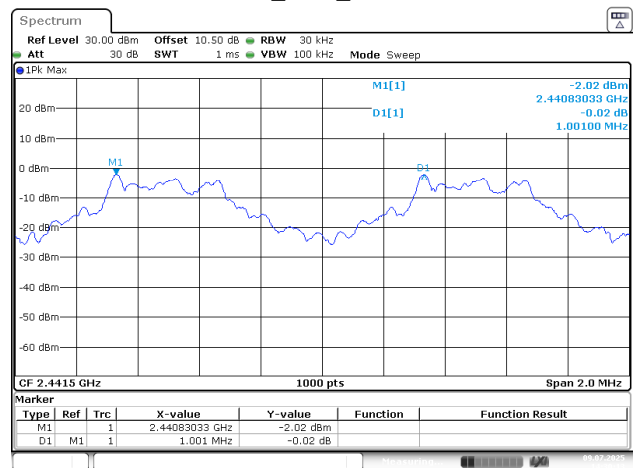
BDR_DH1_Middle
