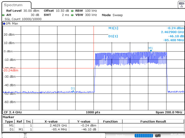
BDR_DH1_Hopping_Lower
