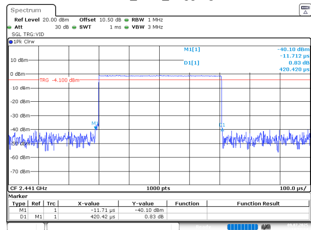
BDR_DH1_Hopping
