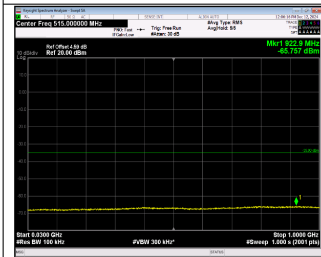
7-7-15MHz-10MHz-QPSK-QPSK-21051-21171-1RB#74-0 RB#0-30~1000MHz-PASS
