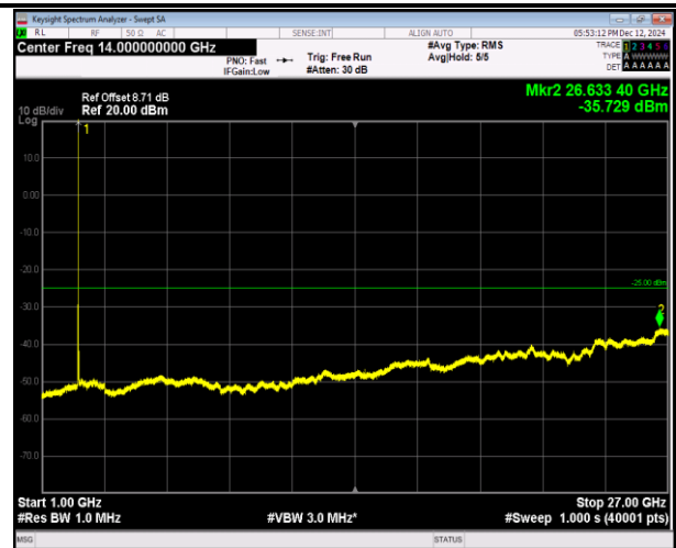
7-7-20MHz-10MHz-16QAM-16QAM-20850-20994-1RB#99- 0RB#0-1000~27000MHz-PASS
