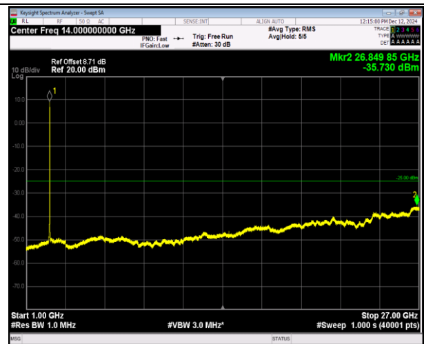
7-7-15MHz-10MHz-16QAM-16QAM-21277-21397-75RB#0- 50RB#0-1000~27000MHz-PASS
