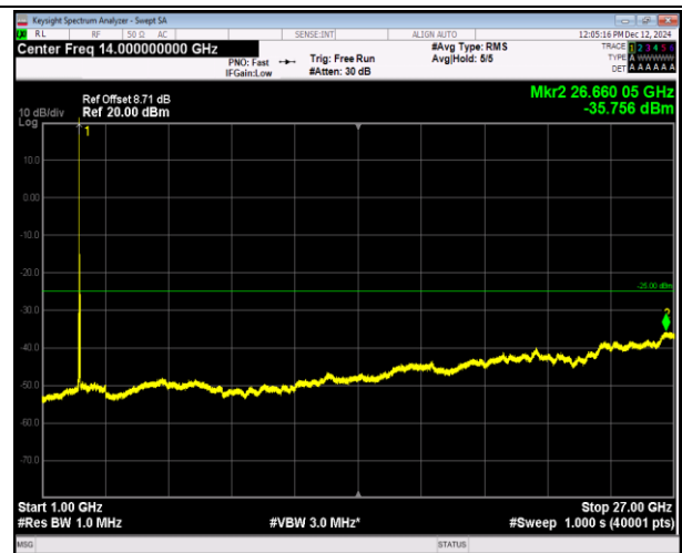
7-7-15MHz-10MHz-QPSK-QPSK-21051-21171-1RB#0-0RB #0-1000~27000MHz-PASS
