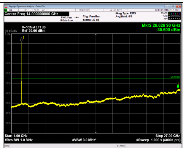
7-7-15MHz-10MHz-QPSK-QPSK-21277-21397-1RB#0-1RB #49-1000~27000MHz-PASS
