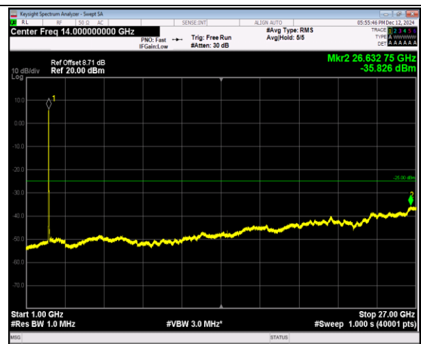
7-7-20MHz-10MHz-16QAM-16QAM-20850-20994-100RB# 0-50RB#0-1000~27000MHz-PASS
