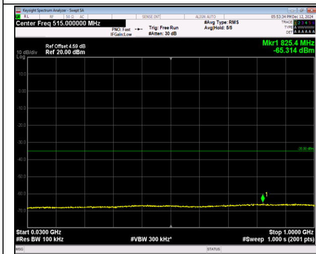
7-7-20MHz-10MHz-QPSK-QPSK-20850-20994-1RB#0-1 RB#49-30~1000MHz-PASS
