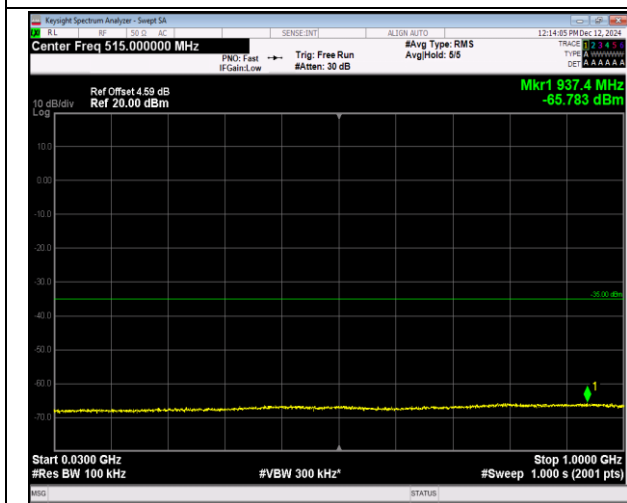
7-7-15MHz-10MHz-QPSK-QPSK-21277-21397-75RB#0-5 ORB#0-30~1000MHz-PASS
