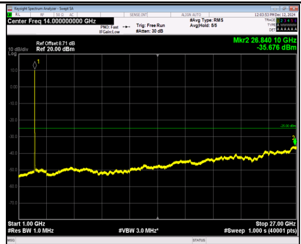
7-7-15MHz-10MHz-QPSK-QPSK-20825-20945-75RB#0-50 RB#0-1000~27000MHz-PASS
