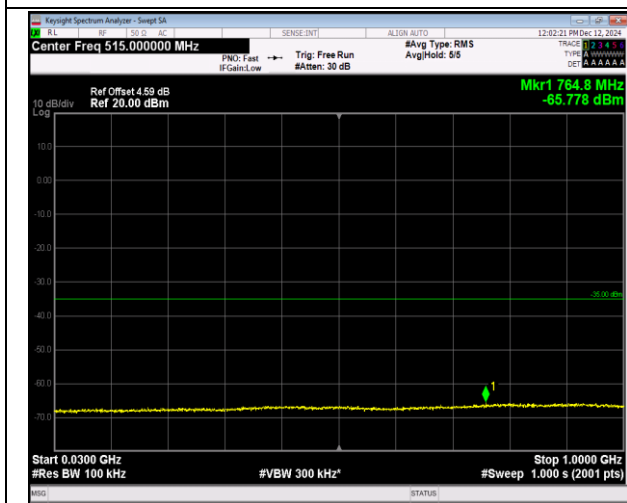
7-7-15MHz-10MHz-QPSK-QPSK-20825-20945-1RB#0-1 RB#49-30~1000MHz-PASS
