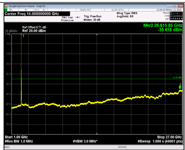
7-7-15MHz-10MHz-16QAM-16QAM-20825-20945-1RB#0-0 RB#0-1000~27000MHz-PASS
