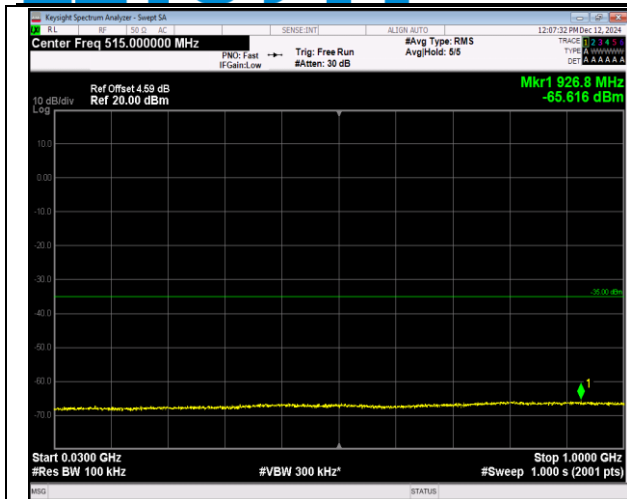
7-7-15MHz-10MHz-QPSK-QPSK-21051-21171-1RB#0-1 RB#49-30~1000MHz-PASS
