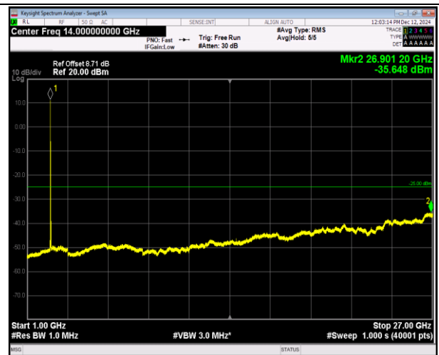
7-7-15MHz-10MHz-16QAM-16QAM-20825-20945-1RB#0-1 RB#49-1000~27000MHz-PASS
