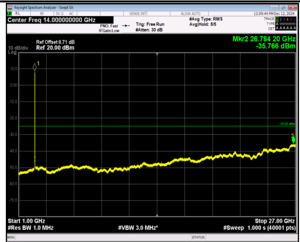
7-7-15MHz-10MHz-16QAM-16QAM-21051-21171-75RB#0- 50RB#0-1000~27000MHz-PASS
