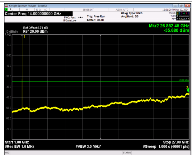
7-7-15MHz-10MHz-QPSK-QPSK-20825-20945-1RB#74-0R B#0-1000~27000MHz-PASS
