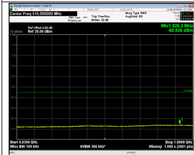
7-7-15MHz-10MHz-QPSK-QPSK-21051-21171-75RB#0-5 ORB#0-30~1000MHz-PASS
