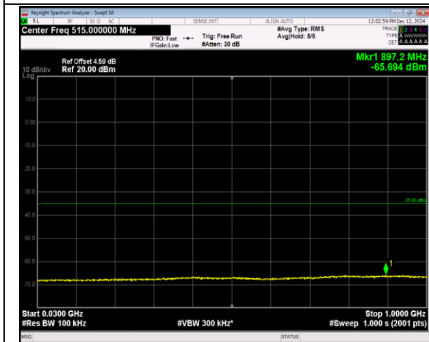
7-7-15MHz-10MHz-16QAM-16QAM-20825-20945-1RB#0 -1RB#49-30~1000MHz-PASS
