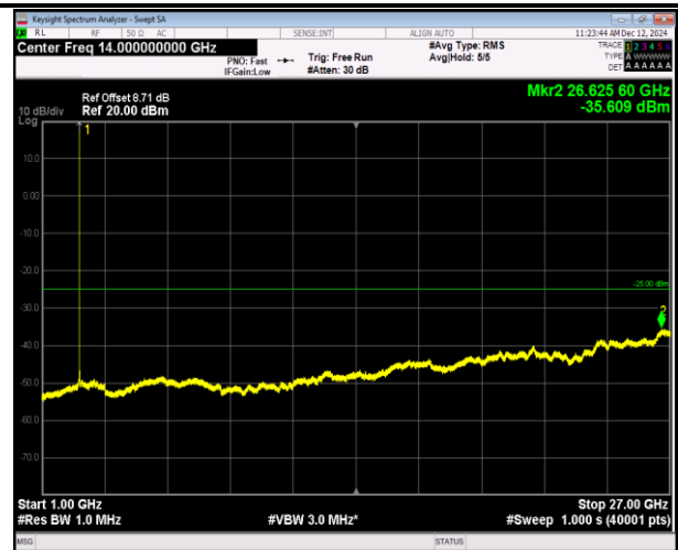
7-7-10MHz-20MHz-QPSK-QPSK-21206-21350-1RB#49-0R B#0-1000~27000MHz-PASS
