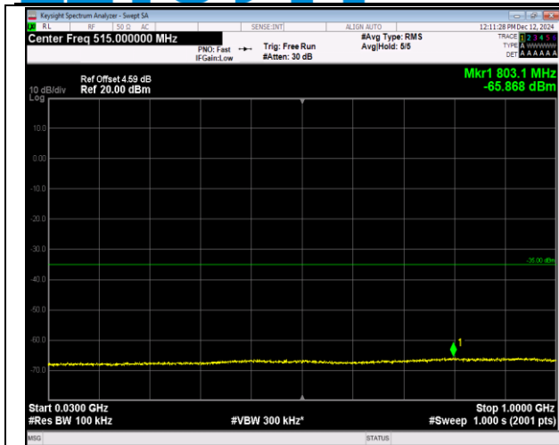
7-7-15MHz-10MHz-QPSK-QPSK-21277-21397-1RB#74-0 RB#0-30~1000MHz-PASS
