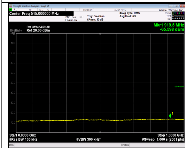
7-7-15MHz-10MHz-16QAM-16QAM-20825-20945-1RB#0 -ORB#0-30~1000MHz-PASS
