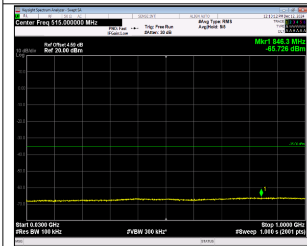
7-7-15MHz-10MHz-QPSK-QPSK-21277-21397-1RB#0-0 RB#0-30~1000MHz-PASS
