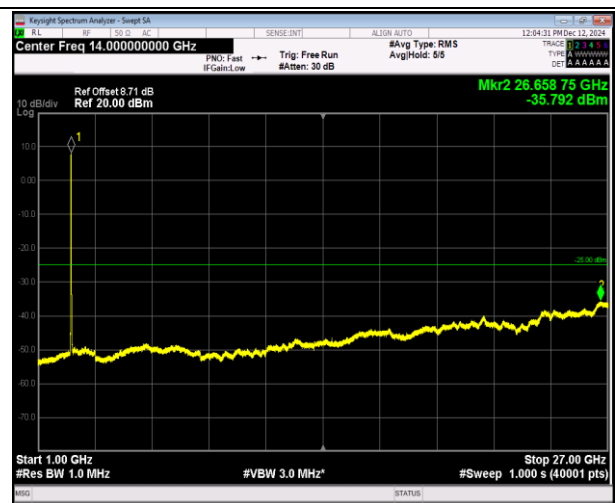
7-7-15MHz-10MHz-16QAM-16QAM-20825-20945-75RB#0- 50RB#0-1000~27000MHz-PASS
