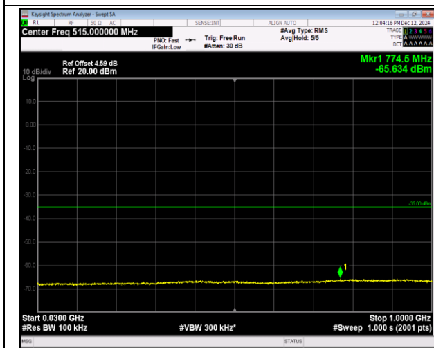
7-7-15MHz-10MHz-16QAM-16QAM-20825-20945-75RB# 0-50RB#0-30~1000MHz-PASS
