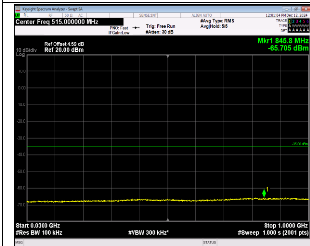
7-7-15MHz-10MHz-QPSK-QPSK-20825-20945-1RB#74-0 RB#0-30~1000MHz-PASS
