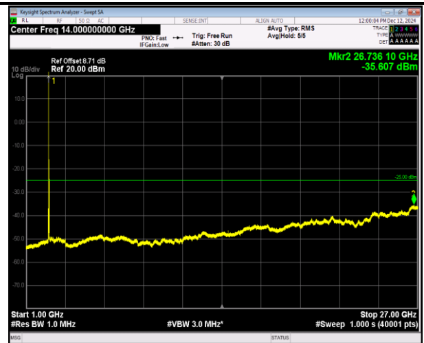
7-7-15MHz-10MHz-QPSK-QPSK-20825-20945-1RB#0-0RB #0-1000~27000MHz-PASS
