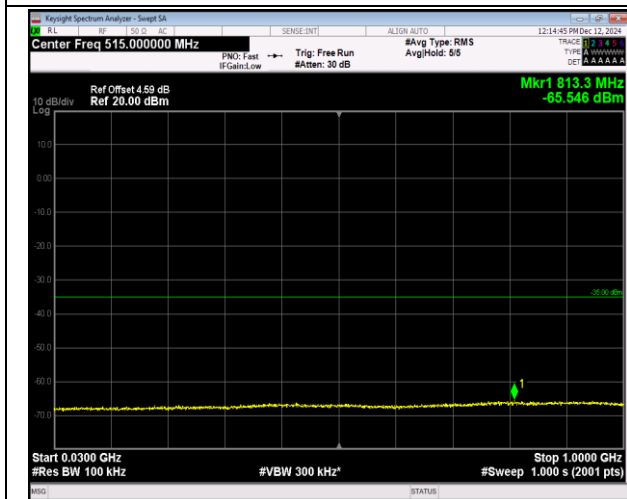
7-7-15MHz-10MHz-16QAM-16QAM-21277-21397-75RB# 0-50RB#0-30~1000MHz-PASS
