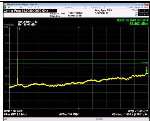
7-7-10MHz-20MHz-16QAM-16QAM-21206-21350-1RB#0-0 RB#0-1000~27000MHz-PASS
