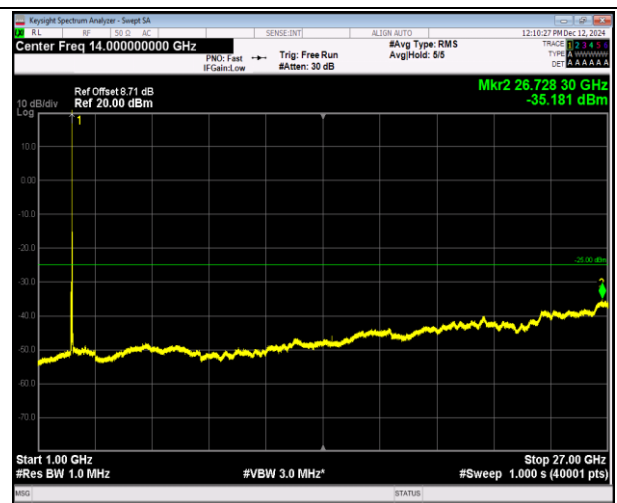
7-7-15MHz-10MHz-QPSK-QPSK-21277-21397-1RB#0-0RB #0-1000~27000MHz-PASS
