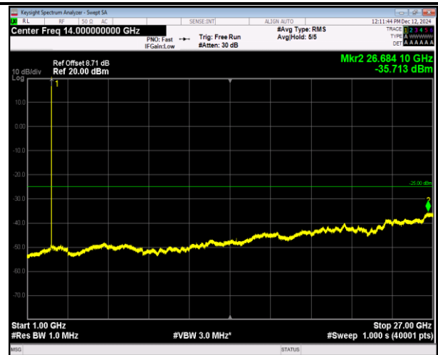
7-7-15MHz-10MHz-QPSK-QPSK-21277-21397-1RB#74-0R B#0-1000~27000MHz-PASS
