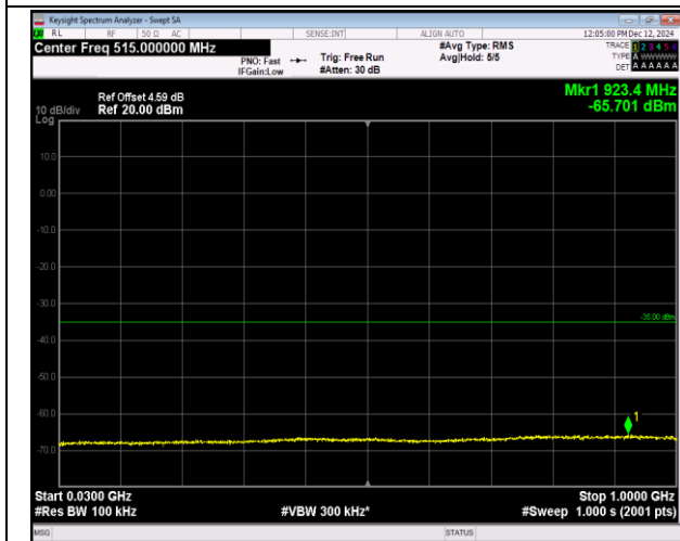
7-7-15MHz-10MHz-QPSK-QPSK-21051-21171-1RB#0-0 RB#0-30~1000MHz-PASS
