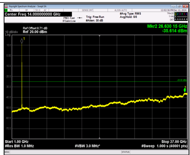
7-7-15MHz-10MHz-QPSK-QPSK-20825-20945-1RB#0-1RB #49-1000~27000MHz-PASS
