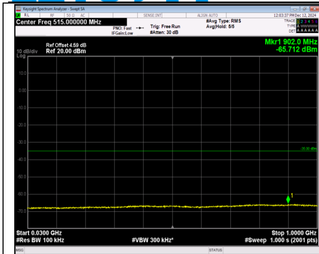
7-7-15MHz-10MHz-QPSK-QPSK-20825-20945-75RB#0-5 ORB#0-30~1000MHz-PASS
