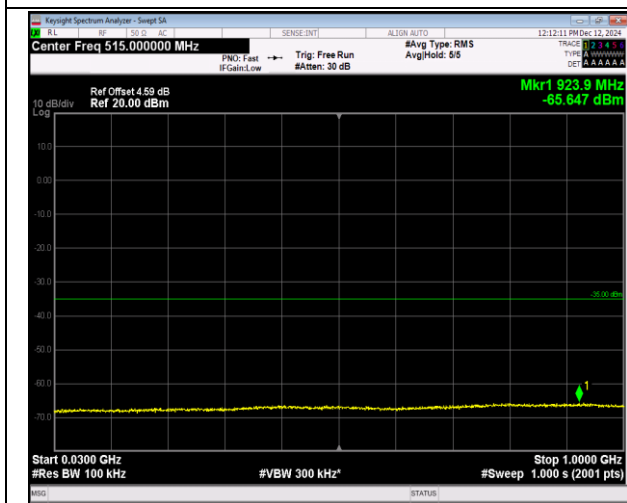
7-7-15MHz-10MHz-16QAM-16QAM-21277-21397-1RB#7 4-0RB#0-30~1000MHz-PASS
