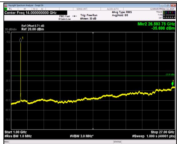
7-7-15MHz-10MHz-QPSK-QPSK-21051-21171-75RB#0-50 RB#0-1000~27000MHz-PASS
