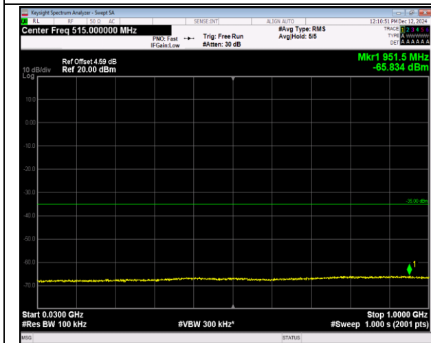
7-7-15MHz-10MHz-16QAM-16QAM-21277-21397-1RB#0 -0RB#0-30~1000MHz-PASS
