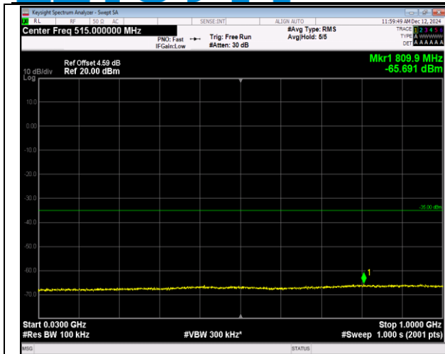
7-7-15MHz-10MHz-QPSK-QPSK-20825-20945-1RB#0-0 RB#0-30~1000MHz-PASS
