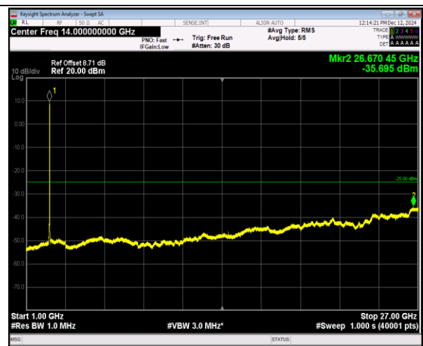
7-7-15MHz-10MHz-QPSK-QPSK-21277-21397-75RB#0-50 RB#0-1000~27000MHz-PASS
