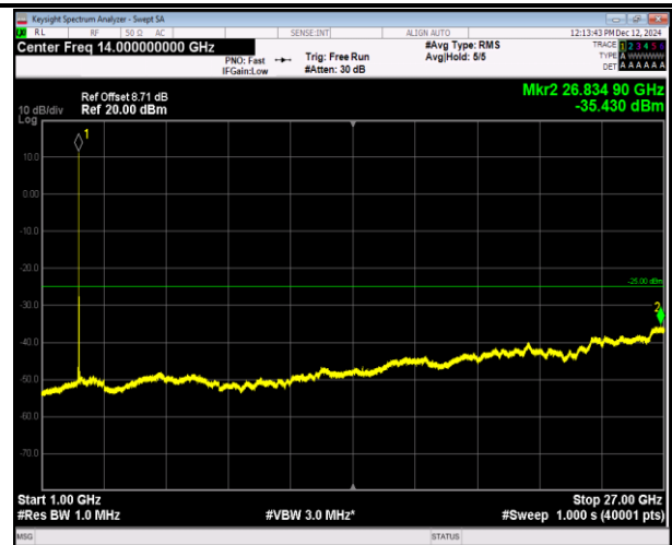
7-7-15MHz-10MHz-16QAM-16QAM-21277-21397-1RB#0-1 RB#49-1000~27000MHz-PASS
