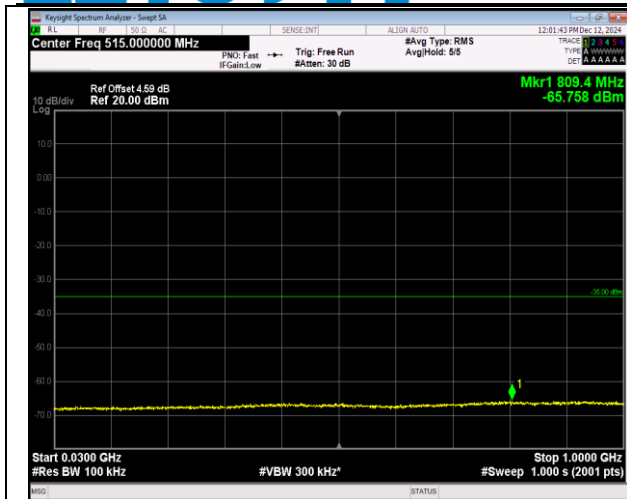
7-7-15MHz-10MHz-16QAM-16QAM-20825-20945-1RB#7 4-0RB#0-30~1000MHz-PASS
