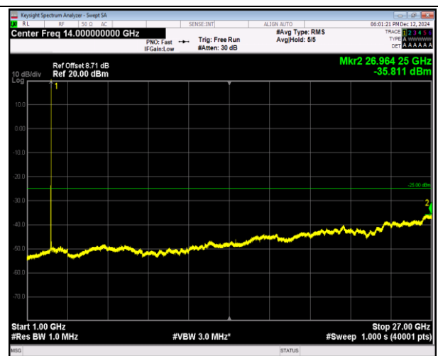
7-7-20MHz-10MHz-16QAM-16QAM-21051-21195-1RB#99- 0RB#0-1000~27000MHz-PASS
