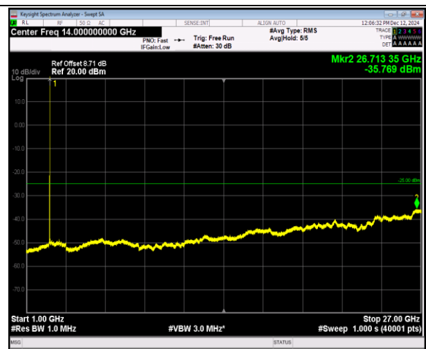
7-7-15MHz-10MHz-QPSK-QPSK-21051-21171-1RB#74-0R B#0-1000~27000MHz-PASS
