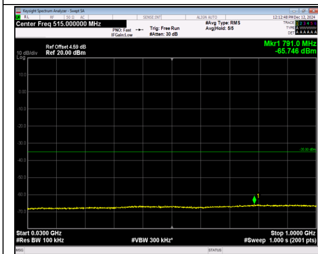
7-7-15MHz-10MHz-QPSK-QPSK-21277-21397-1RB#0-0-1 RB#49-30~1000MHz-PASS
