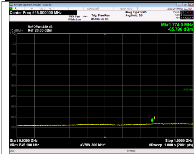
7-7-15MHz-10MHz-16QAM-16QAM-21051-21171-75RB# 0-50RB#0-30~1000MHz-PASS
