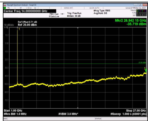
7-7-15MHz-10MHz-16QAM-16QAM-21277-21397-1RB#74- 0RB#0-1000~27000MHz-PASS
