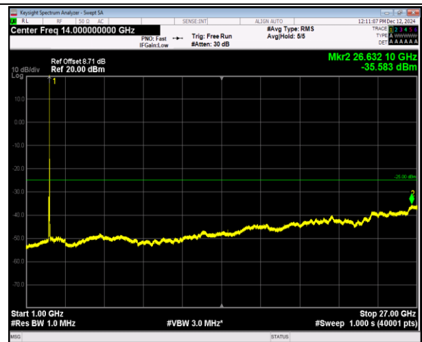
7-7-15MHz-10MHz-16QAM-16QAM-21277-21397-1RB#0-0 RB#0-1000~27000MHz-PASS
