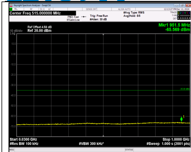
7-7-15MHz-10MHz-16QAM-16QAM-21277-21397-1RB#0 -1RB#49-30~1000MHz-PASS
