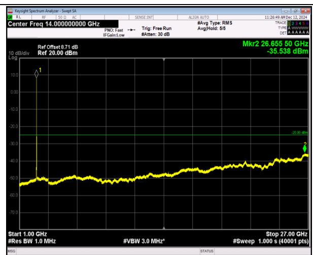
7-7-10MHz-20MHz-16QAM-16QAM-21206-21350-50RB#0- 100RB#0-1000~27000MHz-PASS
