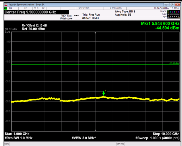
5-5-10MHz-10MHz-QPSK-QPSK-20476-20575-1RB#0-1RB #49-1000~10000MHz-PASS
