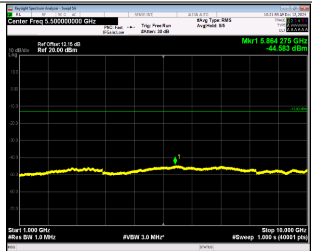
5-5-10MHz-10MHz-QPSK-QPSK-20476-20575-50RB#0-50 RB#0-1000~10000MHz-PASS
