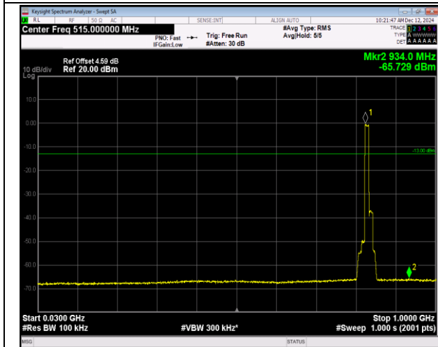
5-5-10MHz-10MHz-QPSK-QPSK-20476-20575-50RB#0-5 ORB#0-30~1000MHz-PASS
