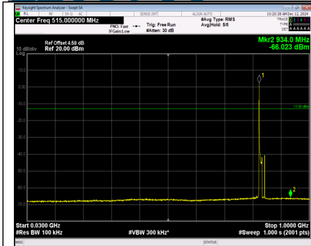
5-5-10MHz-10MHz-QPSK-QPSK-20476-20575-1RB#0-1 RB#49-30~1000MHz-PASS
