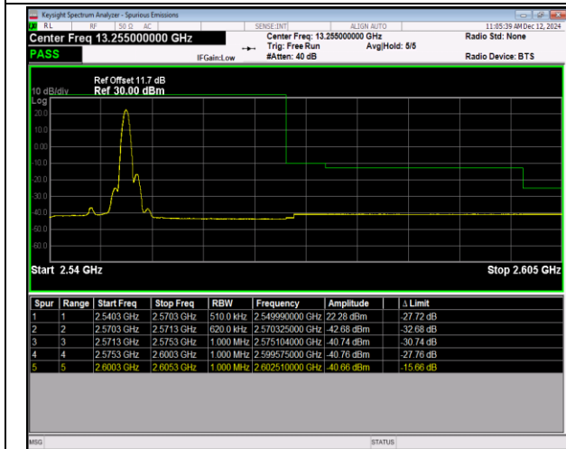
7-7-10MHz-20MHz-16QAM@16QAM-16QAM@16QAM-21206-21350-1RB#49@50RB#0-0RB#0@100RB#0-PASS
