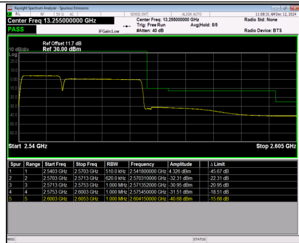
7-7-10MHz-20MHz-16QAM@16QAM-16QAM@16QAM-21206-21350-50RB#0@50RB#0-100RB#0@100RB#0-PASS
