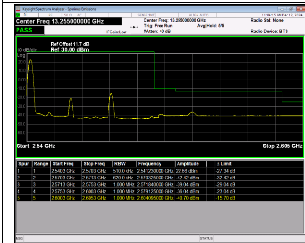
7-7-10MHz-20MHz-16QAM@16QAM-16QAM@16QAM-21206-21350-1RB#0@50RB#0-0RB#0@100RB#0-PASS
