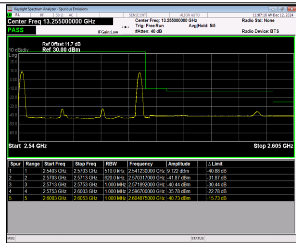
7-7-10MHz-20MHz-16QAM@16QAM-16QAM@16QAM-21206-21350-1RB#0@50RB#0-1RB#99@100RB#0-PASS
