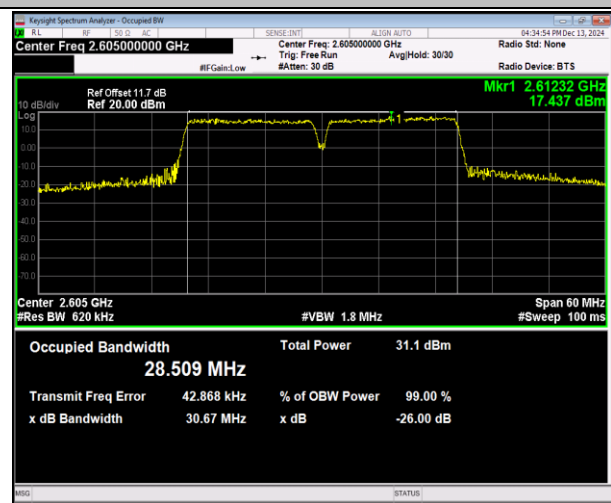
41(2555-2655)-41(2555-2655)-15MHz-15MHz-16QAM-16Q AM-40665-40815-75RB#0-75RB#0-PASS
