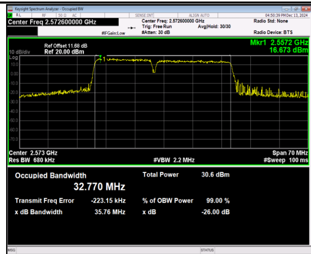
41(2555-2655)-41(2555-2655)-15MHz-20MHz-16QAM-16Q AM-40318-40489-75RB#0-100RB#0-PASS
