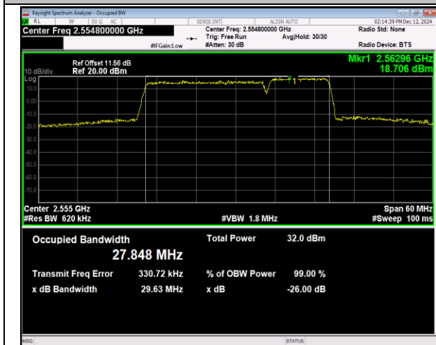
7-7-20MHz-10MHz-QPSK-QPSK-21251-21395-100RB#0-50RB#0-PASS
