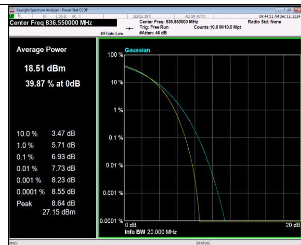
5-5-10MHz-10MHz-16QAM-16QAM-20476-20575-50RB#0 -50RB#0-PASS
