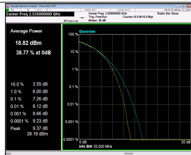
7-7-20MHz-20MHz-16QAM-16QAM-21001-21199-100RB# 0-100RB#0-PASS
