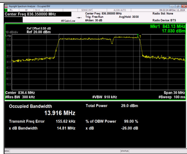
5-5-10MHz-5MHz-16QAM-16QAM-20500-20572-50RB#0-2 5RB#0-PASS
