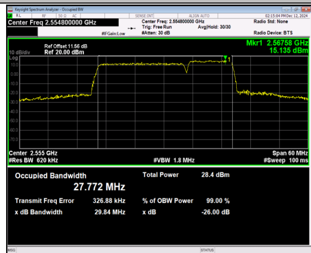
7-7-20MHz-10MHz-16QAM-16QAM-21251-21395-100RB#0-50RB#0-PASS
