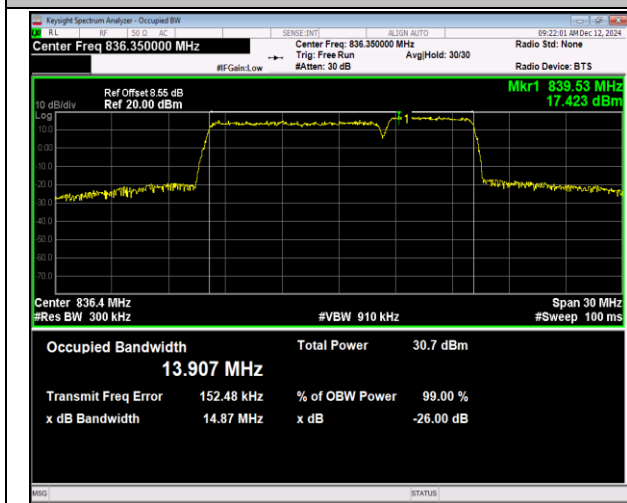
5-5-10MHz-5MHz-QPSK-QPSK-20500-20572-50RB#0-25 RB#0-PASS
