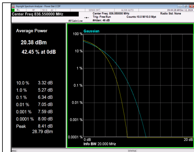
5-5-10MHz-10MHz-QPSK-QPSK-20476-20575-50RB#0-5 ORB#0-PASS
