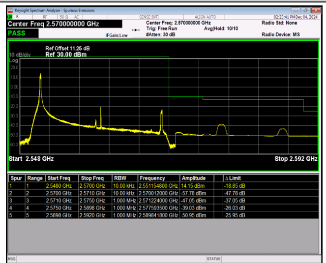
Band7-20MHz-16QAM-21350-100RB#0
