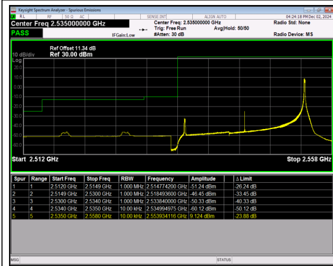
Band41-20MHz-16QAM-41140-1RB#0
