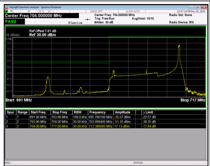
Band17-10MHz-16QAM-23800-1RB#0
