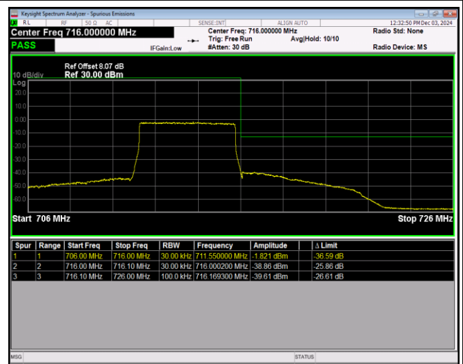
Band17-10MHz-QPSK-23780-1RB#49
