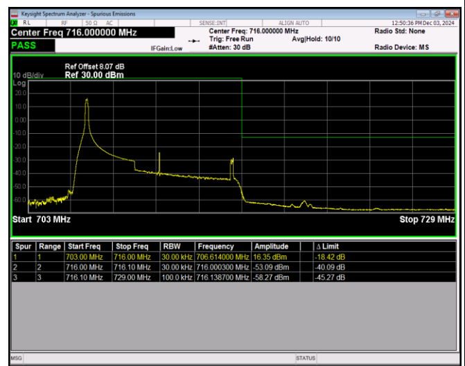
Band17-10MHz-64QAM-23800-50RB#0
