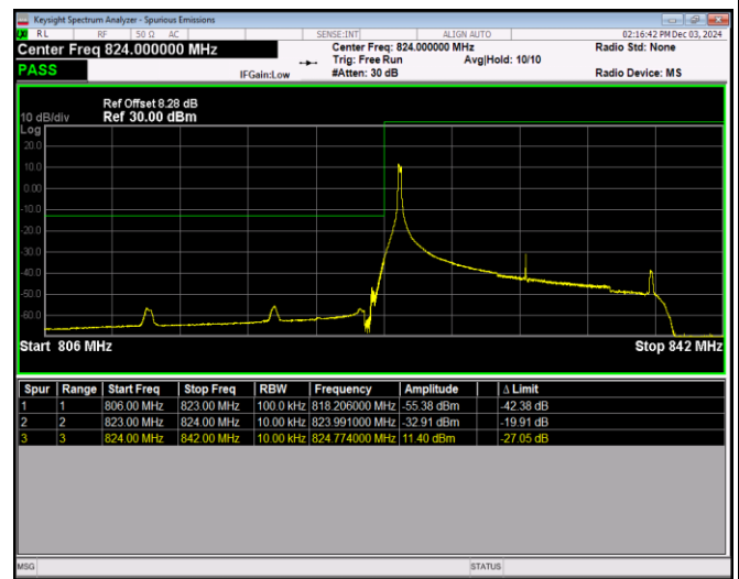
Band26-15MHz-QPSK-26865-75RB#0
