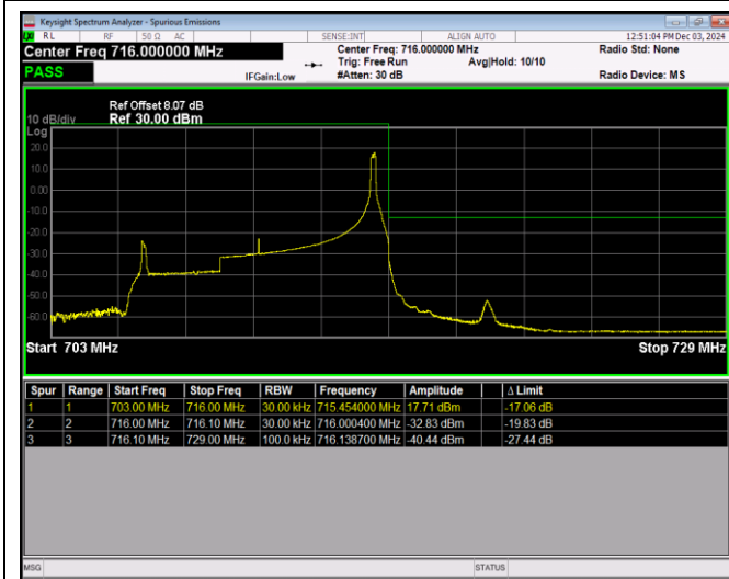
Band17-10MHz-16QAM-23780-1RB#0
