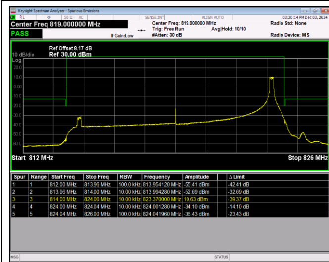
Band26-10MHz-64QAM-26740-1RB#0
