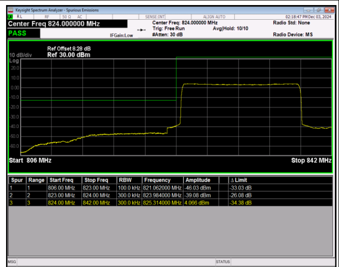
Band26-15MHz-QPSK-26965-1RB#74
