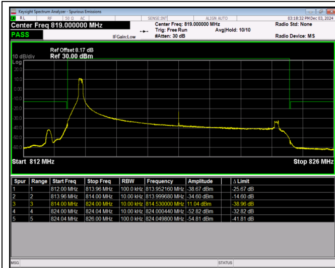
Band26-10MHz-64QAM-26740-50RB#0
