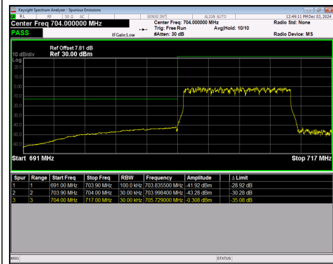
Band17-10MHz-64QAM-23800-1RB#49
