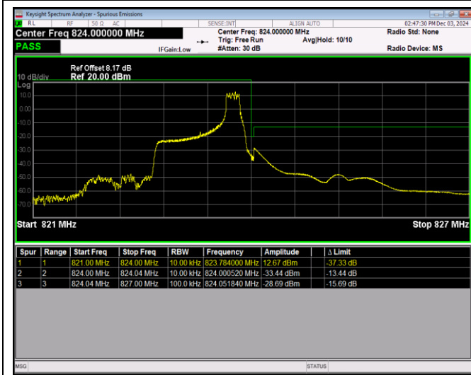
Band26-1.4MHz-16QAM-26797-1RB#0
