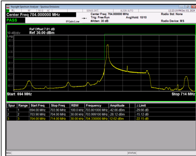
Band17-5MHz-64QAM-23755-25RB#0
