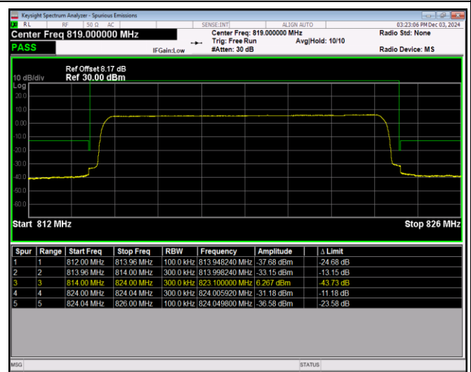
Band26-10MHz-64QAM-26740-1RB#49
