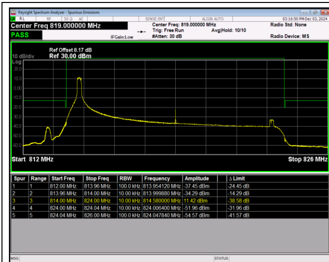
Band26-10MHz-QPSK-26740-50RB#0
