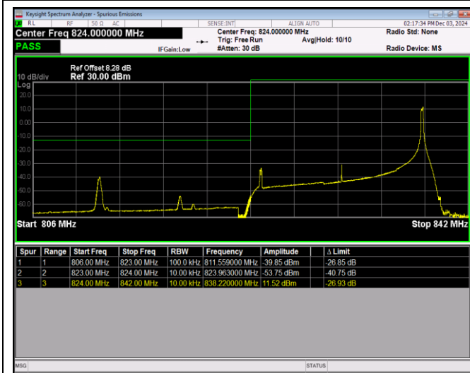
Band26-15MHz-QPSK-26965-1RB#0
