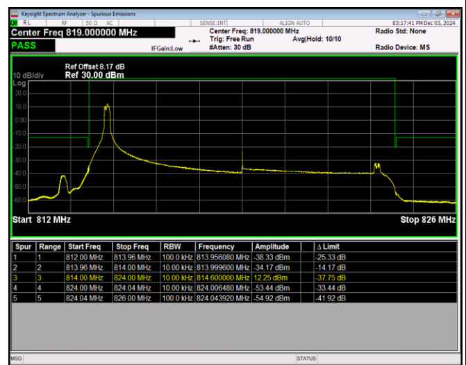
Band26-10MHz-16QAM-26740-50RB#0
