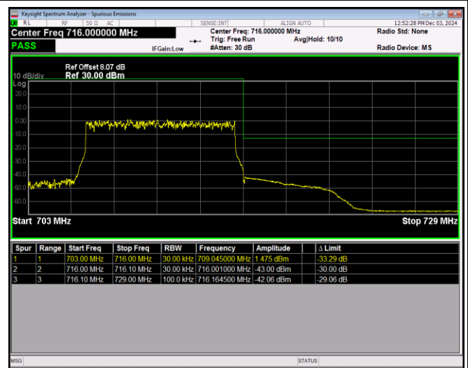
Band17-10MHz-16QAM-23780-1RB#49
