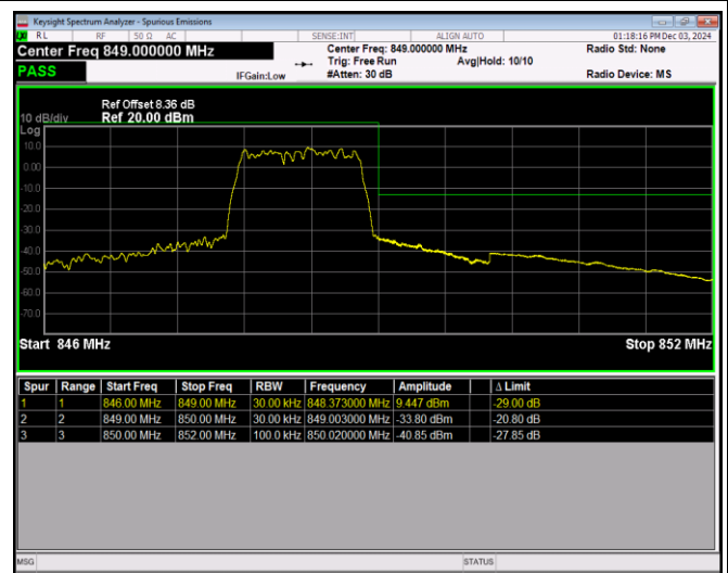
Band26-1.4MHz-64QAM-26697-1RB#5
