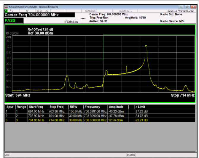
Band17-5MHz-64QAM-23825-1RB#0
