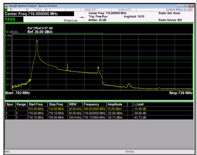
Band17-10MHz-QPSK-23800-50RB#0
