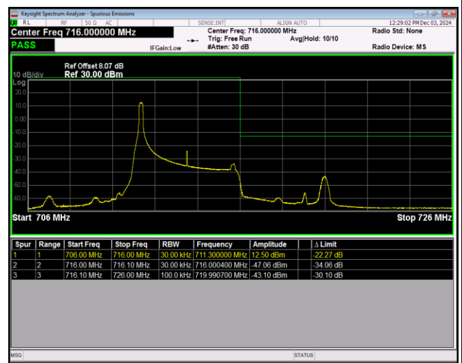
Band17-5MHz-64QAM-23825-25RB#0
