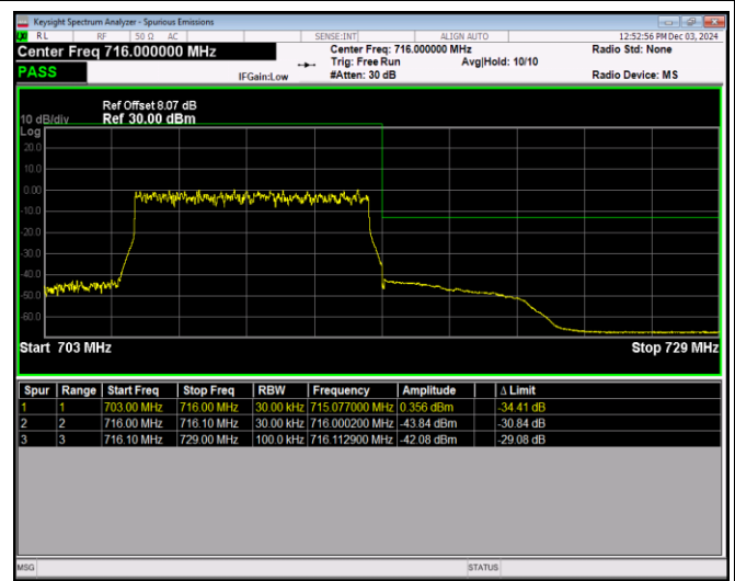
Band17-10MHz-64QAM-23780-1RB#49
