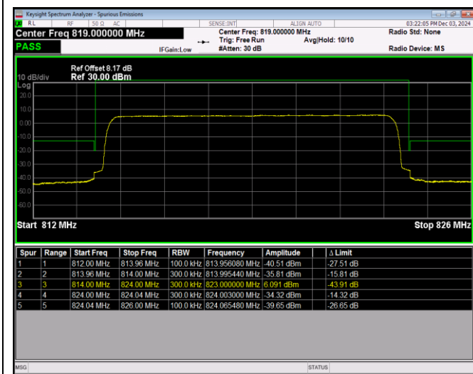
Band26-10MHz-16QAM-26740-1RB#49
