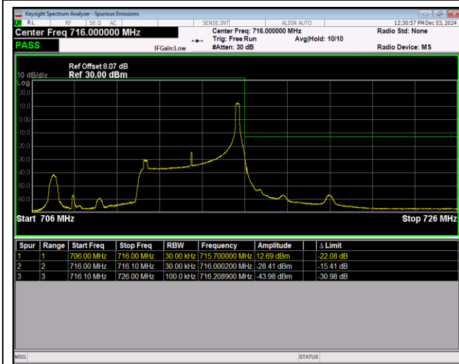
Band17-10MHz-QPSK-23780-1RB#0
