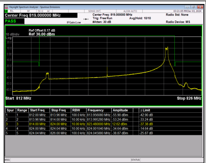
Band26-15MHz-QPSK-26865-1RB#0
