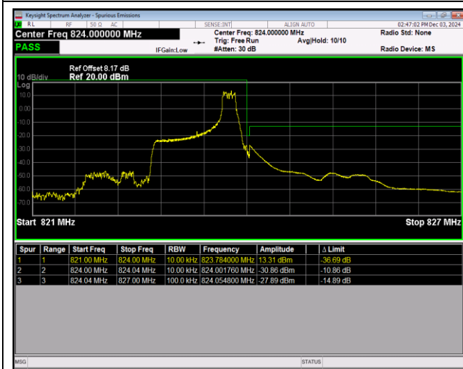
Band26-1.4MHz-QPSK-26797-1RB#0
