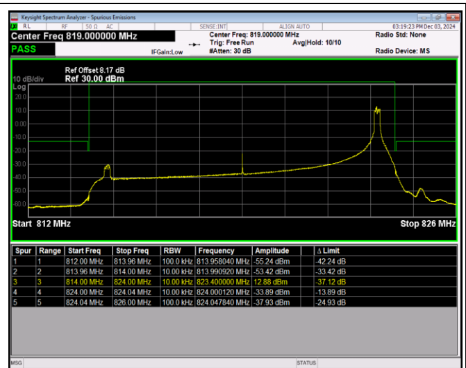
Band26-10MHz-16QAM-26740-1RB#0
