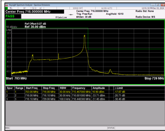
Band17-10MHz-64QAM-23780-1RB#0
