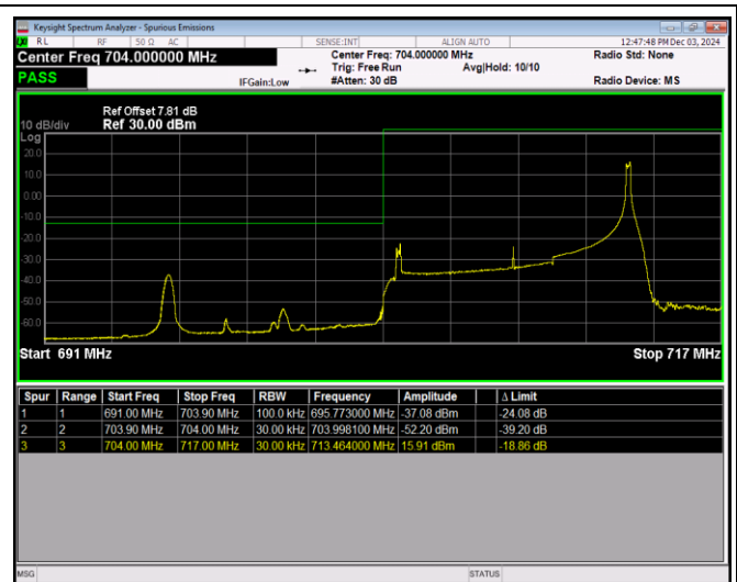
Band17-10MHz-64QAM-23800-1RB#0
