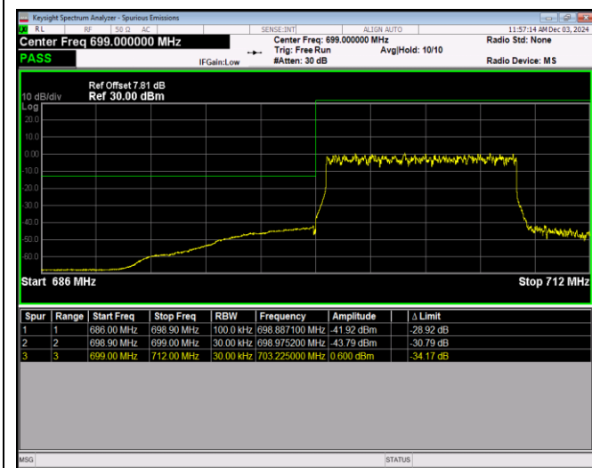
Band12-10MHz-QPSK-23130-1RB#49
