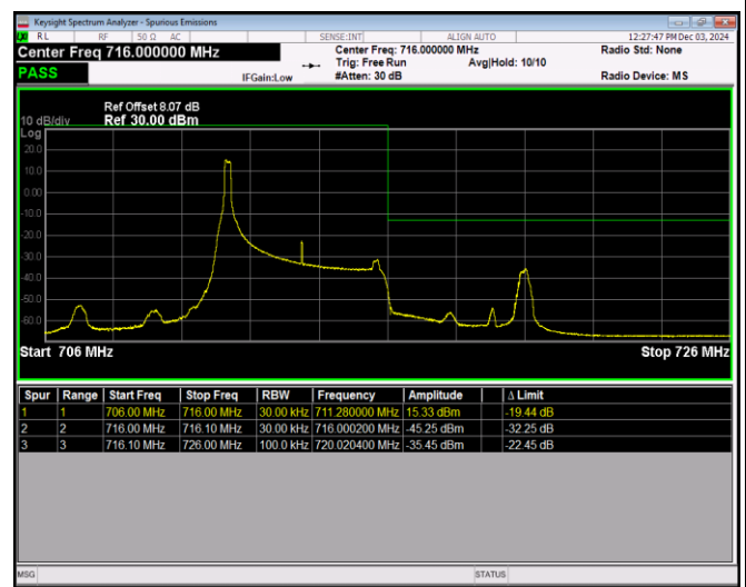
Band17-5MHz-QPSK-23825-25RB#0
