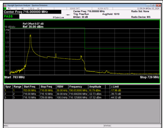
Band12-10MHz-64QAM-23130-50RB#0
