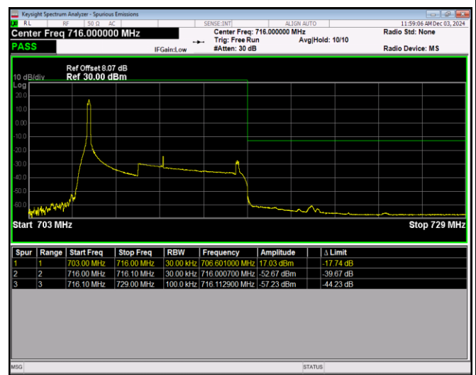
Band12-10MHz-16QAM-23130-50RB#0
