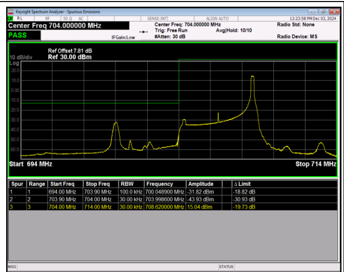
Band17-5MHz-QPSK-23825-1RB#0
