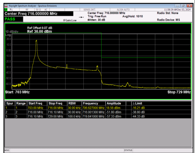
Band12-10MHz-QPSK-23130-50RB#0
