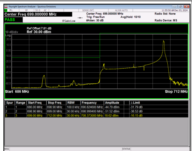
Band12-10MHz-QPSK-23130-1RB#0
