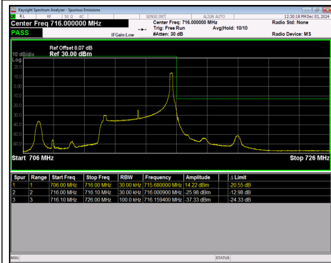
Band17-5MHz-64QAM-23755-1RB#0
