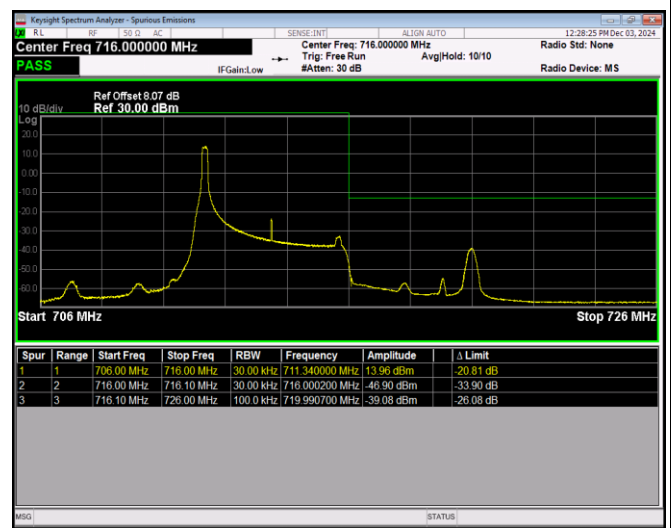
Band17-5MHz-16QAM-23825-25RB#0
