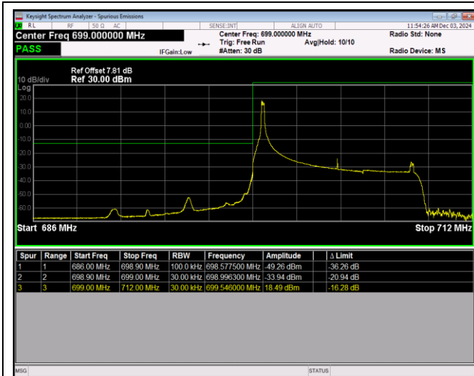
Band12-10MHz-QPSK-23060-50RB#0
