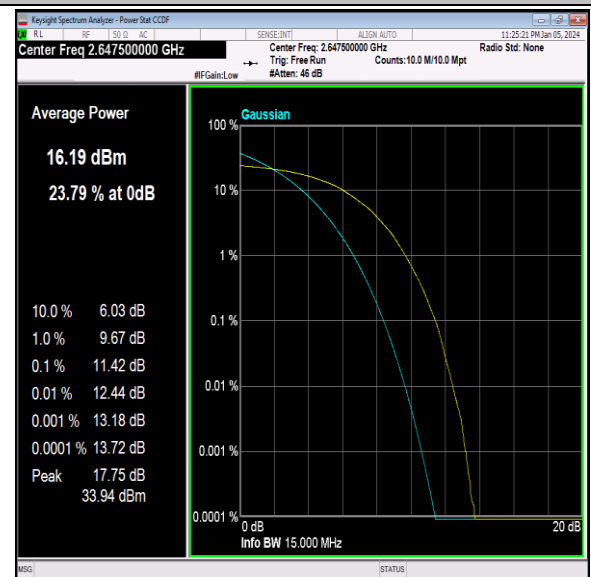
41(2535-2655)-15MHz-64QAM-41165-75RB#0-PASS
