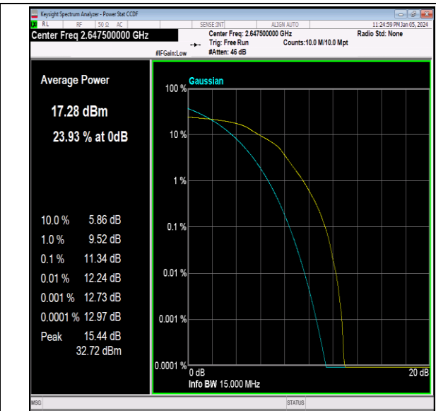
41(2535-2655)-15MHz-16QAM-41165-75RB#0-PASS
