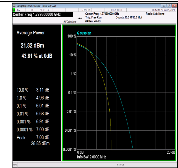
Band66-1.4MHz-16QAM-132665-6RB#0-PASS
