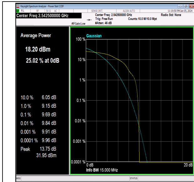
41(2535-2655)-15MHz-16QAM-40115-1RB#0-PASS
