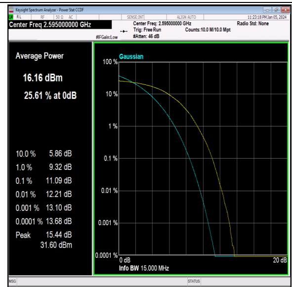
41(2535-2655)-15MHz-64QAM-40640-75RB#0-PASS
