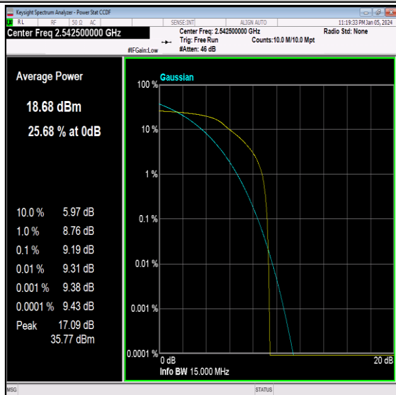
41(2535-2655)-15MHz-QPSK-40115-1RB#0-PASS
