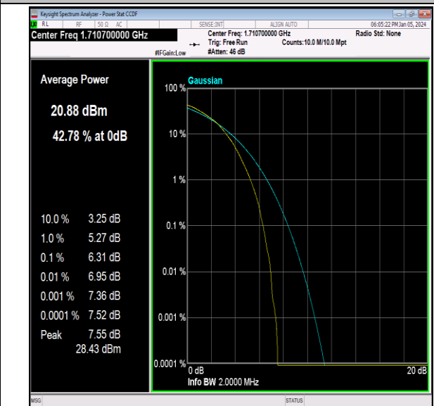
Band66-1.4MHz-64QAM-131979-6RB#0-PASS
