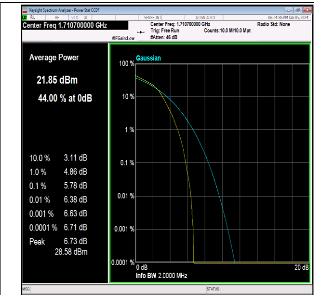
Band66-1.4MHz-16QAM-131979-6RB#0-PASS
