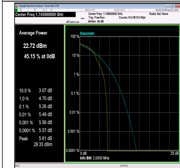
Band66-1.4MHz-16QAM-132322-1RB#0-PASS
