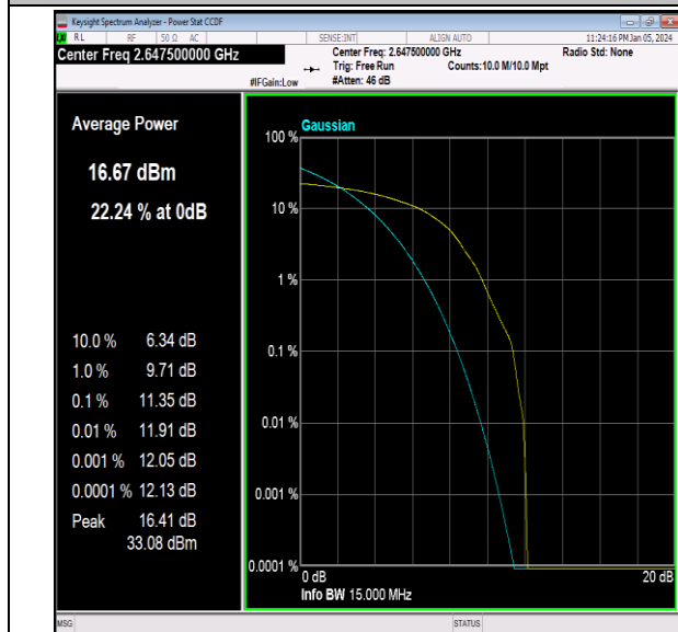
41(2535-2655)-15MHz-64QAM-41165-1RB#0-PASS
