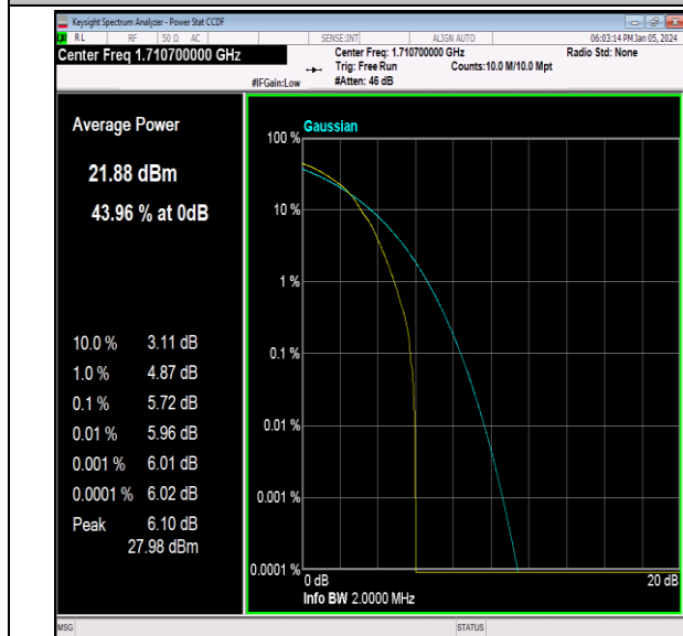
Band66-1.4MHz-64QAM-131979-1RB#0-PASS
