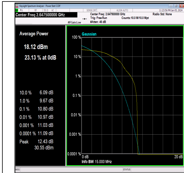
41(2535-2655)-15MHz-16QAM-41165-1RB#0-PASS
