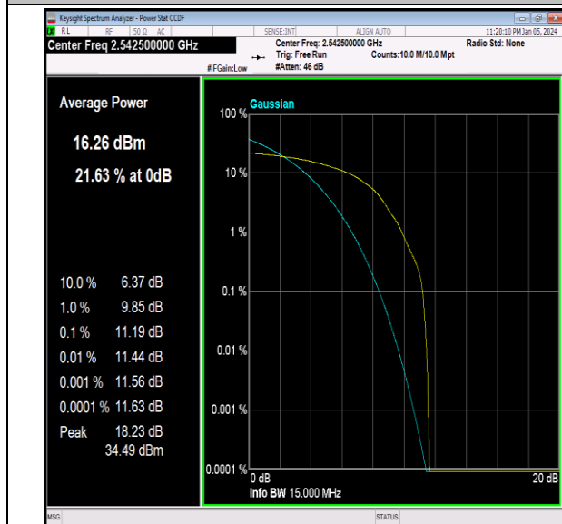
41(2535-2655)-15MHz-64QAM-40115-1RB#0-PASS
