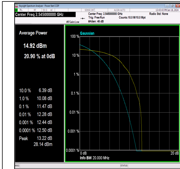
41(2535-2655)-20MHz-64QAM-40140-1RB#0-PASS
