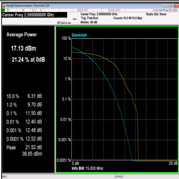
41(2535-2655)-15MHz-16QAM-40640-1RB#0-PASS
