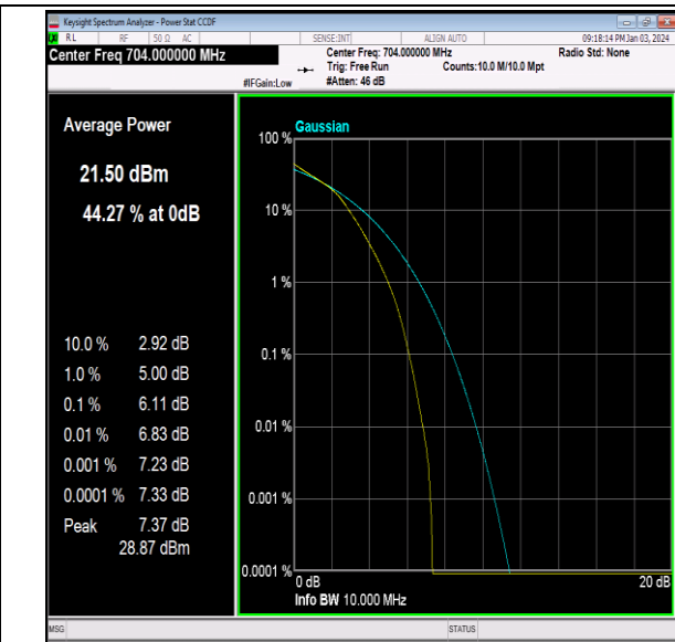
Band12-10MHz-16QAM-23060-50RB#0-PASS
