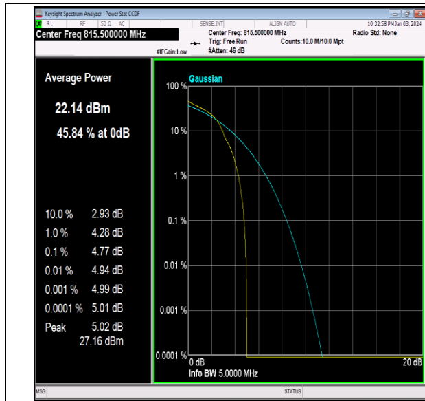
26(814-824)-3MHz-16QAM-26705-1RB#0-PASS
