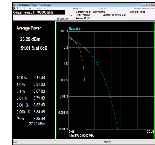
26(814-824)-1.4MHz-64QAM-26697-1RB#0-PASS
