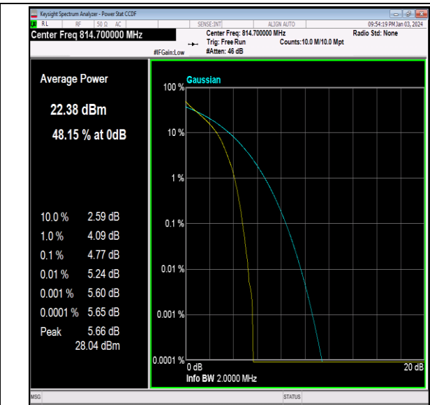
26(814-824)-1.4MHz-QPSK-26697-6RB#0-PASS
