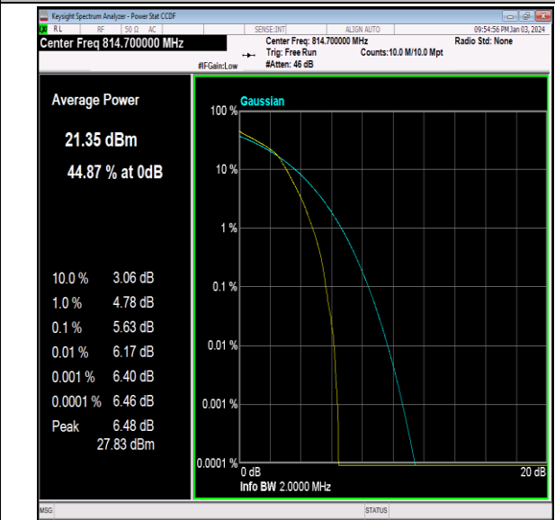
26(814-824)-1.4MHz-16QAM-26697-6RB#0-PASS
