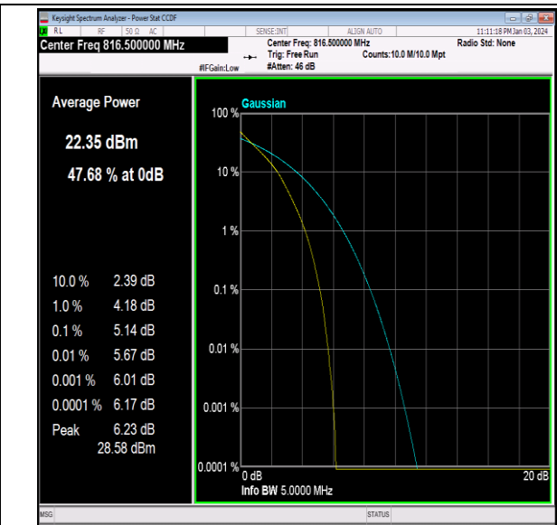
26(814-824)-5MHz-64QAM-26715-25RB#0-PASS
