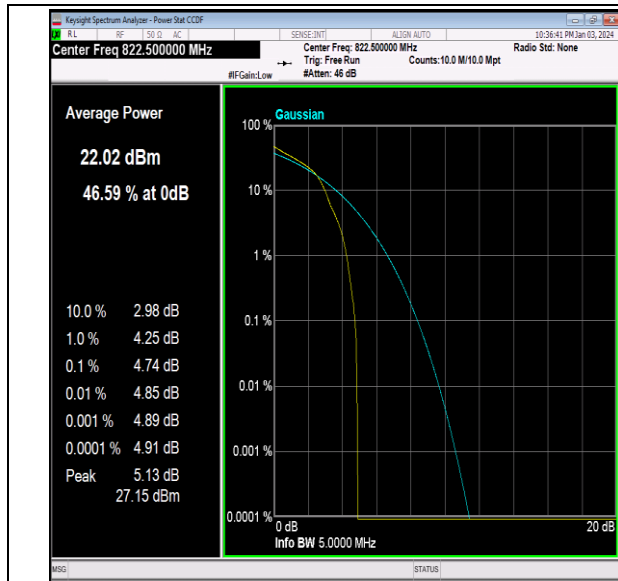
26(814-824)-3MHz-16QAM-26775-1RB#0-PASS
