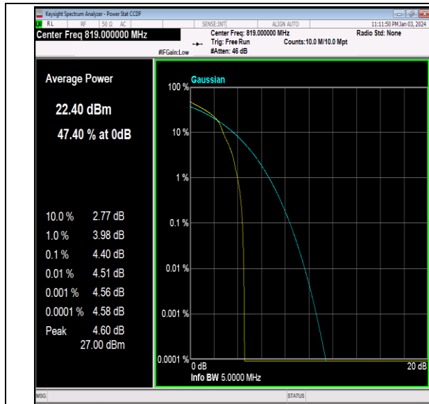
26(814-824)-5MHz-16QAM-26740-1RB#0-PASS
