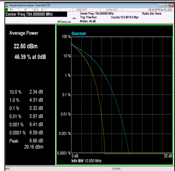
Band12-10MHz-64QAM-23060-50RB#0-PASS
