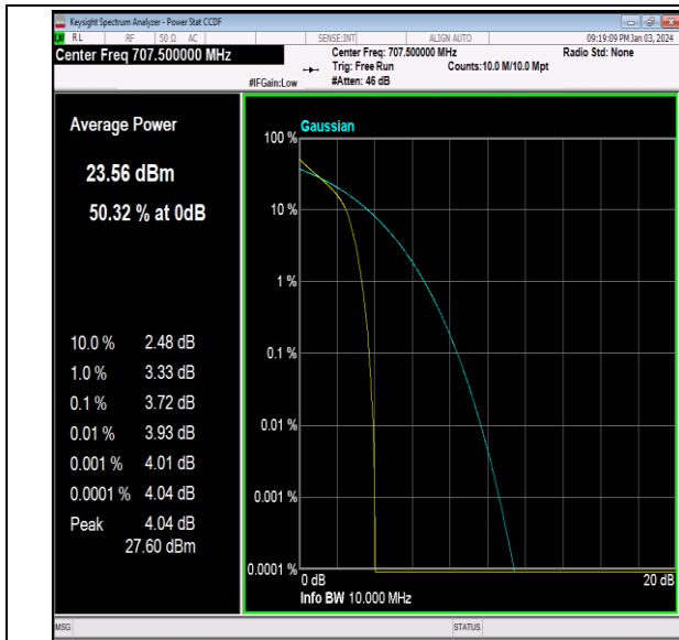
Band12-10MHz-64QAM-23095-1RB#0-PASS
