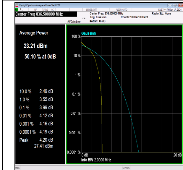
26(824-849)-1.4MHz-QPSK-26915-1RB#0-PASS
