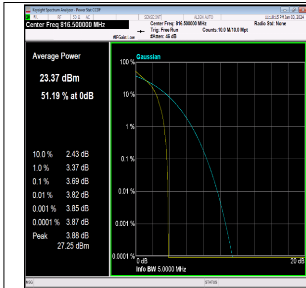
26(814-824)-5MHz-64QAM-26715-1RB#0-PASS
