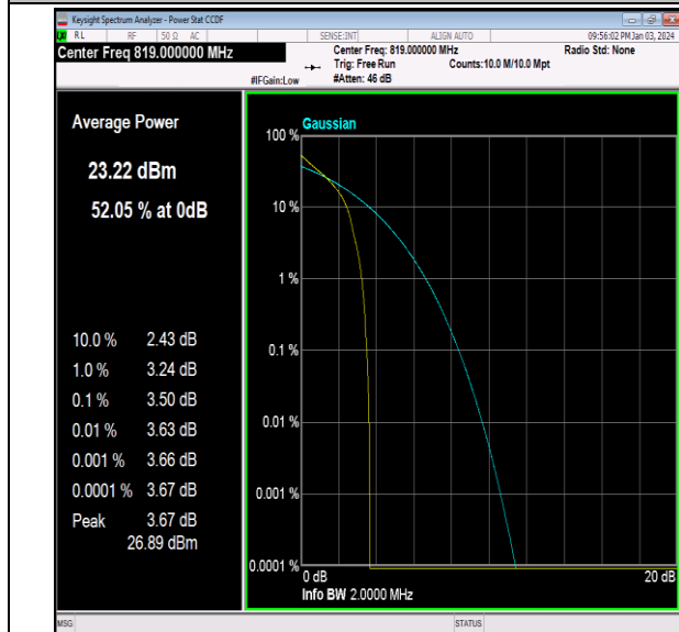
26(814-824)-1.4MHz-QPSK-26740-1RB#0-PASS
