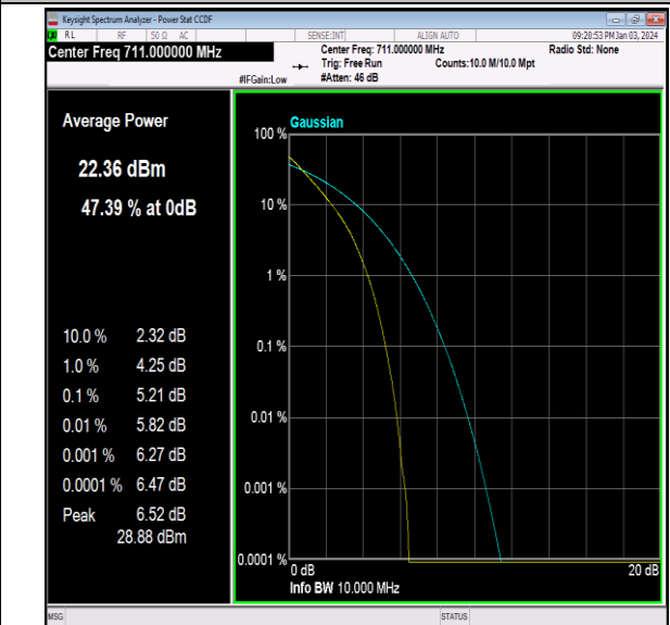
Band12-10MHz-QPSK-23130-50RB#0-PASS
