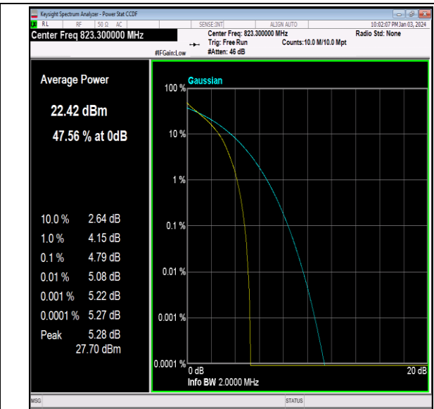
26(814-824)-1.4MHz-64QAM-26783-6RB#0-PASS
