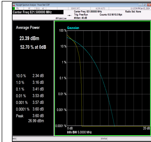
26(814-824)-5MHz-64QAM-26765-1RB#0-PASS
