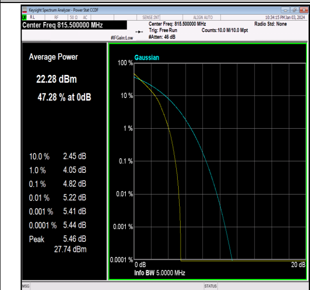
26(814-824)-3MHz-64QAM-26705-15RB#0-PASS
