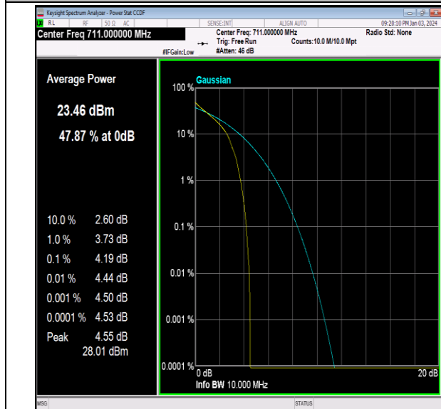
Band12-10MHz-QPSK-23130-1RB#0-PASS
