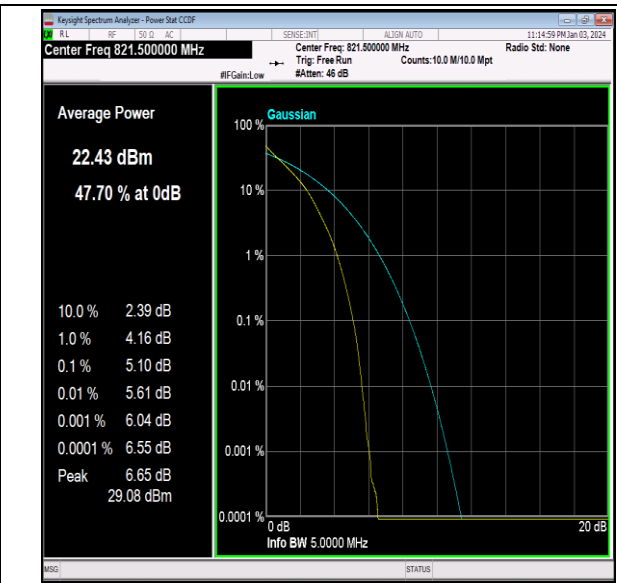
26(814-824)-5MHz-64QAM-26765-25RB#0-PASS
