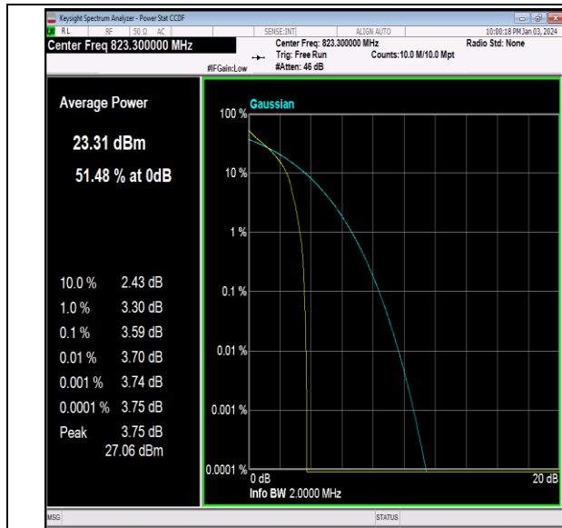
26(814-824)-1.4MHz-64QAM-26783-1RB#0-PASS
