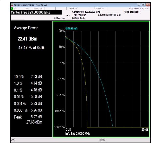
26(814-824)-1.4MHz-QPSK-26783-6RB#0-PASS
