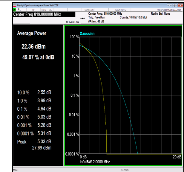
26(814-824)-1.4MHz-QPSK-26740-6RB#0-PASS
