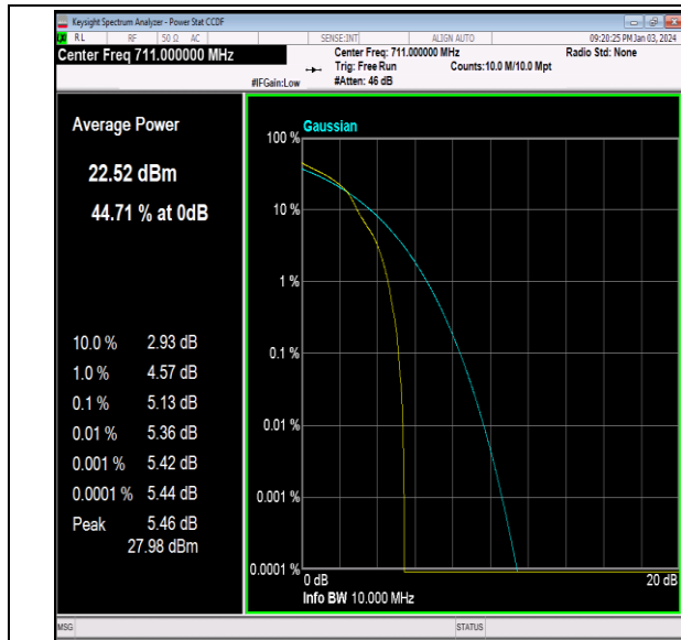
Band12-10MHz-16QAM-23130-1RB#0-PASS
