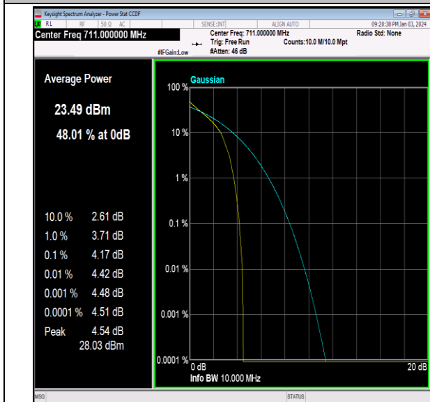
Band12-10MHz-64QAM-23130-1RB#0-PASS
