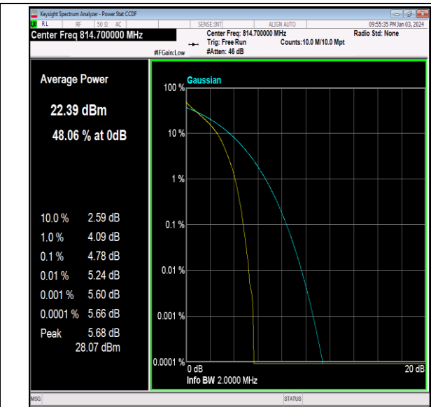
26(814-824)-1.4MHz-64QAM-26697-6RB#0-PASS
