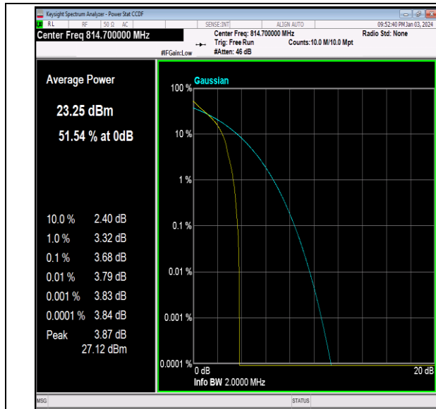
26(814-824)-1.4MHz-QPSK-26697-1RB#0-PASS
