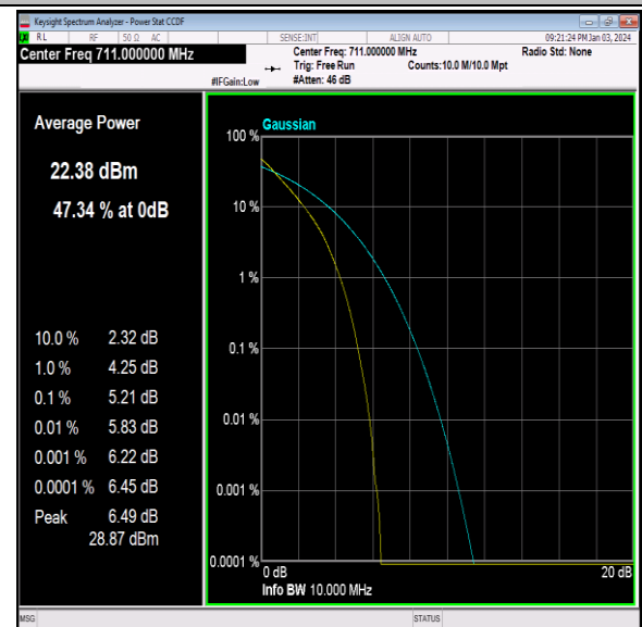
Band12-10MHz-64QAM-23130-50RB#0-PASS
