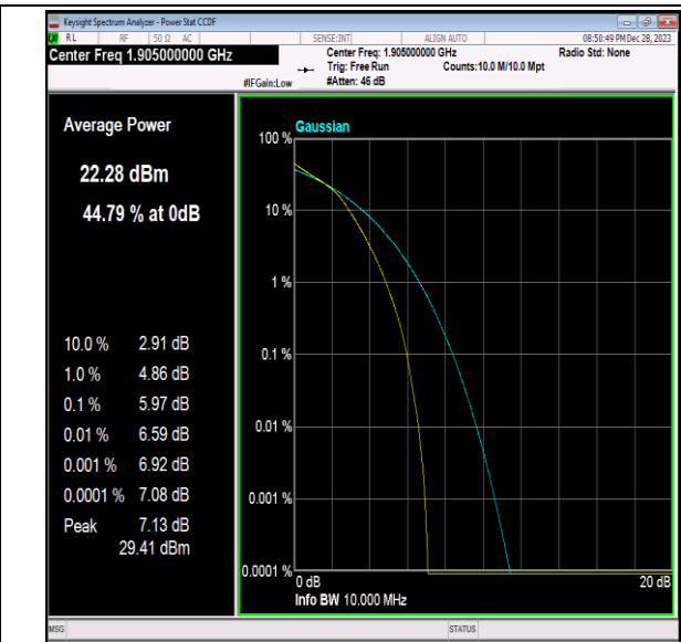
Band2-10MHz-16QAM-19150-50RB#0-PASS
