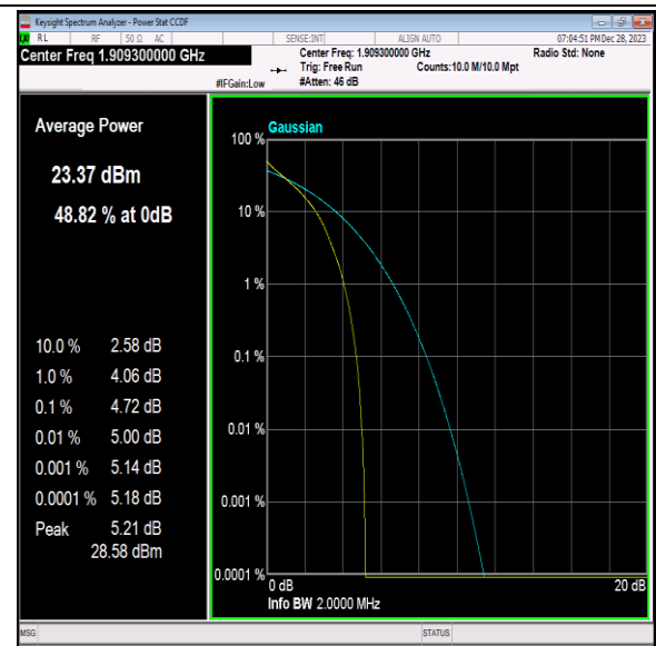
Band2-1.4MHz-QPSK-19193-6RB#0-PASS
