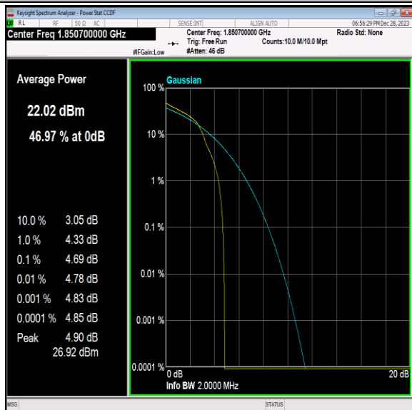
Band2-1.4MHz-16QAM-18607-1RB#0-PASS
