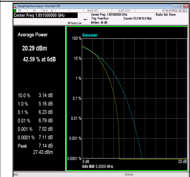
Band2-3MHz-64QAM-18615-15RB#0-PASS
