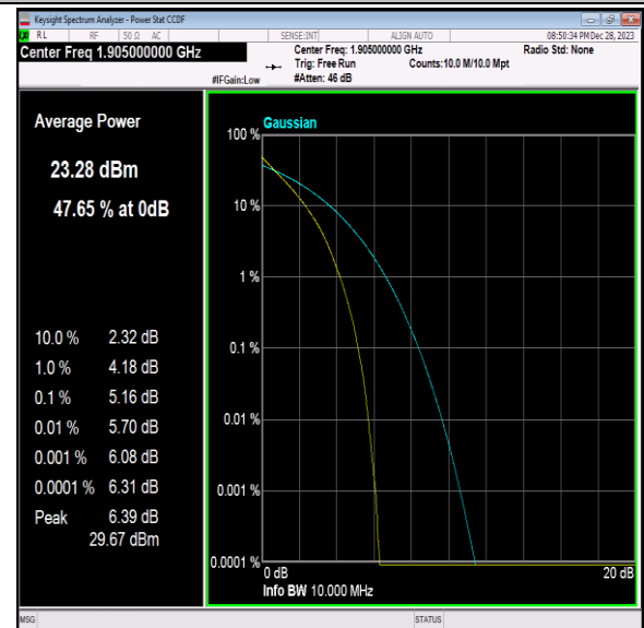
Band2-10MHz-QPSK-19150-50RB#0-PASS
