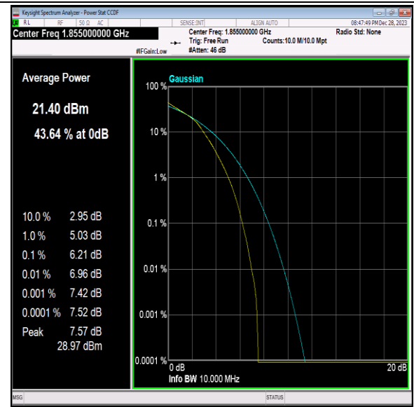
Band2-10MHz-16QAM-18650-50RB#0-PASS
