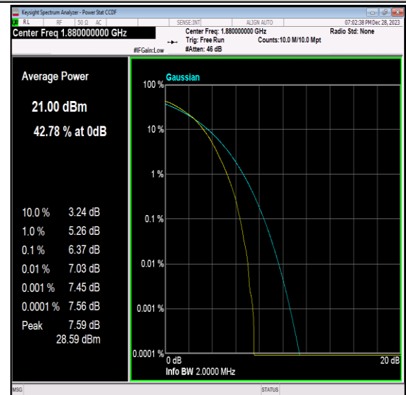
Band2-1.4MHz-64QAM-18900-6RB#0-PASS
