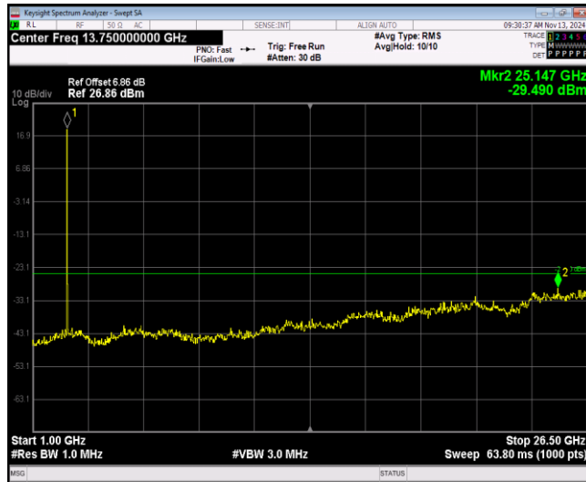
Band41-5MHz-16QAM-41215-1RB#0-Range2:1000~26500MHz
