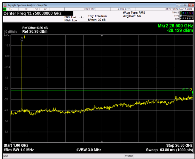
Band7-20MHz-16QAM-20850-1RB#0-Range2:1000~ 26500MHz
