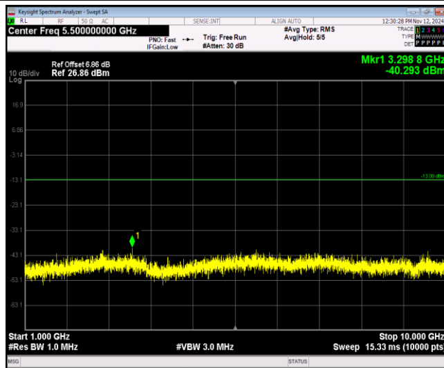
Band5-10MHz-64QAM-20450-1RB#0-Range2:1000~10000MHz
