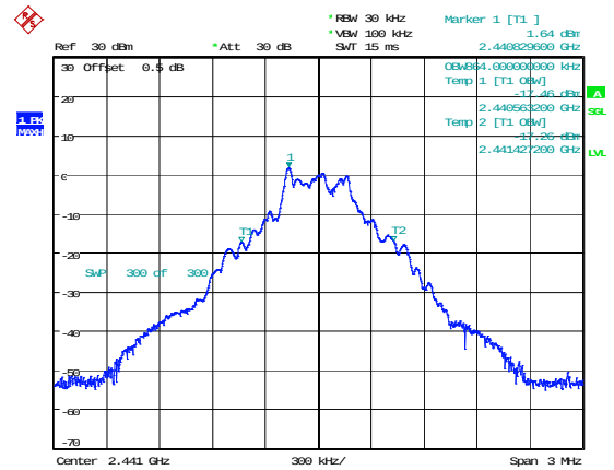
DH1_Middle 0.864MHz
