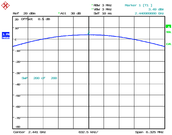
2DH1_Middle 3.49dBm
