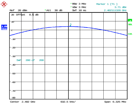
2DH1_Low 3.71dBm
