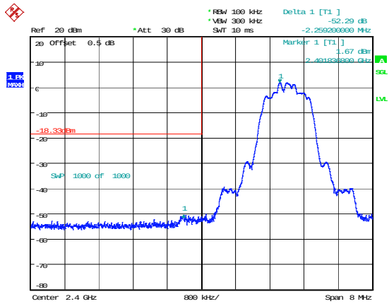
3DH1_Low 52.29dB
