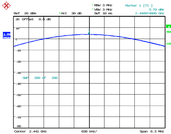
3DH1_Middle 3.79dBm
