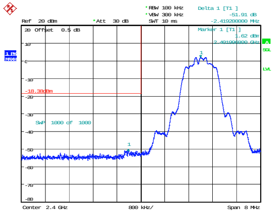
2DH1_Low 51.91dB
