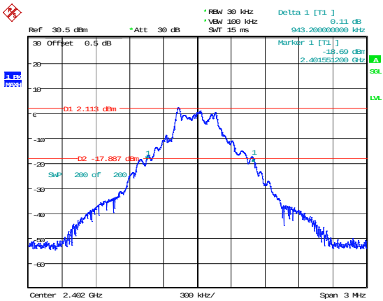
DH1_Low 0.943MHz
