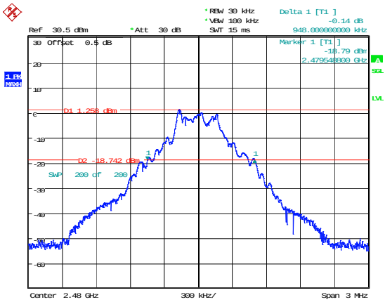
DH1_High 0.948MHz
