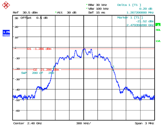
2DH1_High 1.267MHz
