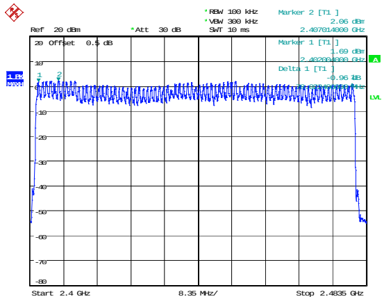
2DH1_Hopping 79
