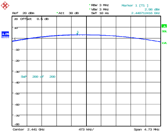
DH1_Middle 2.98dBm
