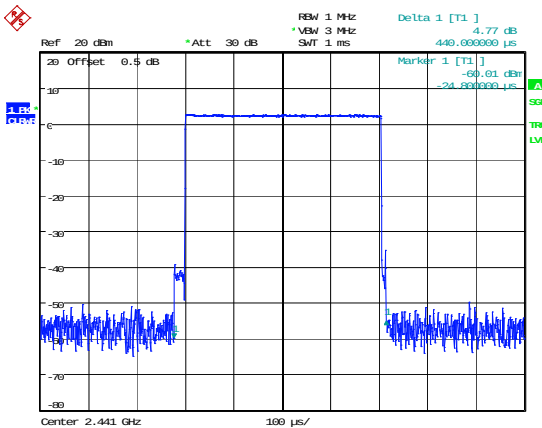
DH1_Hopping 0.440ms
