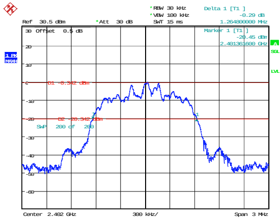
2DH1_Low 1.265MHz
