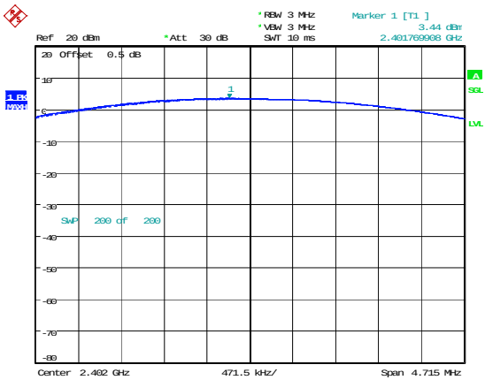
DH1_Low 3.44dBm
