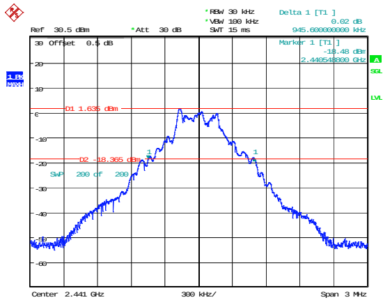
DH1_Middle 0.946MHz
