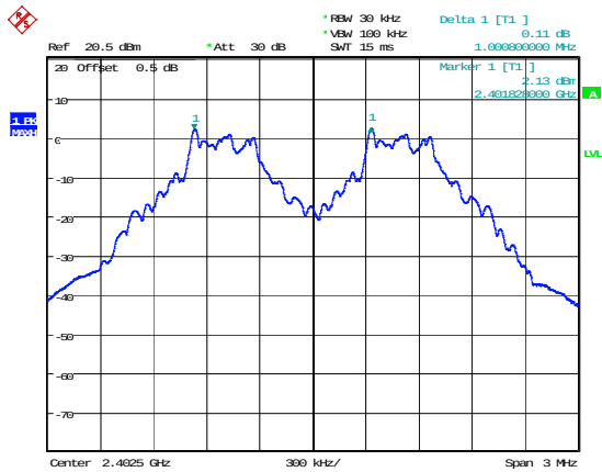
DH1_Low 1.001MHz
