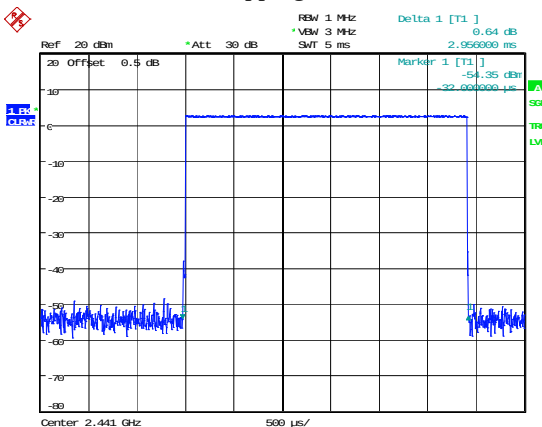
DH5_Hopping 2.956ms
