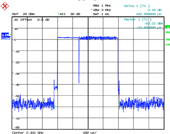
2DH1_Hopping 0.433ms
