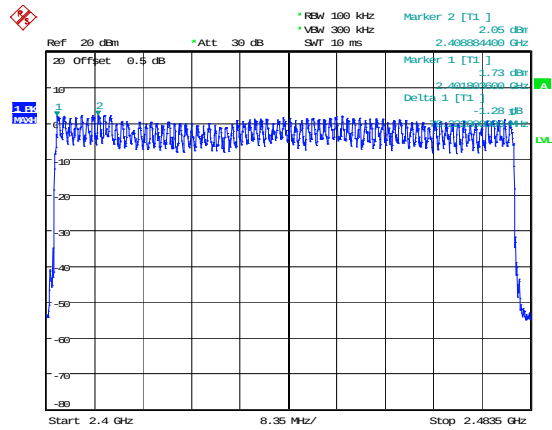
3DH1_Hopping 79
