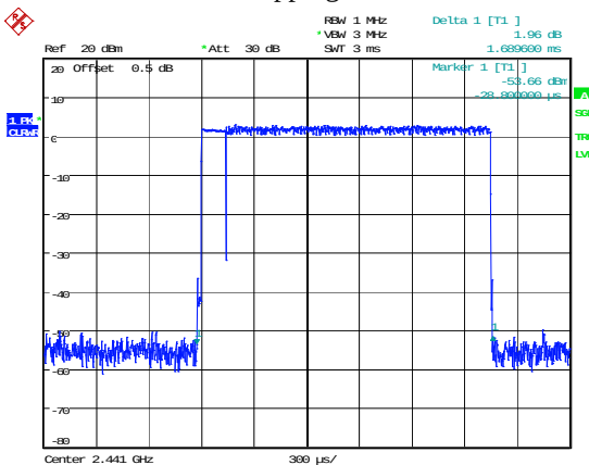
2DH3_Hopping 1.690ms
