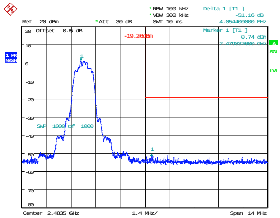
3DH1_High 51.16dB
