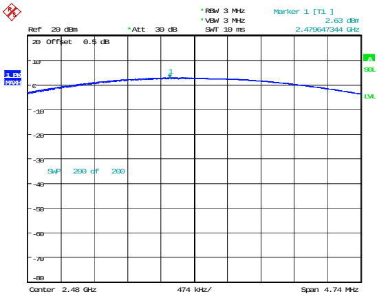
DH1_High 2.63dBm
