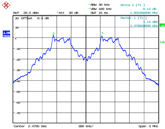
DH1_High 1.003MHz
