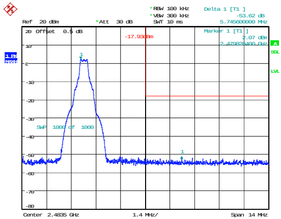
DH1_High 53.62dB
