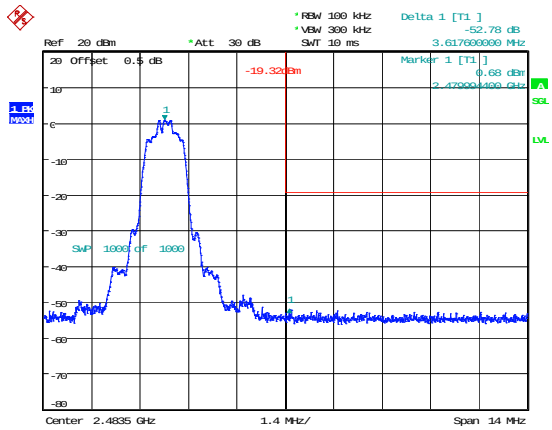
2DH1_High 52.78dB
