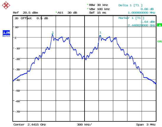
DH1_Middle 1.001MHz
