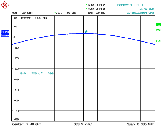
2DH1_High 2.76dBm
