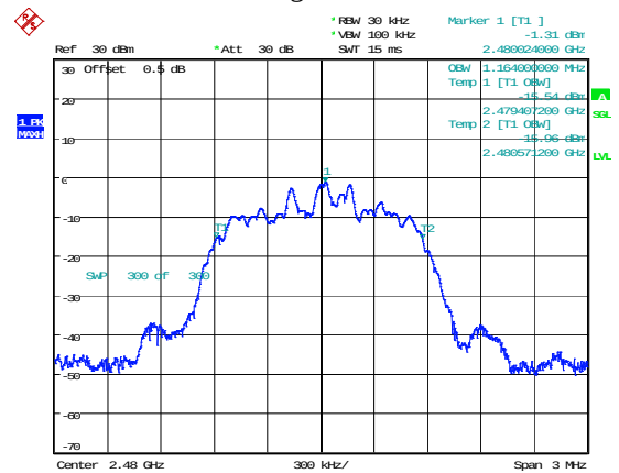
2DH1_High 1.164MHz
