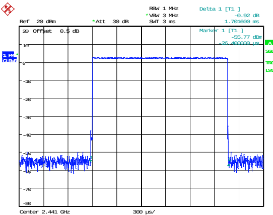
DH3_Hopping 1.702ms
