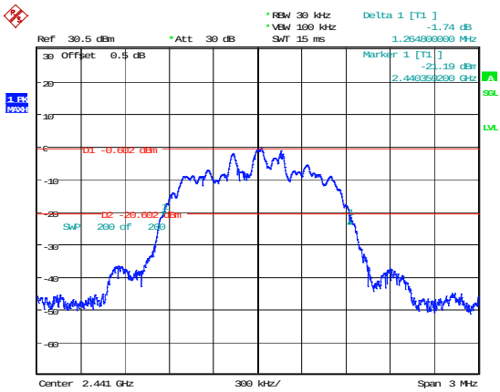
2DH1_Middle 1.265MHz
