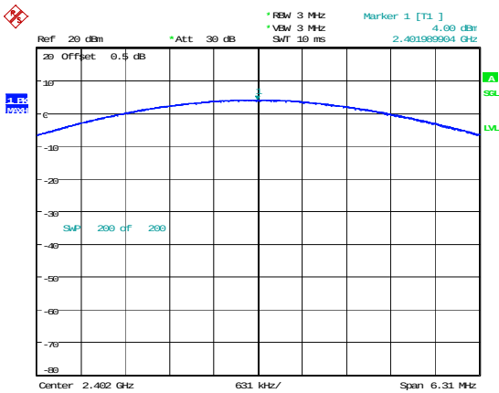
3DH1_Low 4.00dBm
