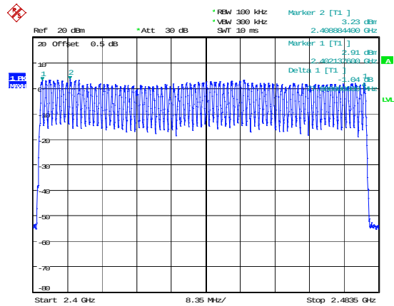
DH1_Hopping 79
