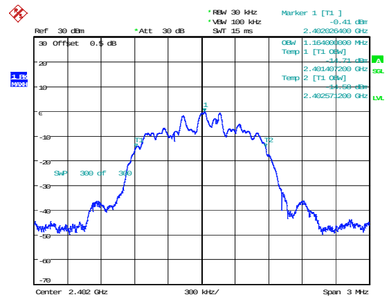
2DH1_Low 1.164MHz
