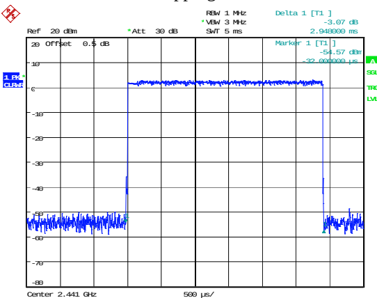
2DH5_Hopping 2.948ms
