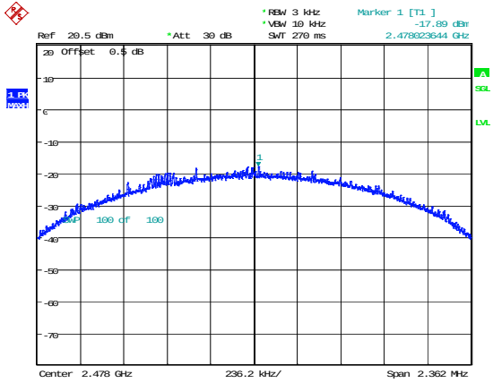
BLE_2M_High_Channel
