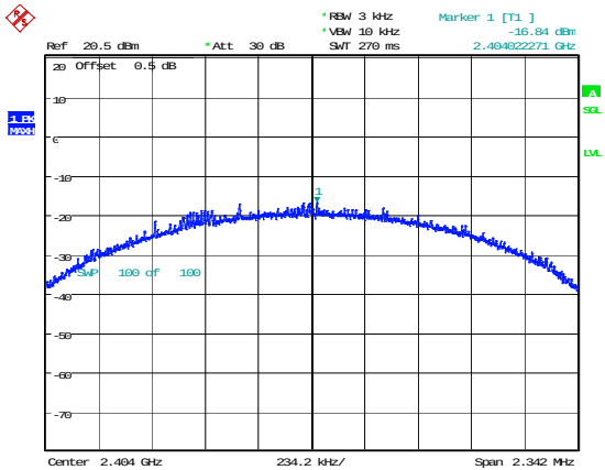
BLE_2M_Low_Channel
