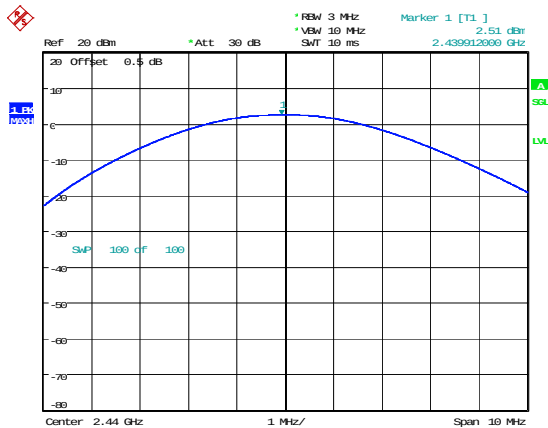
BLE_1M_Middle_Channel
