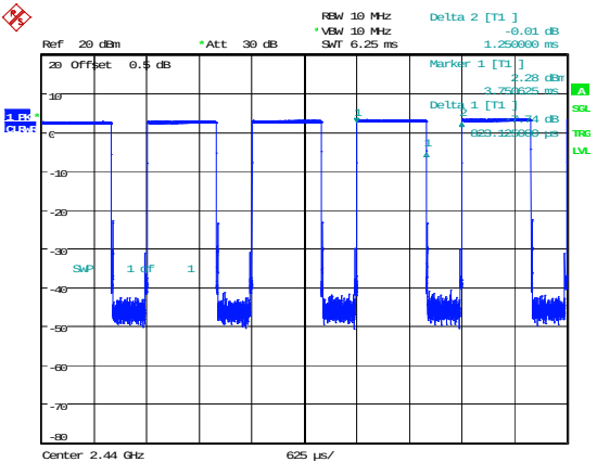
BLE_2M_Middle_Channel
