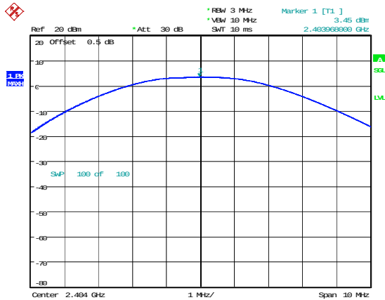
BLE_2M_Low_Channel
