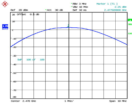
BLE_2M_High_Channel
