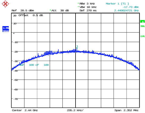
BLE_2M_Middle_Channel
