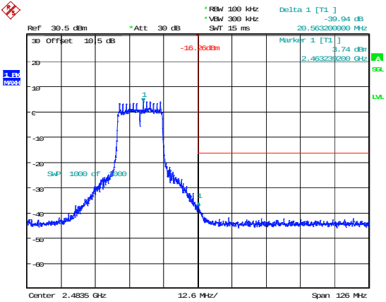
802.11g_2462MHz
