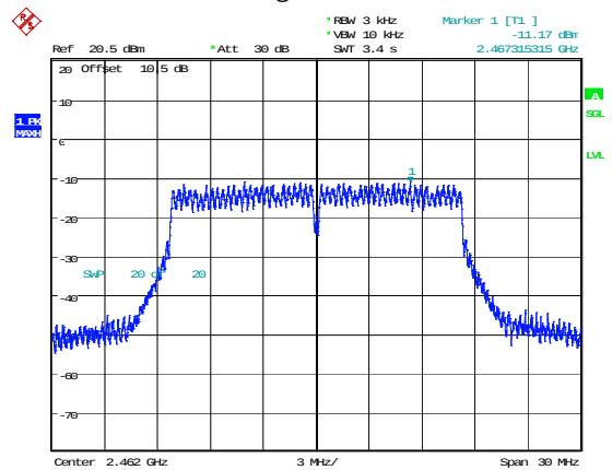
802.11g_2462MHz
