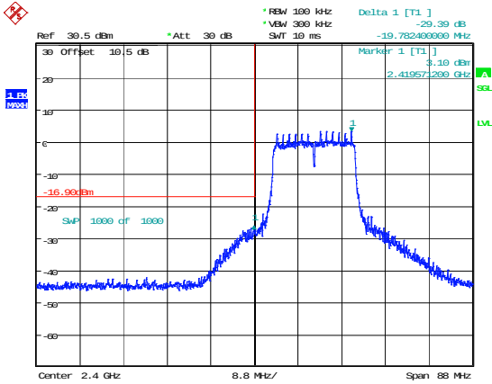
802.11g_2412MHz
