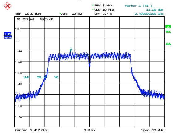
802.11g_2412MHz
