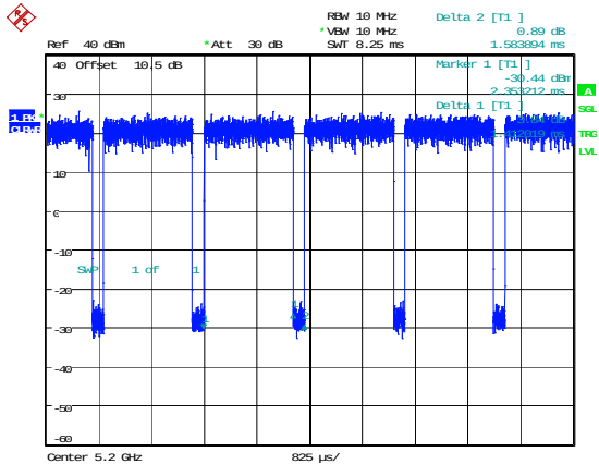
802.11a_5200MHz
