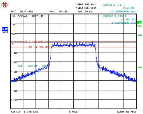
802.11n20_5745MHz
