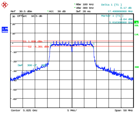
802.11n20_5825MHz
