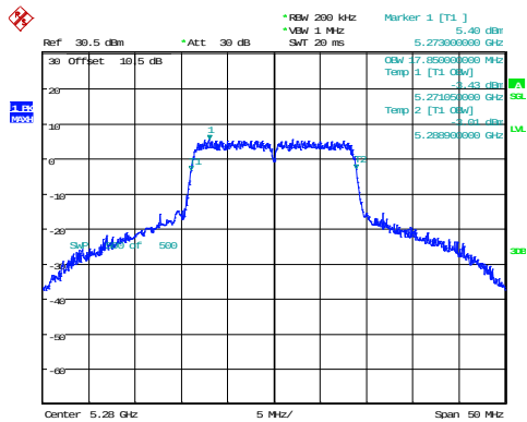
802.11n20_5280MHz
