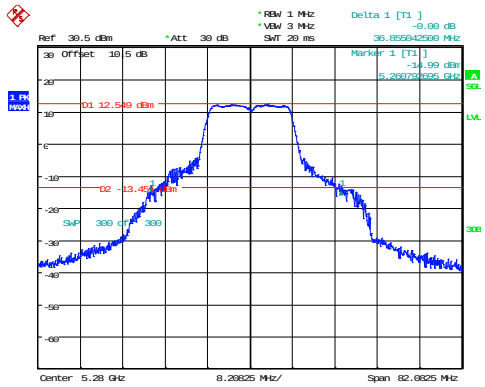
802.11a_5280MHz
