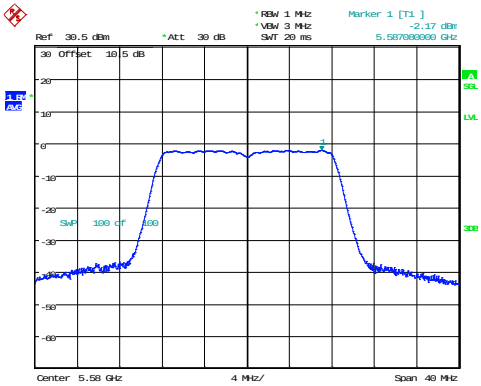
802.11a_5580MHz
