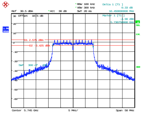
802.11a_5745MHz
