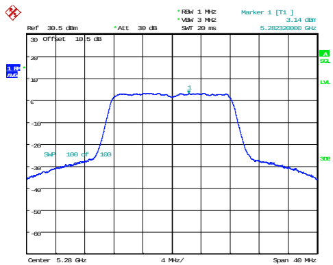
802.11a_5280MHz
