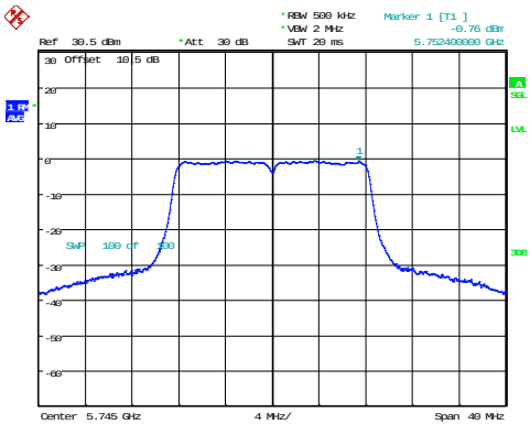
802.11a_5745MHz
