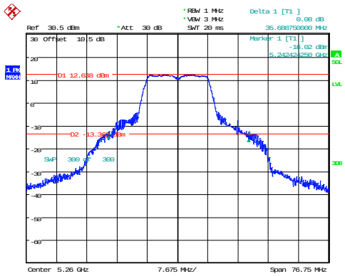
802.11a_5260MHz
