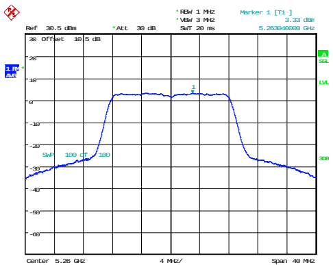
802.11a_5260MHz
