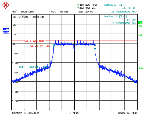
802.11a_5825MHz
