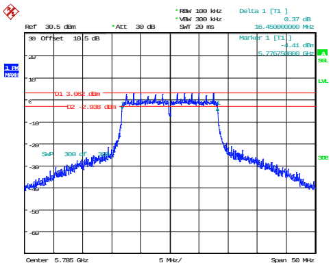
802.11a_5785MHz
