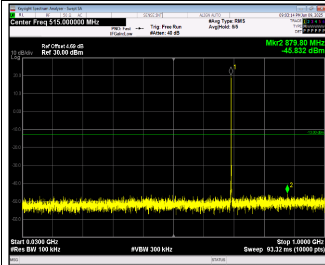
Band12-1.4MHz-64QAM-23095-1RB#0-Range1:30~1000MHz
