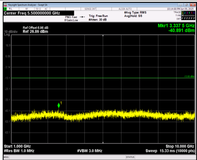
Band17-5MHz-64QAM-23755-1RB#0-Range2:1000~10000MHz
