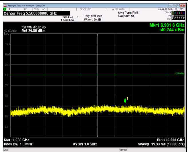
Band12-10MHz-64QAM-23060-1RB#0-Range2:1000 ~10000MHz
