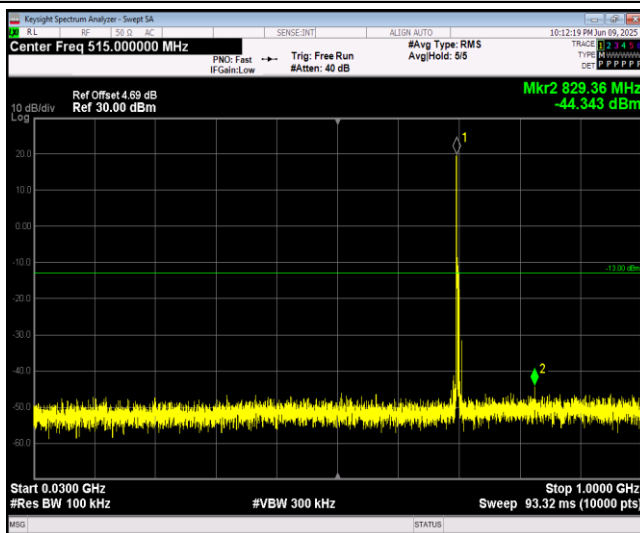
Band17-5MHz-64QAM-23790-1RB#0-Range1:30~1000MHz
