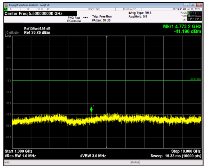
Band26-1.4MHz-16QAM-26783-1RB#0-Range2:1000 ~10000MHz
