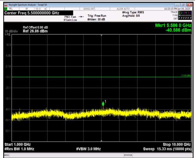
Band17-10MHz-QPSK-23800-1RB#0-Range2:1000~10000MHz
