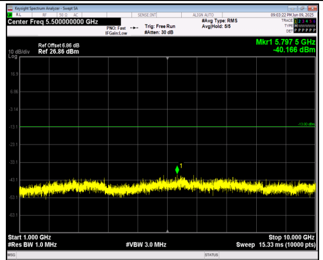
Band12-1.4MHz-64QAM-23095-1RB#0-Range2:1000~10000MHz
