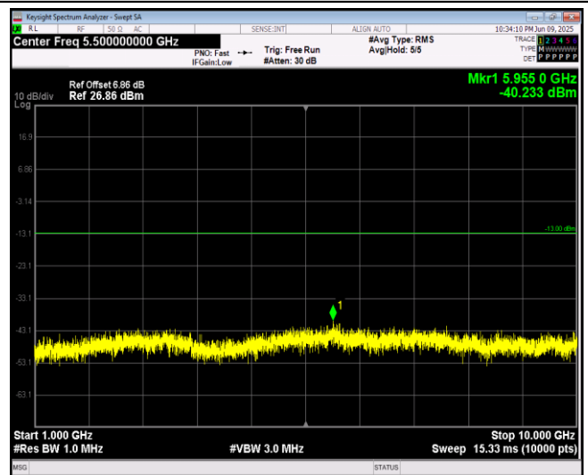
Band17-10MHz-16QAM-23780-1RB#0-Range2:1000~10000MHz
