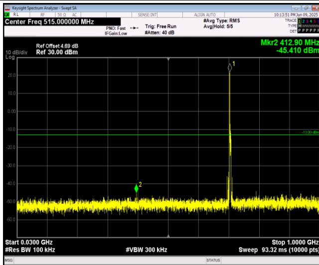
Band17-5MHz-64QAM-23755-1RB#0-Range1:30~1000MHz
