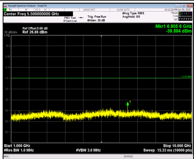
Band17-5MHz-64QAM-23790-1RB#0-Range2:1000~10000MHz
