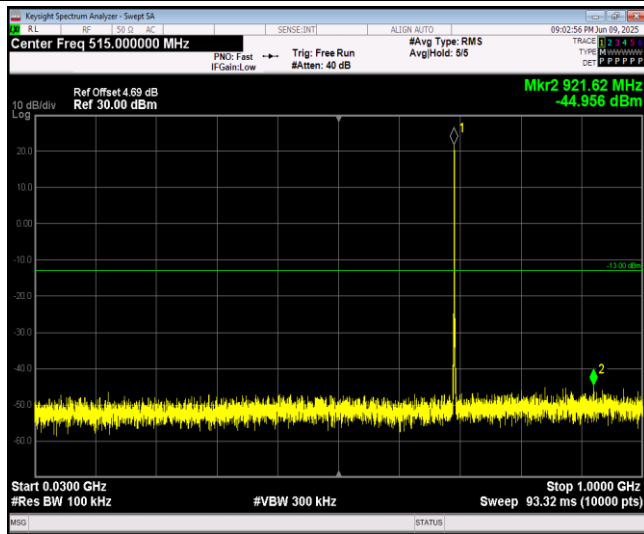
Band12-1.4MHz-16QAM-23095-1RB#0-Range1:30~1 000MHz
