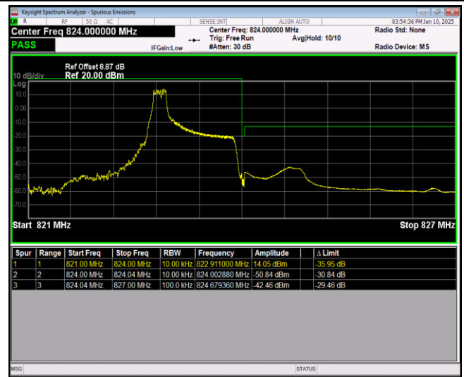
Band26-1.4MHz-QPSK-26783-6RB#0
