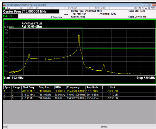
Band17-10MHz-64QAM-23780-1RB#0
