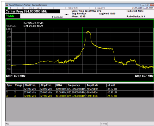
Band26-1.4MHz-QPSK-26797-6RB#0
