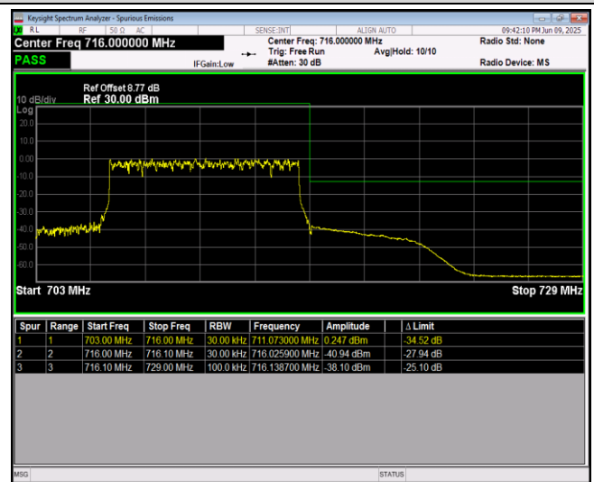
Band17-5MHz-QPSK-23755-1RB#24
