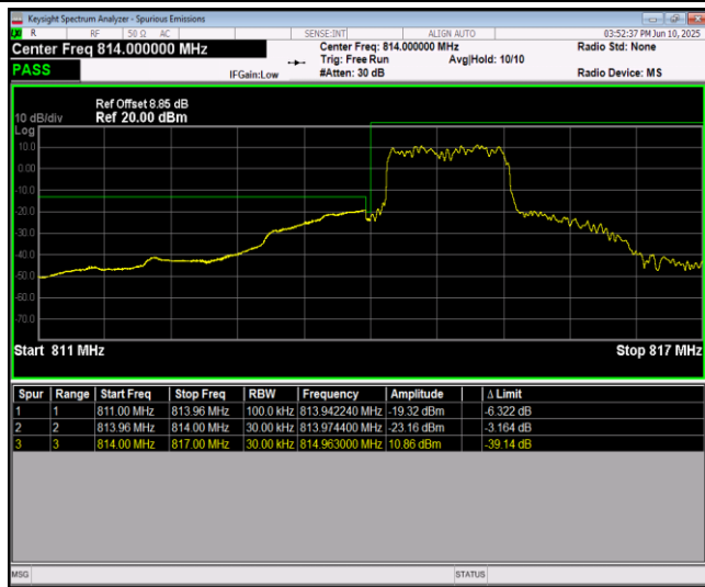
Band26-1.4MHz-QPSK-26783-1RB#5
