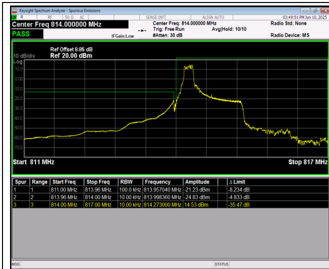
Band26-1.4MHz-QPSK-26697-6RB#0
