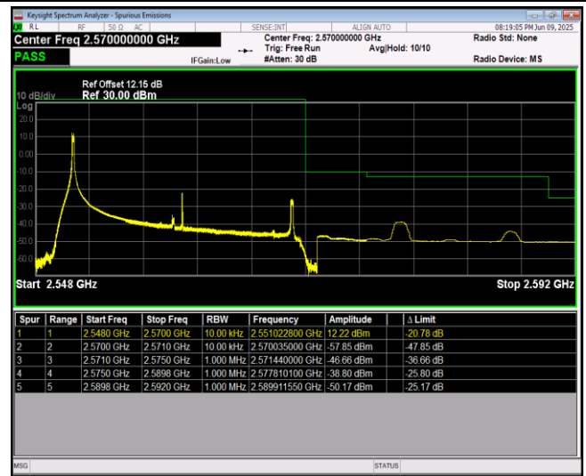
Band7-20MHz-64QAM-21350-100RB#0
