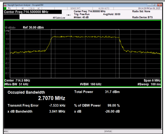
Band12-3MHz-16QAM-23095-15RB#0
